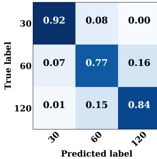
Fig. 7.14 Cascaded RF model prediction performance on test set as confusion matrices.
