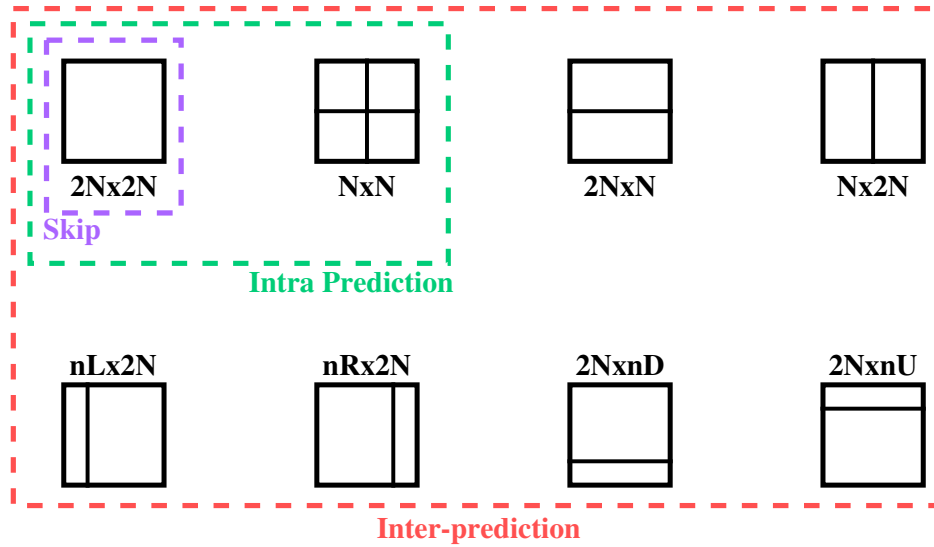
Fig. 2.9 HEVC Prediction Unit (PU) modes.
