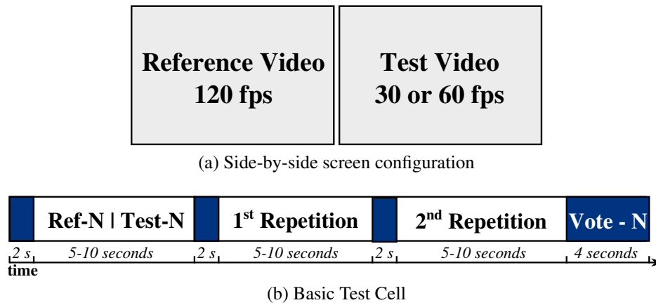
Fig. 7.4 Ground truth generation SDSCE evaluation method.
