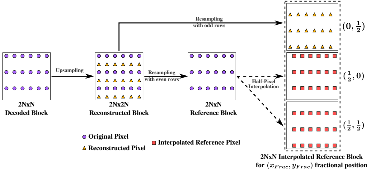
Fig. 6.11 Example fractional pixel interpolation for ASR-based inter-prediction with 2N \times N as chosen resolution.
