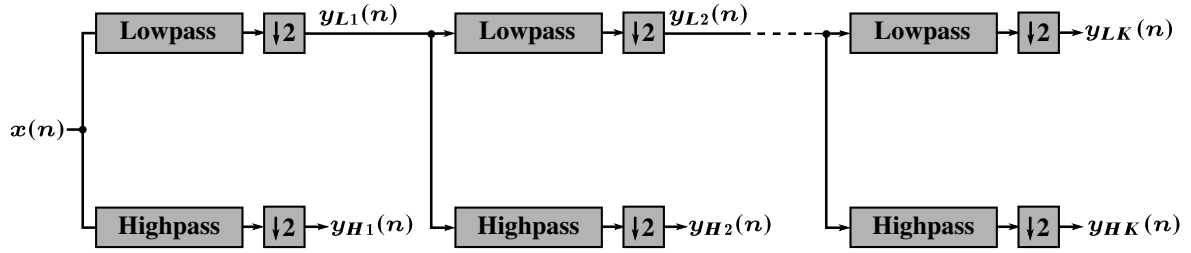
Fig. 4.2 Analysis stage of a K-level 1-D wavelet decomposition. \mathbf{y}_{f_k} represents the wavelet coefficients for frequency sub-band f , f \in \{L, H\} , at the k^{th} level of decomposition.
