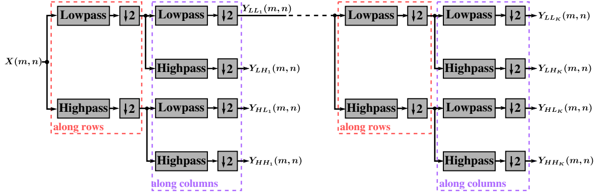
Fig. 4.3 Analysis stage of a K -level 2-D wavelet decomposition. y_{fk} represents the wavelet coefficients for frequency sub-band f , f \in \{LL, LH, HL, HH\} , at the k^{th} level of decomposition.
