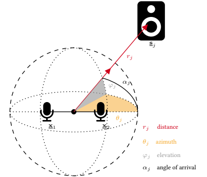
FIGURE 8.3: Geometrical illustration of the Sound Source Localization, showing the azimuth \theta_j , the elevation \varphi_j and angle of arrival \alpha_j for the source j at \mathbf{s}_j and two microphones at \mathbf{x}_1, \mathbf{x}_2 respectively.
