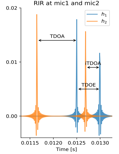
FIGURE 10.6: Superposition of two RIRs and visualization of time difference of arrival between direct paths ( TDOA ), first echoes ( iTDOA ) and direct path and first echo ( TDOE ).
