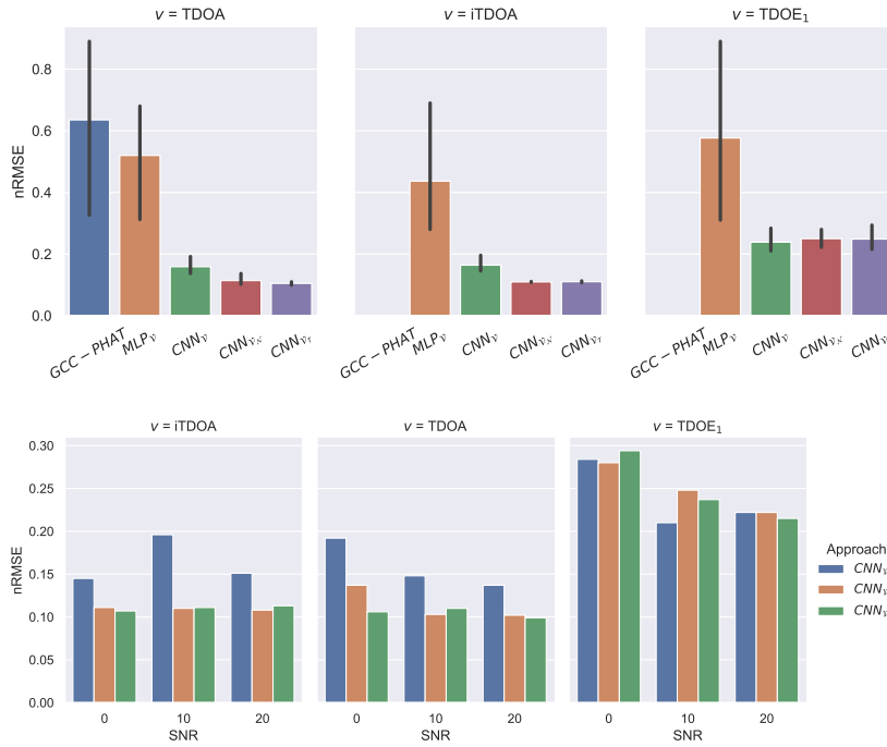
FIGURE 6.4: Normalize root mean squared error (the lower, the better) for TDOA estimation using the proposed architectures on white noise source signals.
