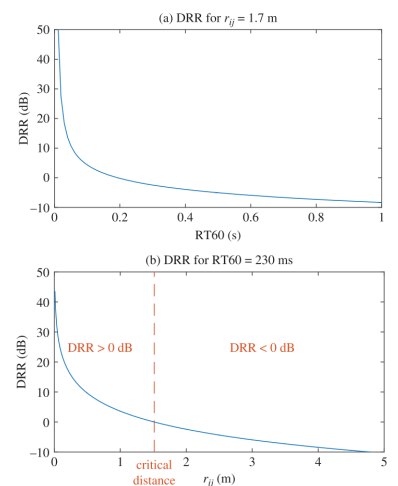
FIGURE 2.17: DRR as a function of the RT_{60} and the source distance r_{ij} based on Eyring's formula (Gustafsson et al., 2003). These curves assume that there is no obstacle between the source and the microphone, so that the direct path exists. The room dimensions are the same as in Figure 3.1.
