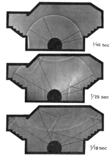
Schlieren photographs showing successive stages in the progress of a sound pulse in a section of a Debating Chamber. Image courtesy of [Davis and Fleming 1926]. Sabine used Schlieren photography to investigate sound propagation paths in the early 1900s. Their impressive visualizations show wavefronts that are augmented with rays that are perpendicular to the wavefronts
