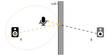
FIGURE 4.4: Illustration of the ellipsoid method: the length of the reflected path from the image source \hat{s} to the microphone at \mathbf{x} constrain the reflector line to be tangent to an ellipse.
