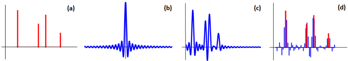
FIGURE 3.6: (a) Continuous-time stream of Diracs \tilde{h}(t) , (b) sinc kernel \tilde{\phi}_{LP}(t) , (c) smoothed stream of Diracs, (d) original stream of Dirac \tilde{h}(t) (red) and its sampled (i. e., smoothed and discrete) version (blue). Image courtesy of [Tukuljac et al. 2018]
