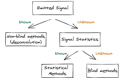
FIGURE 4.6: Classification of the State of the Art in channel estimation.
