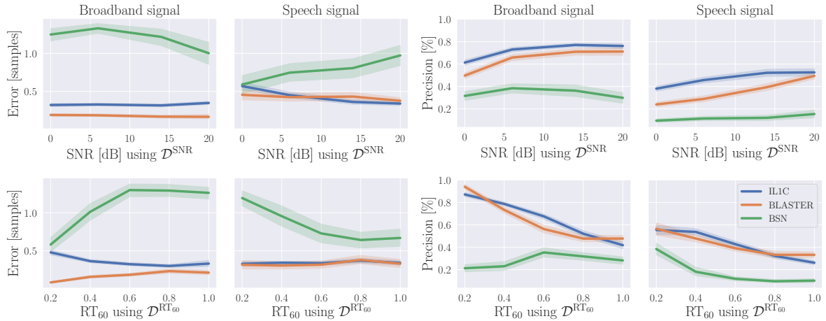
FIGURE 5.4: Mean error (left) and precision (right) versus SNR level (top) and RT_{60} level (bottom) using broadband and speech signals for the task of recovering R = 7 echoes. A threshold of \tau_{\max} = 2 samples is used to compute the precision. Error bands denotes 95% confidence intervals.
