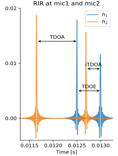
FIGURE 6.2: Superposition of two synthetic RIRs and visualization of time differences of arrival between direct paths ( TDOA ), first echoes ( iTDOA ) and direct path and first echo ( TDOE ).
