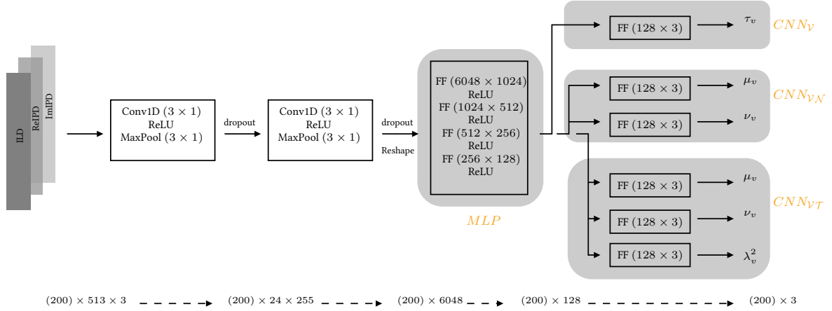
FIGURE 6.3: Architecture of the proposed deep neural network. Input dimensions for each stage are reported. The first dimension is the batch size |\Xi| = 200
