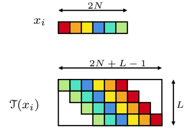
FIGURE 5.1: Graphical representation of the construction of \mathcal{T}(x_i) from x_i
