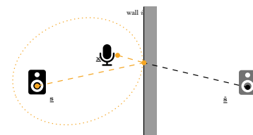
FIGURE 4.4: Illustration of the ellipsoid method: the length of the reflected path from the image source \hat{s} to the microphone at \underline{x} constrain the reflector line to be tangent to an ellipse.
