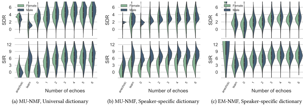
FIGURE 9.7: Distribution of SDR and SIR for male and female speakers as a function of the number of echoes included in modeling, and comparison with the three baselines.
