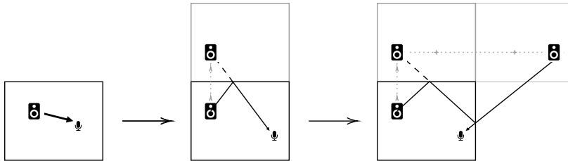
FIGURE 2.16: From left to right, path involving the direct path, one reflection obtained using first-order image, and two reflections obtained using two images. Image inspired from [Habets 2006].
