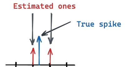
FIGURE 5.2: Schematics of the bodyguard effect affecting on-grid approaches. This is true only if h is non-negative.
