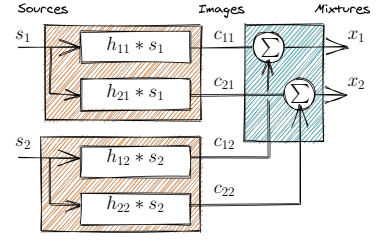
FIGURE 3.3: Graphical representation of the mixing model 3.5 for 2 sources and 2 microphones. The text is overlapping on purpose.
