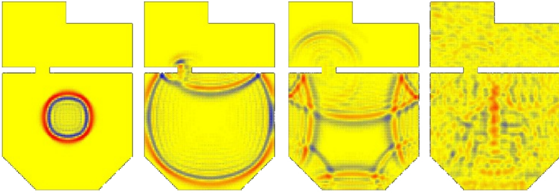
FIGURE 2.11: Simulation of Sound propagation at four consecutive timestamps using the DWM technique. A short, sharp, impulsive sound fired into the larger of two rooms causes a circular wavefront to spread out from the sound source. The wave is reflected from the walls and part of it passes through a gap into the smaller room. In the larger room, interference effects are clearly visible; in the smaller room, the sound wave has spread out into an arc, demonstrating the effects of diffraction. A short while after the initial event, the sound energy has spread out in a much more random and complex fashion. Image taken from University of York's AudioLab website.
