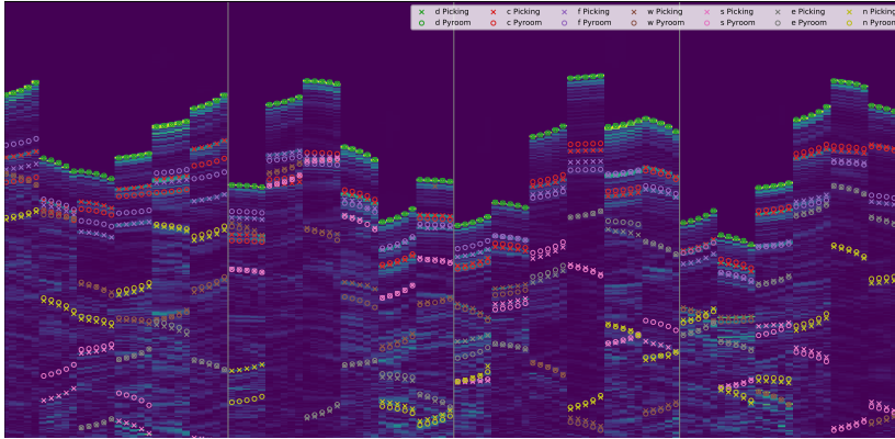
FIGURE 7.6: RIR Skyline annotated with observed peaks ( \times ) together with their geometrically-expected position ( \circ ) computed with the Pyroomacoustic simulator. As specified in the legend, different colors are used to indicate the room facets responsible for the reflection: direct path (d), ceiling (c), floor (f), west wall (w), . . . , north wall (n).
