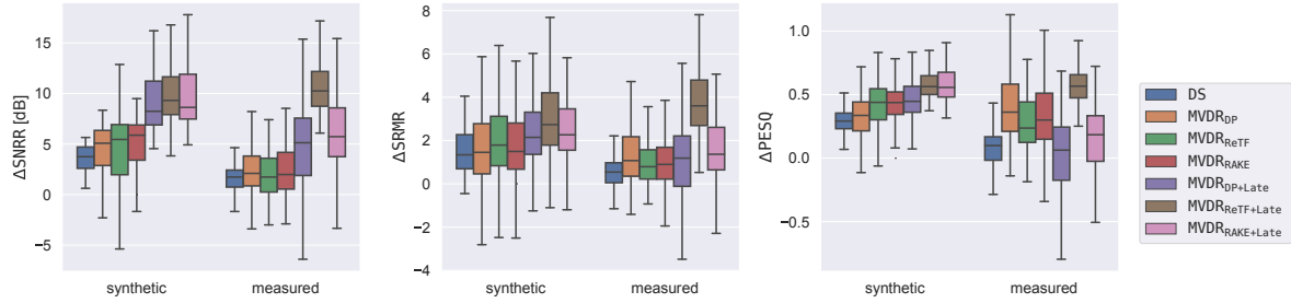
FIGURE 11.1: Comparison of echo-aware beamforming for the room configuration 011111 ( RT_{60} \approx 600 ms) on measured and synthetic data for all combinations of source-array positions in the dEchorate dataset.
