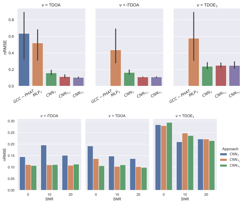
FIGURE 6.4: Normalize root mean squared error (the lower, the better) for TDOA estimation using the proposed architectures on white noise source signals.
