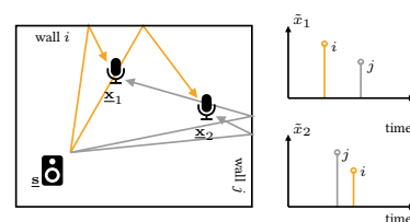
FIGURE 4.3: Illustration of different orders of arrival of wall reflections
