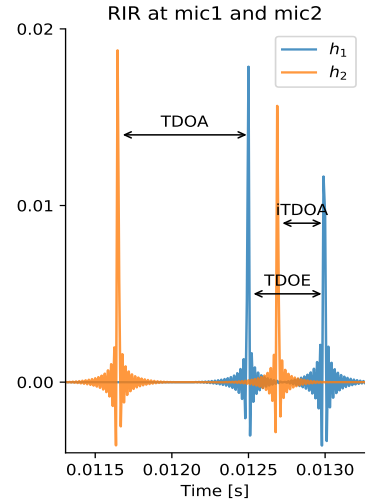
FIGURE 10.6: Superposition of two RIRs and visualization of time difference of arrival between direct paths (TDOA), first echoes (iTDOA) and direct path and first echo (TDOE).
