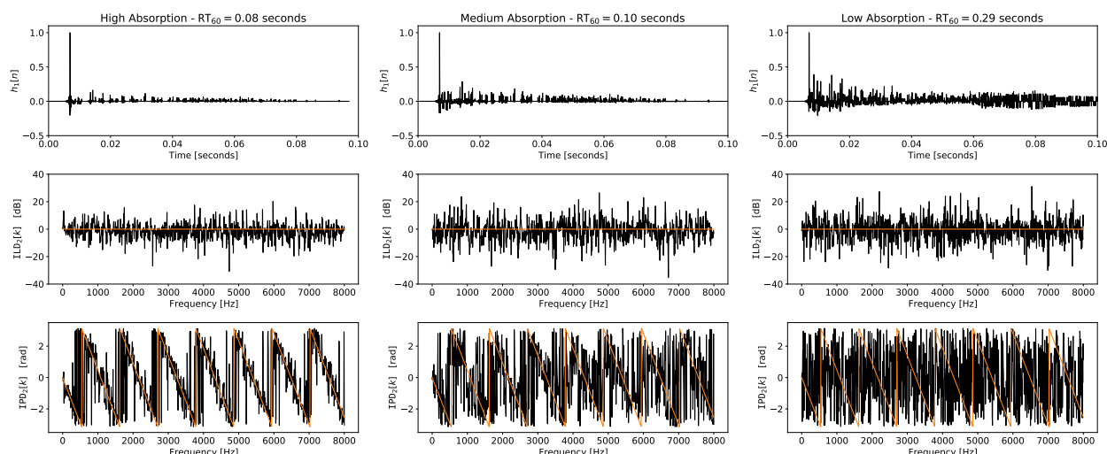
FIGURE 3.8: (Top) Synthetic RIR for different absorption conditions for the reference channel 1. (Below) ILD and IPD related the too channel 2 computed with respect to channel 1. Orange lines denote the theoretical far- and free-field ILD and IPD as defined by the relative steering vectors of Eq. (3.33). As the source is placed far from the microphones, the attenuation is similar on both the channels, whereas the delay is not.
