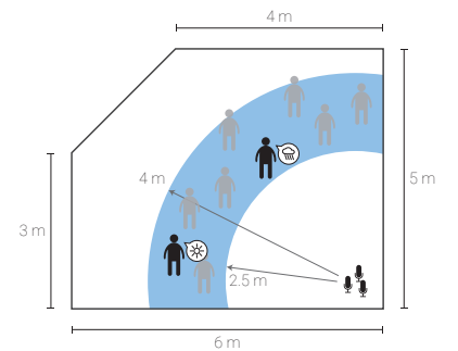
FIGURE 9.5: The simulated scenario. Image taken from the paper of this work [Scheibler et al. 2018c]
