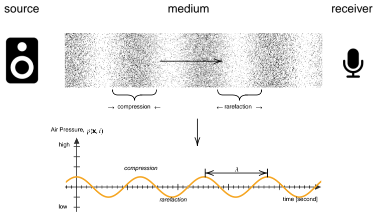
FIGURE 2.2: Illustration of the molecules under sound compression and rarefaction due to longitudinal sound wave and its waveform representation.
