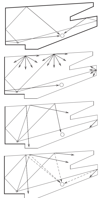
FIGURE 2.13: Visualization of ray-tracing method. From top to bottom: first the method will eventually find specular reflection; then diffuse reflections can be modeled either by splitting a ray into several new rays or a single random one. In the diffuse rain technique a shadow-ray is cast from each diffuse reflection point to the receiver to speed-up convergence of the simulation. Image courtesy of [Savioja and Svensson 2015]
