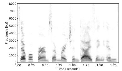
FIGURE 3.7: STFT spectrogram of an example speech signal. Higher energies are illustrated with darker colors.
