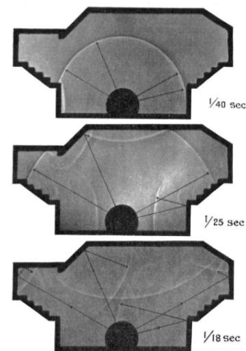
Schlieren photographs showing successive stages in the progress of a sound pulse in a section of a Debating Chamber. Image courtesy of [Davis and Fleming 1926]. Sabine used Schlieren photography to investigate sound propagation paths in the early 1900s. Their impressive visualizations show wavefronts that are augmented with rays that are perpendicular to the wavefronts
