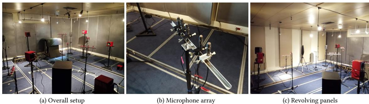
FIGURE 7.3: Picture of the acoustic lab. From left to right: the overall setup, one microphone array, the setup with revolved panels.
