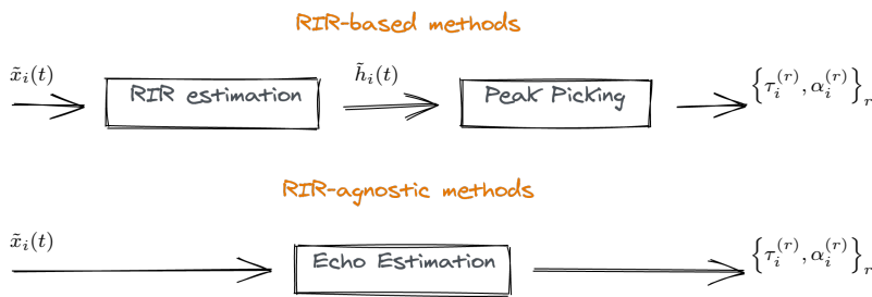
FIGURE 4.2: Schematics of RIR-based and RIR-agnostic approaches.
