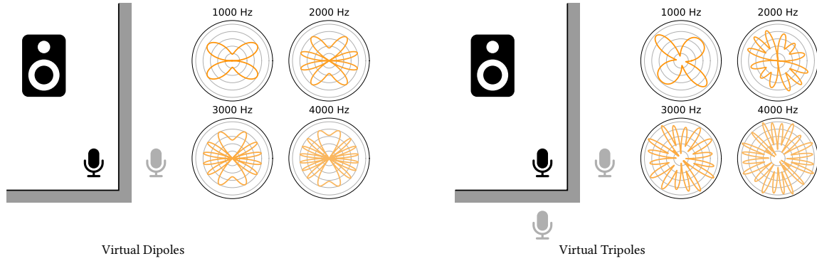
FIGURE 9.2: The frequency-dependent directivity pattern for a virtual array built with a real and one (left) and two (right) image microphones. Image taken from the presentation of the paper [Scheibler et al. 2018c].
