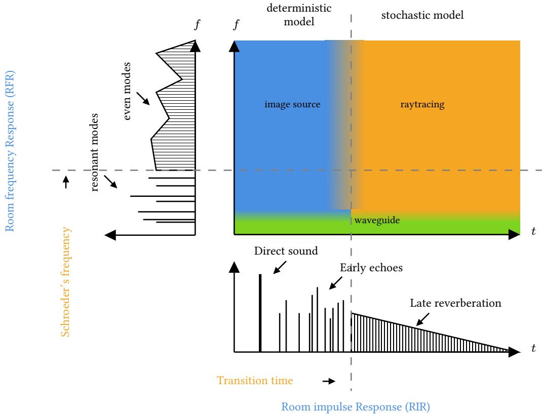
FIGURE 2.14: Time-Frequency regions of the RIR associated to the method that better simulate them. Image adapted from [Thomas 2017; Badeau 2019].
