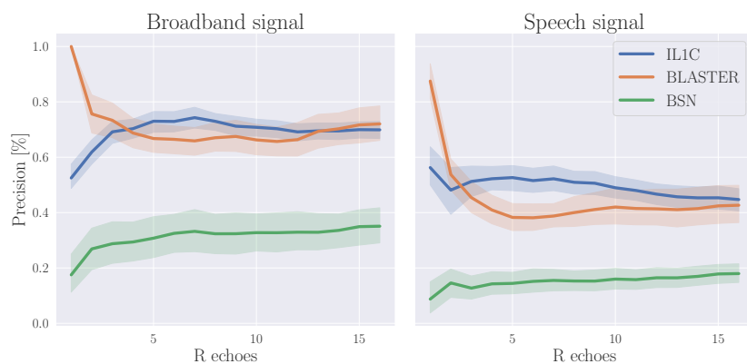
FIGURE 5.5: Precision versus number of echoes R to be retrieved for broadband (left) and speech (right) signals with RT_{60} = 400 ms and SNR = 20 dB. Error bands denotes 95% confidence intervals.
