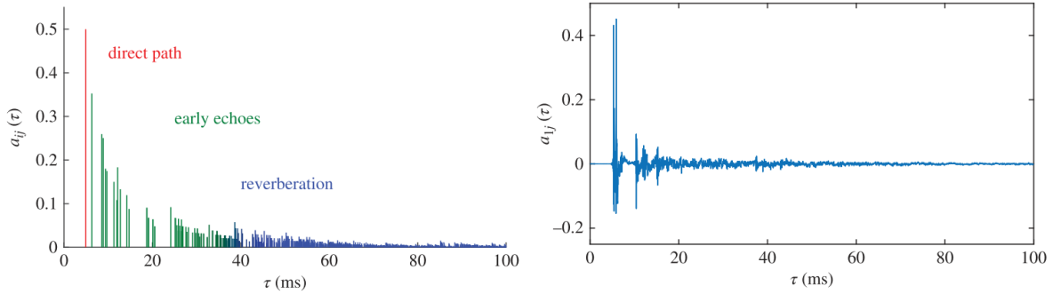
FIGURE 2.9: Schematic illustration of the shape of an RIR and the first 100 ms of a measured one. Image taken from [Vincent et al. 2018]
