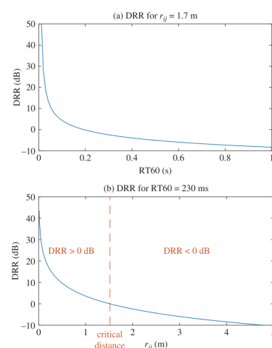
FIGURE 2.17: DRR as a function of the RT_{60} and the source distance r_{ij} based on Eyring's formula (Gustafsson et al., 2003). These curves assume that there is no obstacle between the source and the microphone, so that the direct path exists. The room dimensions are the same as in Figure 3.1.
