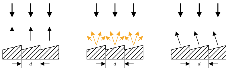
FIGURE 2.6: A reflector having irregularities on its surface with width d much smaller than the sound wavelength \lambda . Image courtesy of [Kuttruff 2016].
