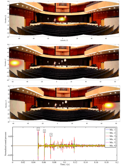
FIGURE 4.5: Visualization of the audio camera: The angular spectrum is overlapped to the corresponding images. Also shown are the impulse responses for 6 microphones. The numbered boxes indicate events shown in the audio camera. Images from [Tervo 2011].
