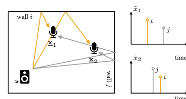
FIGURE 4.3: Illustration of different orders of arrival of wall reflections
