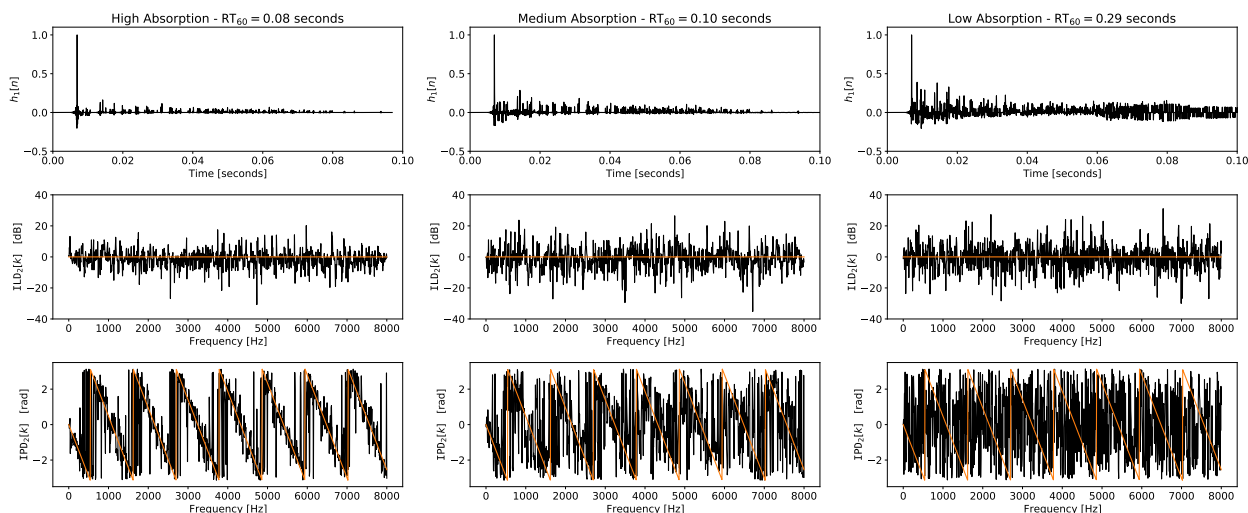
FIGURE 3.8: (Top) Synthetic RIR for different absorption conditions for the reference channel 1. (Below) ILD and IPD related the two channel 2 computed with respect to channel 1. Orange lines denote the theoretical far- and free-field ILD and IPD as defined by the relative steering vectors of Eq. (3.33). As the source is placed far from the microphones, the attenuation is similar on both the channels, whereas the delay is not.
