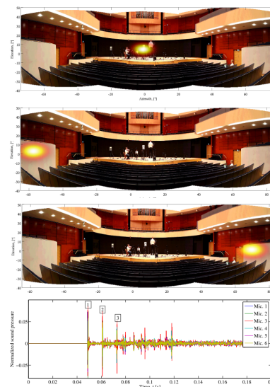
FIGURE 4.5: Visualization of the audio camera: The angular spectrum is overlapped to the corresponding images. Also shown are the impulse responses for 6 microphones. The numbered boxes indicate events shown in the audio camera. Images from [Tervo 2011].
