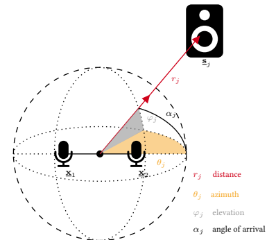
FIGURE 8.3: Geometrical illustration of the Sound Source Localization, showing the azimuth \theta_j , the elevation \varphi_j and angle of arrival \alpha_j for the source j at \underline{s}_j and two microphones at \underline{x}_1, \underline{x}_2 respectively.
