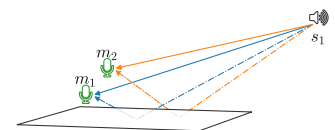
FIGURE 6.1: Typical setup with one sound source recorded by two microphones. The illustration shows the direct sound path (blue lines) and the resulting first-order echoes (orange lines).
