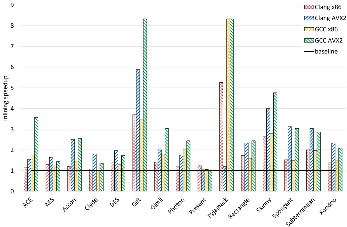
Figure 4.3: Impact on throughput of fully inlining bitsliced ciphers (raw numbers in Table A.3, Page 196)
