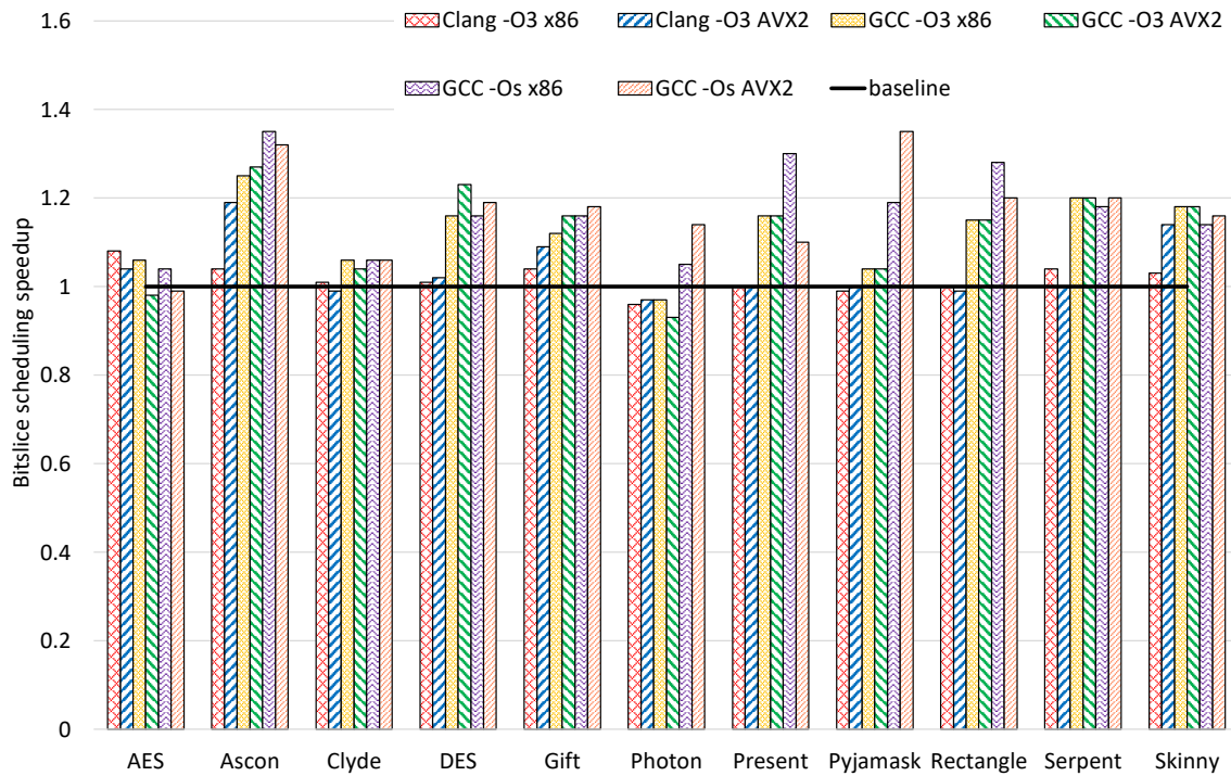
Figure 4.5: Performance of the bitsliced code scheduling algorithm (raw numbers in Table A.4, Page 196)
