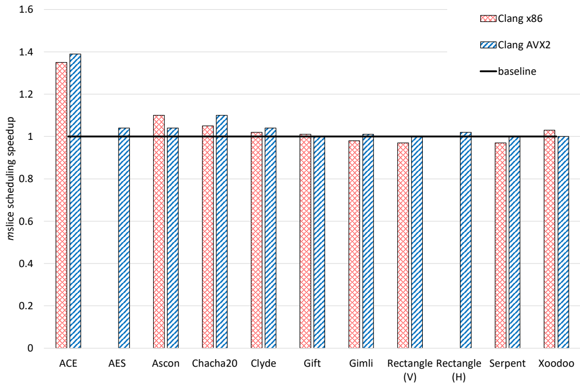
Figure 4.6: Performance of the msliced code scheduling algorithm (raw numbers in Table A.2, Page 195)
