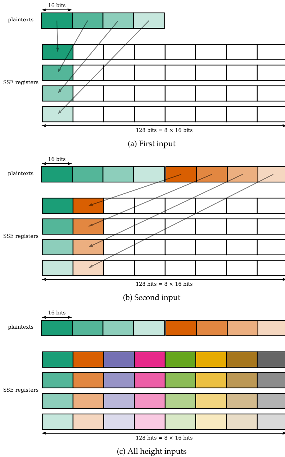
Figure 1.11: Data layout of vsliced RECTANGLE
