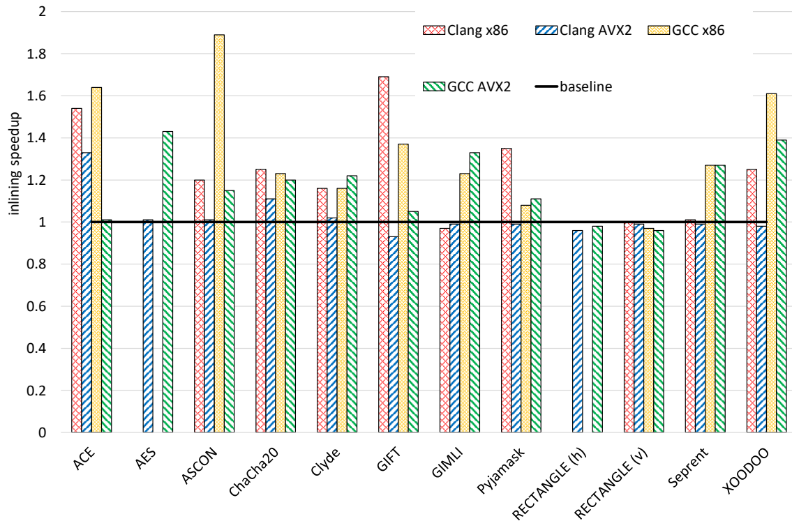
Figure 4.2: Impact on throughput of fully inlining msliced ciphers (raw numbers in Table A.1, Page 195)
