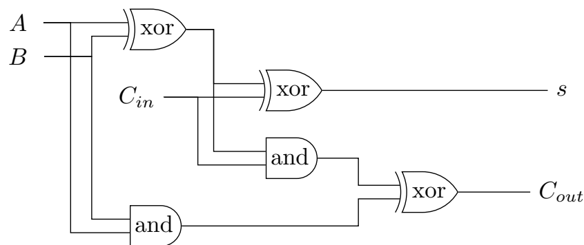
(a) Full-adder
