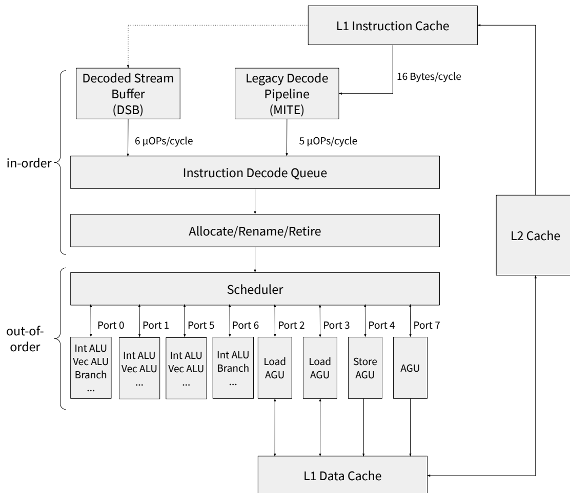
Figure 1.2: Skylake's pipeline
