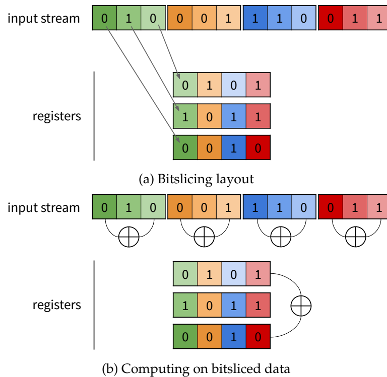
Figure 1.5: Bitslicing example with 3-bit data and 4-bit registers
