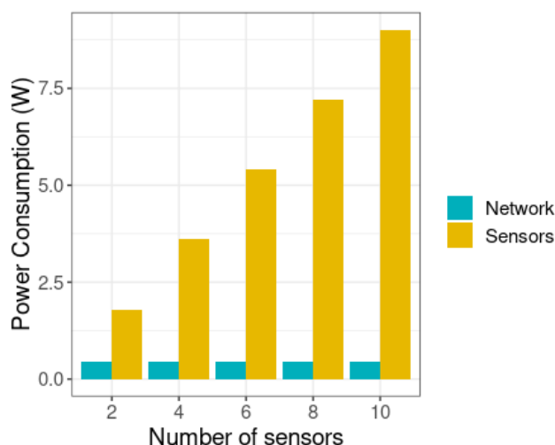
Figure 3.3: Analysis of the variation of the number of sensors on the IoT/Network part energy consumption for a transmission interval of 10s.
