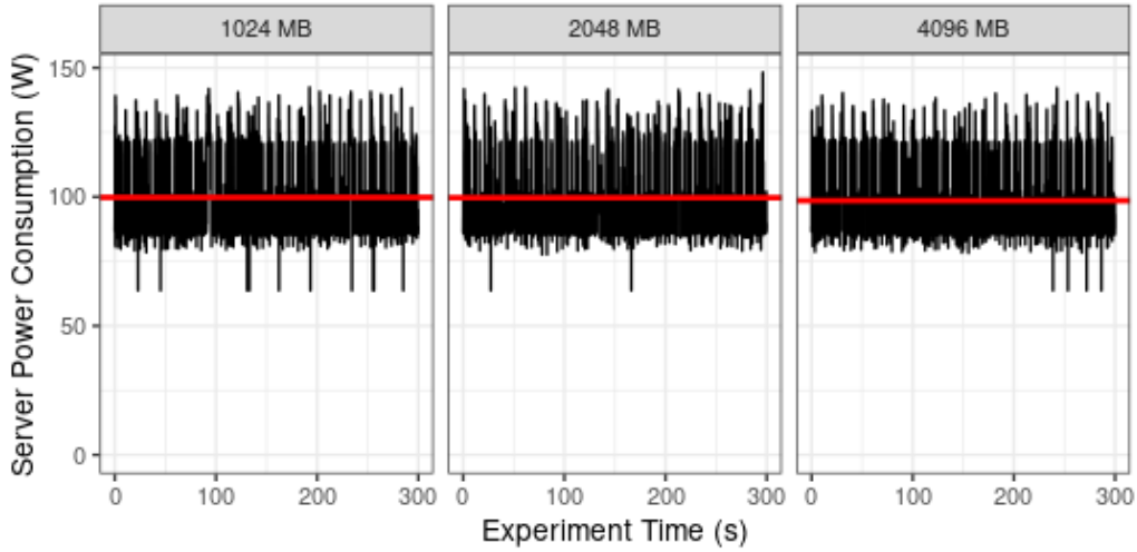
Figure 3.4: Server power consumption multiplied by the PUE ( = 1.2 ) using 20 sensors sending data every 10s for various VM memory sizes.
