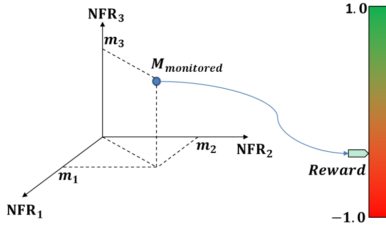
FIGURE 4.5: An example of a mapping between three monitored metrics ( m_1, m_2, m_3 ) of three respective NFRs ( NFR_1, NFR_2, NFR_3 ) and the obtained reward. The reward is clipped in a range of [-1.0, 1.0] , where the best reward is 1.0 and the worst reward is -1.0 .
