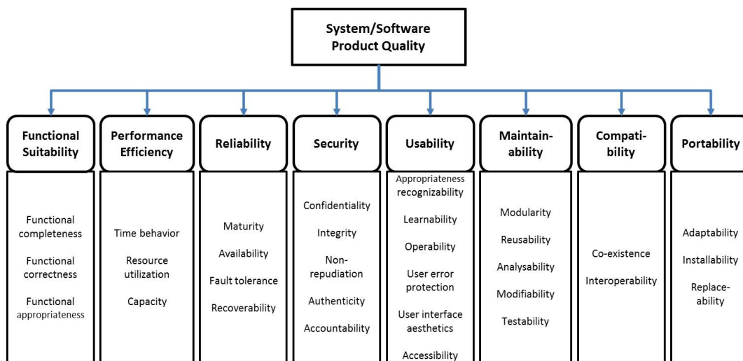
FIGURE 1.4: Product quality model proposed by the ISO 25010. It evaluates the intrinsic quality characteristics of the software or system.
