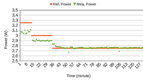
(C) Computing power consumption of Server Mission.
