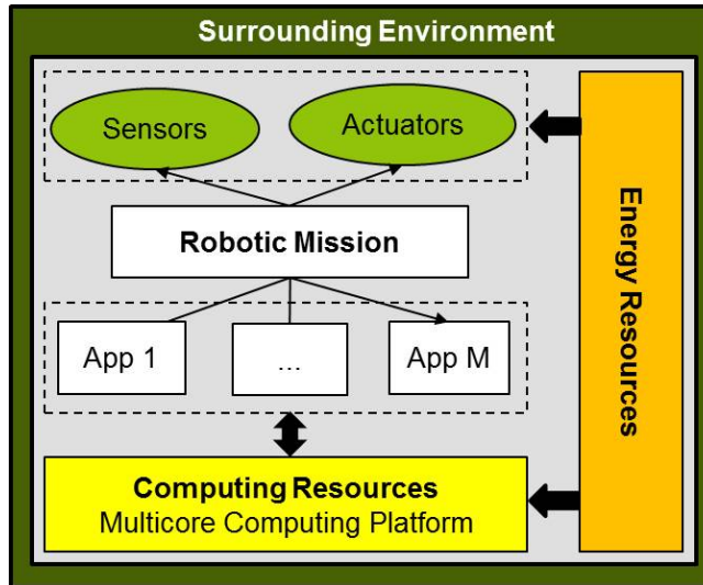
FIGURE 3.2: Mobile robotic mission model with components of sensors, actuators and computing applications, and connection with computing platform, power supply and surrounding environment.
