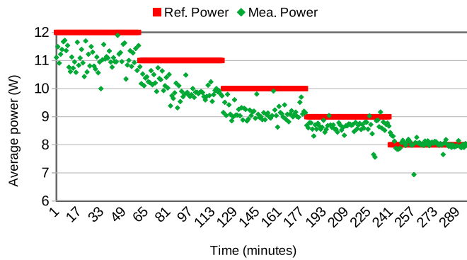
FIGURE 5.9: System-level computing power consumption controlled by the Multi-Mission Manager. The red points indicate the maximum computing power allocated to two missions and the green points are the measured values or the actual computing power (averaged during an episode or a decision epoch of 1 minute of the Multi-Mission Manager) consumed by two missions.
