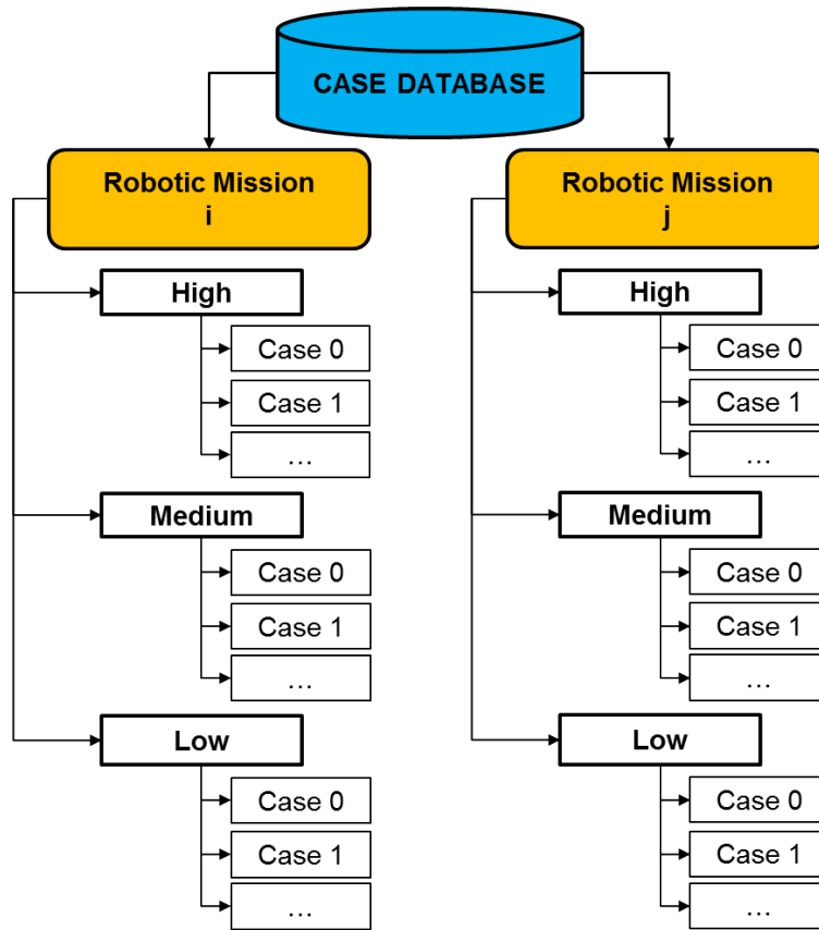
FIGURE 5.6: Case-Based Reasoning for adapting to changing NFRs. For the case base of each mission, the case is first indexed by the computing power mode ( High , Medium , and Low ) and then by other non-functional requirements.
