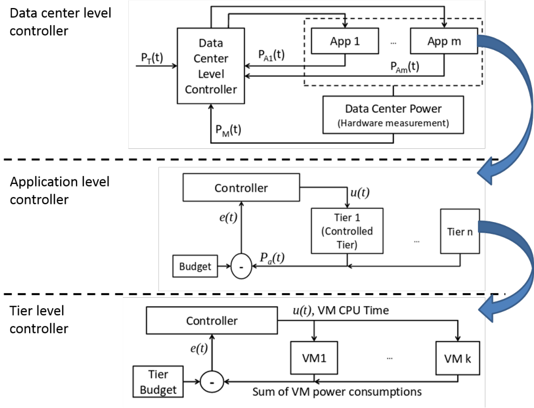
FIGURE 5.1: Hierarchical management in data center (adapted from [Lim, Kansal, and Liu, 2011]). The adaptive management is defined at three levels: data center, application and tier level.
