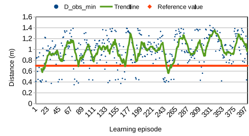
(B) Minimum distance to obstacles.
