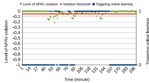
(G) NFRs violation and online learning triggering of Server Mission.
