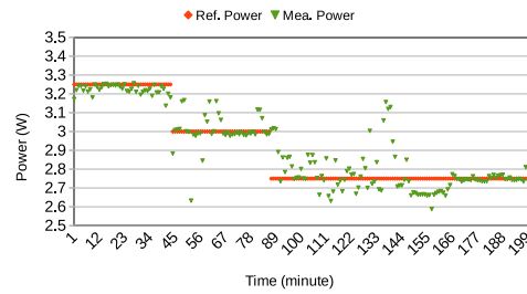
(C) Computing power consumption of Server Mission.
