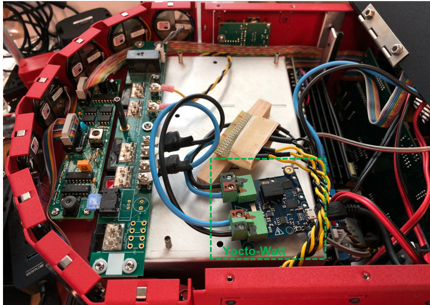
FIGURE D.1: Install Yocto-Watt in Pioneer-3DX mobile base.
