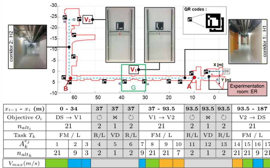
FIGURE 2.21: Mission decomposition (reprinted from [Jaiem et al., 2016b]). The mission is divided into several objectives. For each objective, there are a number of alternative implementations ( n_{alt} ) that can be chosen for deployment.
