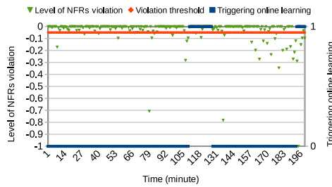
(F) NFRs violation and online learning triggering of Navigation Mission.
