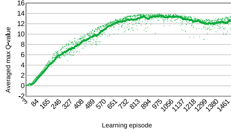
(B) Average max Q-value of Server Mission.
