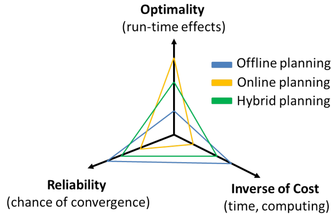
FIGURE 2.9: Planning strategy in self-adaptive systems. The three strategies are evaluated in terms of optimality, reliability and computing cost.
