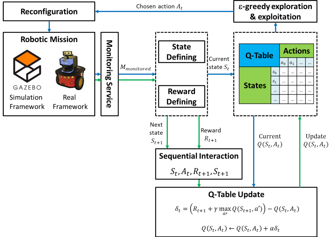
FIGURE 4.7: Q-Learning implementation details.
