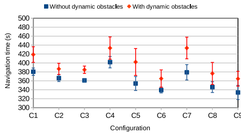
(A) Navigation time. The lower is the better.
