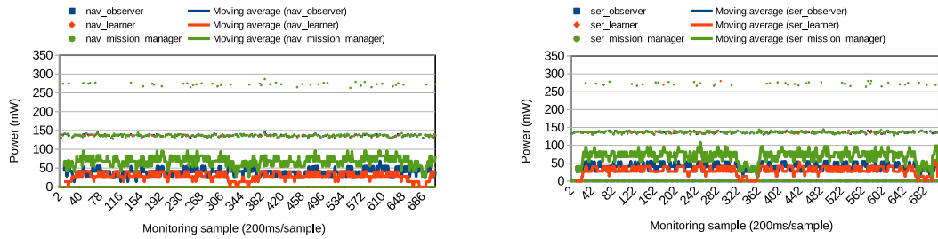
(A) Power consumption of Navigation Mission Manager: 70mW in average.
