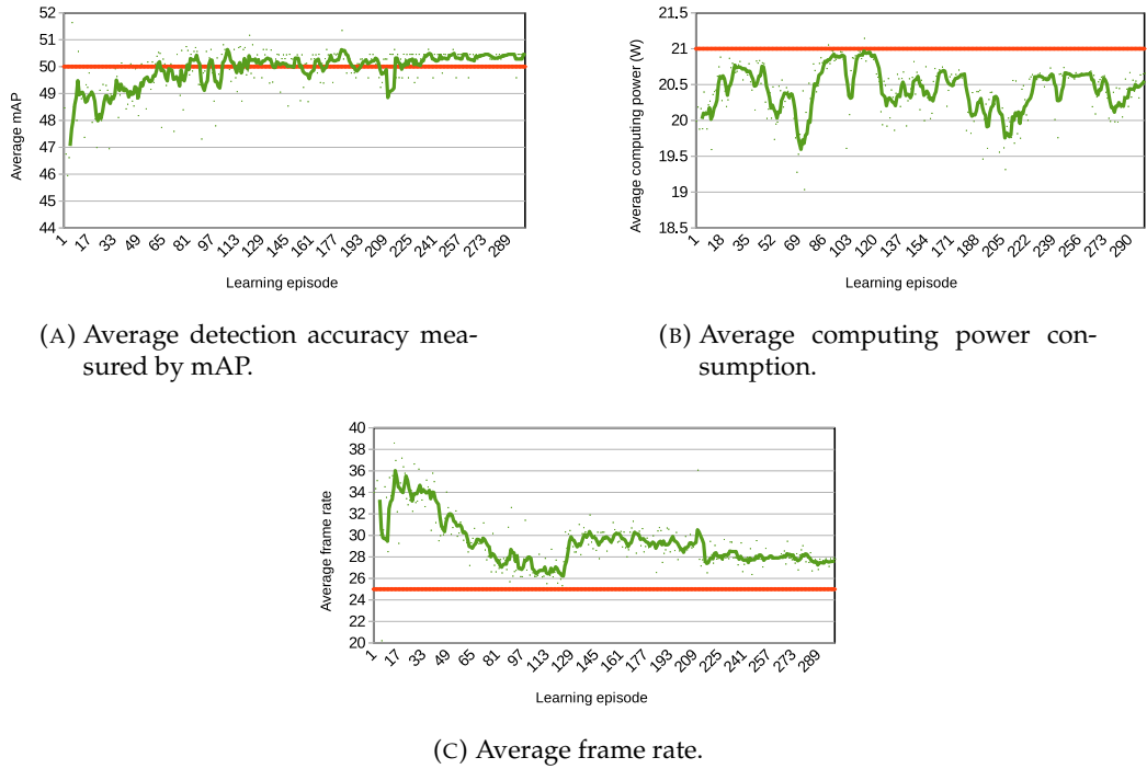
FIGURE 6.18: Learning phase results of a semantic mission manager at the High computing power mode: non-functional requirements.
