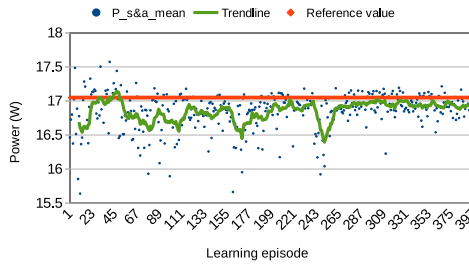
(C) Mean sensing&acting power consumption.
