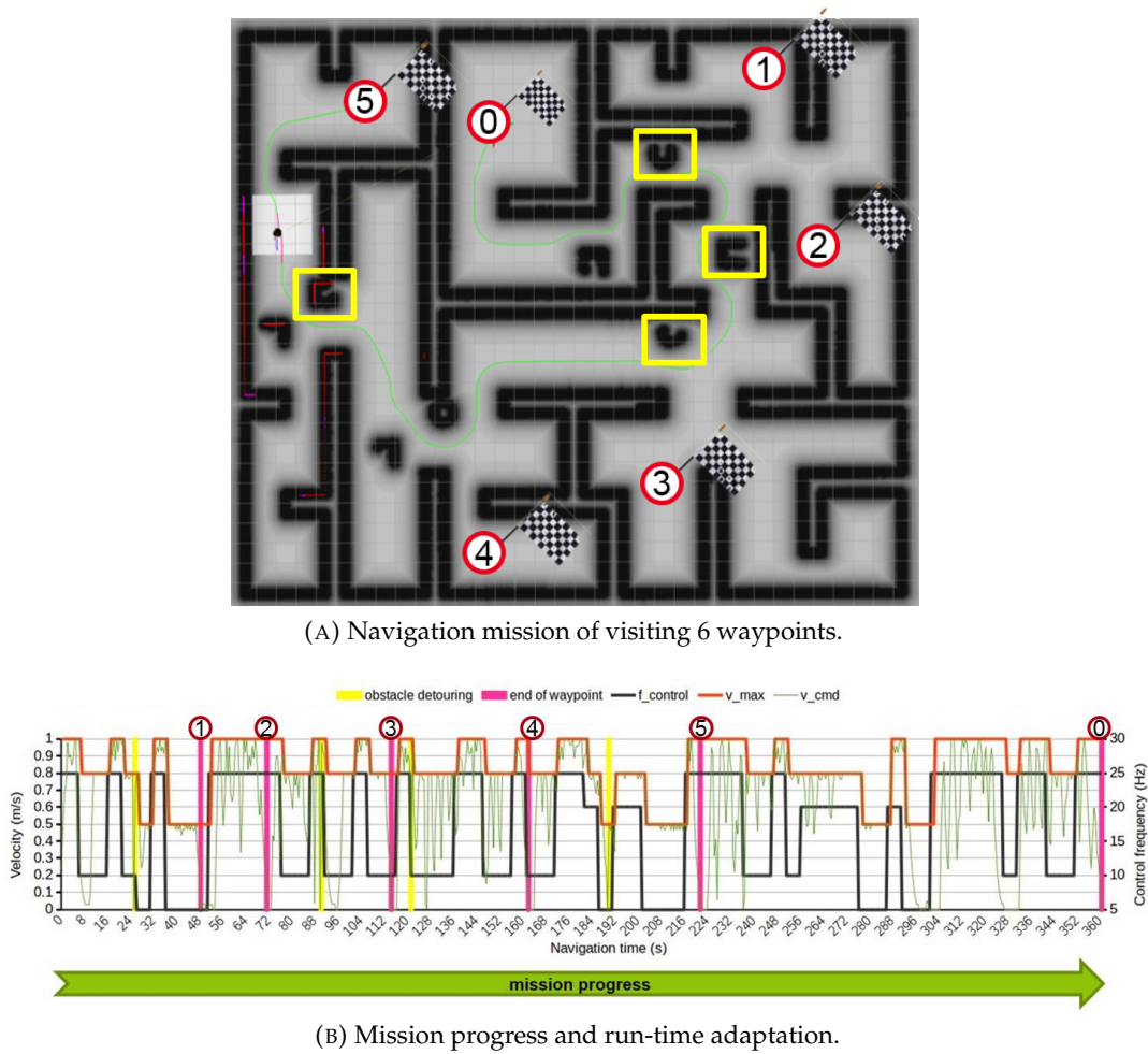
FIGURE 4.18: Example of run-time adaptation during a navigation mission of visiting a set of 6 waypoints. The max robot velocity v_{max} and control frequency f_{control} are dynamically reconfigured by our proposed mission manager whilst targeting the four required non-functional goals. The v_{cmd} is the actual velocity sent by the navigation mission in order to command directly the mobile base.
