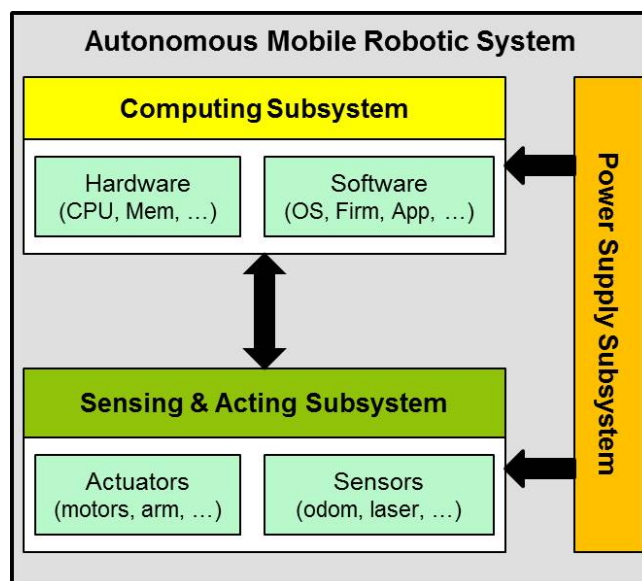
FIGURE 2.1: Generic structure of mobile robotic systems. A mobile robotic system is composed of three main subsystems: sensing and acting, computing and power supply subsystems.
