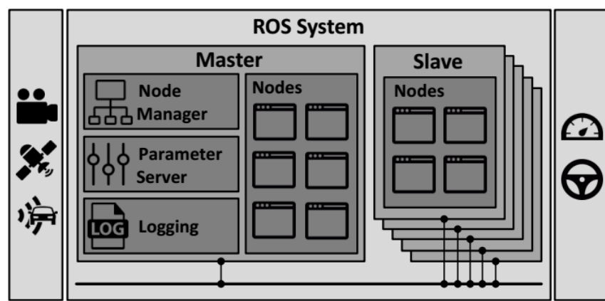
FIGURE 2.4: ROS system architecture (reprinted from [Hellmund et al., 2016]). Each hardware and software component in the system is managed by ROS nodes and all the nodes are managed by a central ROS master. After registering with ROS master, the communication between ROS nodes is direct.
