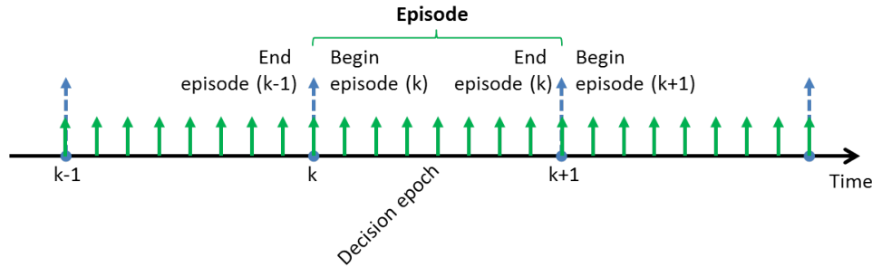
FIGURE 2.15: Illustration of episodes and decision epochs in the reinforcement learning. An episode is composed of many decision epochs.
