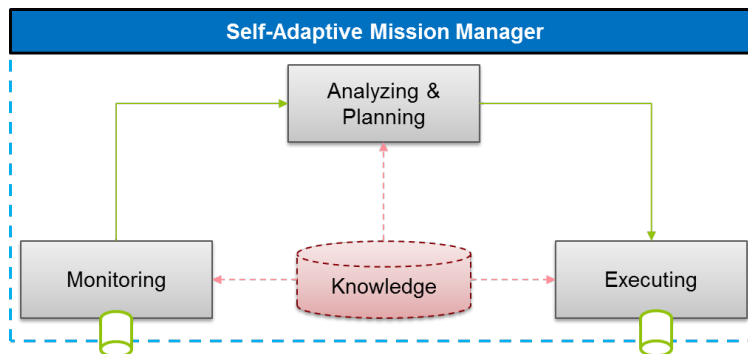
FIGURE 7.2: Mission knowledge used for the run-time adaptation algorithm.
