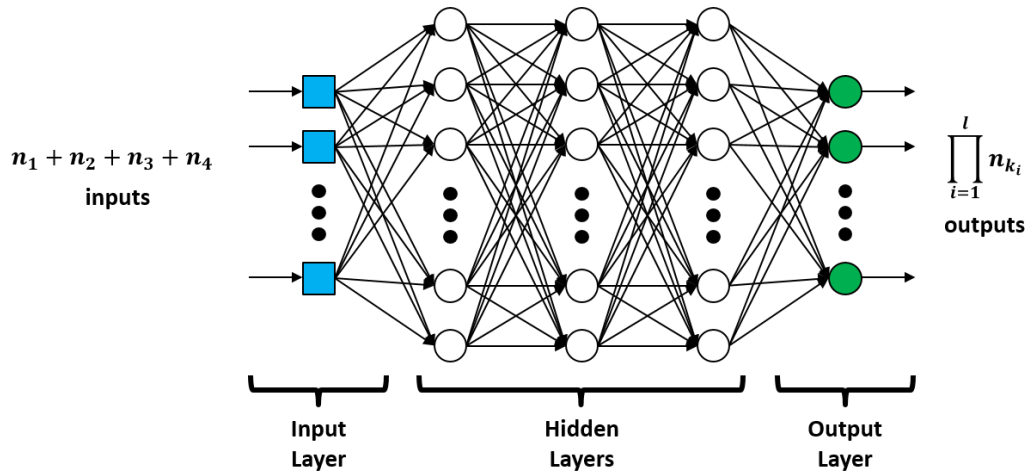
FIGURE 4.9: Q-Network structure: a Multi-Layer Perceptron (MLP) with an input layer of (n_1 + n_2 + n_3 + n_4) neurons, a number of hidden layers and an output layer of \prod_{i=1}^l n_{k_i} neurons.
