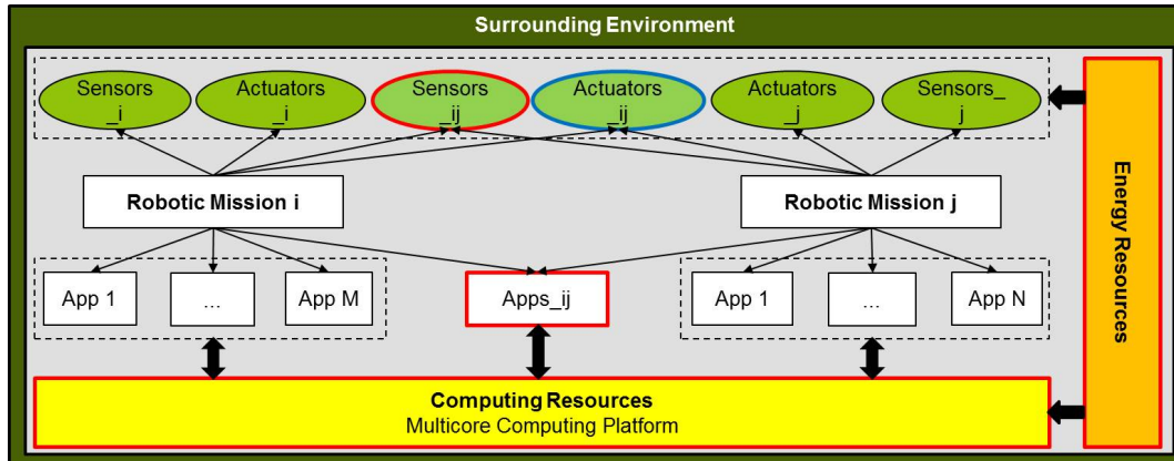
FIGURE 3.8: Multi-Mission context. Here, two example missions i and j can share resources (sensors, actuators, computing resources) and energy in a mutex locked (blue contour) or superposed manner (red contour).
