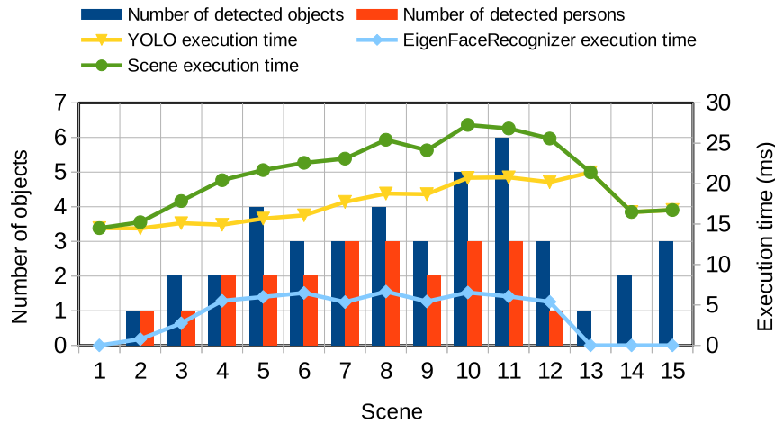
FIGURE 3.19: The non-functional properties of the semantic mission depend on the scene. In this case, 15 scenes with a different number of objects and people detected give different execution times (inverse of the frame rate) and therefore the power consumption of the semantic mission.
