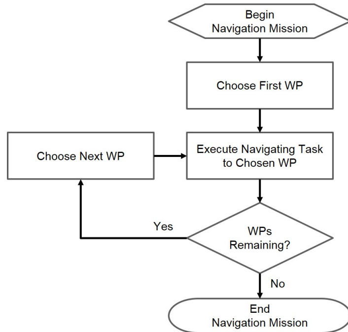
FIGURE 3.1: Example of an autonomous navigation mission: task sequencing algorithm (adapted from [Brutzman et al., 2018] for a navigation mission). Note: WP - waypoint.
