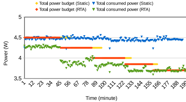
FIGURE 6.10: System-level computing power consumption.
