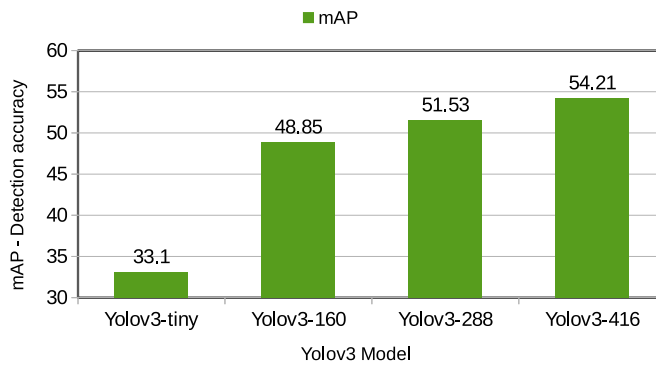
FIGURE 3.20: Detection accuracy of four Yolov3 models.
