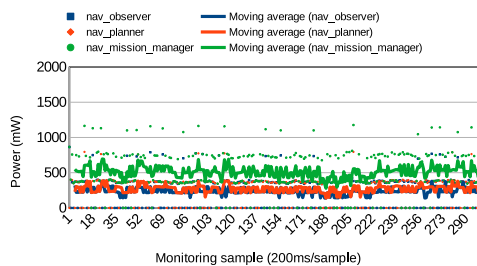
(A) Power consumption of Navigation Mission Manager: 505mW in average.
