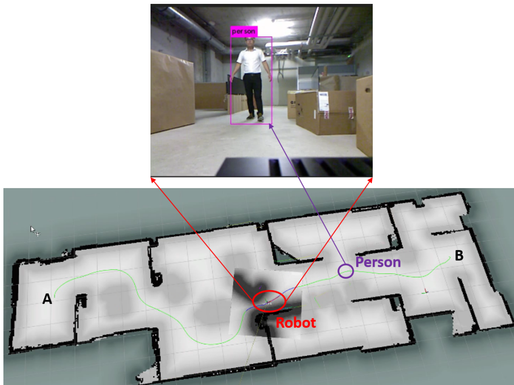
FIGURE 6.16: Integration of a semantic environment understanding mission into the multi-mission context on the real robotic platform. The robot is navigating from A to B and the semantic mission is in charge of detecting and recognizing the objects including people in the environment.
