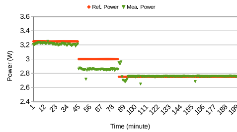
(B) Computing power consumption (RTA).
