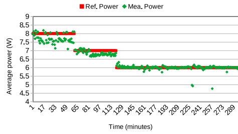
(B) Computing power consumption of Server Mission.
