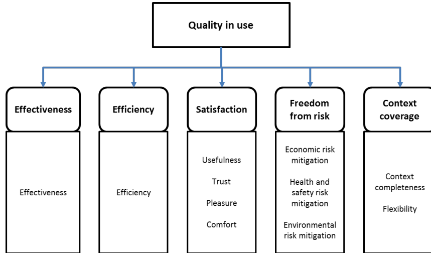
FIGURE 1.5: Quality in use model proposed by the ISO 25010. It evaluates the quality characteristics of the system or software when it is used under a specific context.
