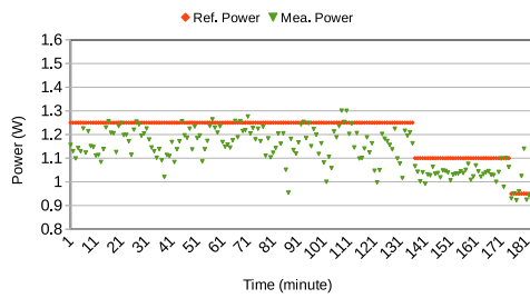
(B) Computing power consumption of Navigation Mission.
