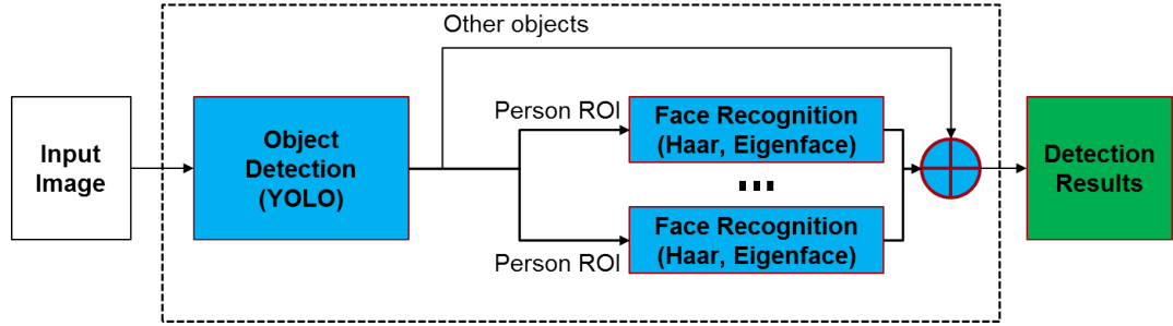
FIGURE 3.18: Semantic Environment Understanding Mission. Its functional requirement is to understand the scene by detecting and recognizing the objects and people in the robot’s working environment.
