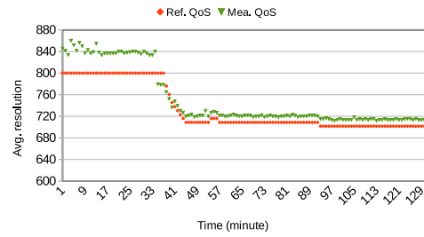
(E) Quality of service of Server Mission.
