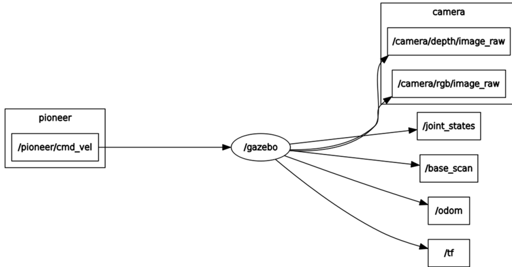
FIGURE 3.13: Simulating robot’s sensors and actuators in Gazebo. The robot simulated in Gazebo receives the velocity command from the navigation’s applications for controlling simulated actuators (motors), and publishes the data from simulated sensors such as depth and color images of RGBD camera, LIDAR scanner, odometry, etc.
