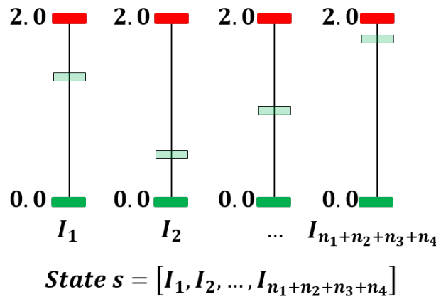
FIGURE 4.6: State formulation for the Deep Q-Learning approach. A state is an 1D vector of (n_1 + n_2 + n_3 + n_4) continuous elements. The state space is therefore infinite.
