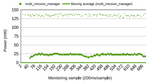
FIGURE 6.15: Power consumption of Multi-Mission Manager: 25mW in average.
