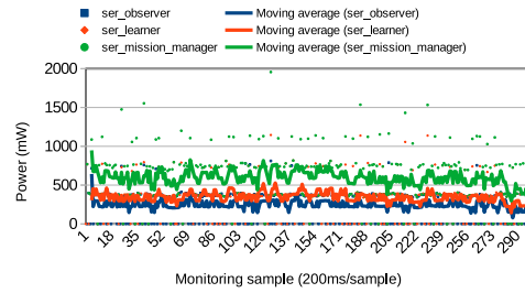
(B) Power consumption of Server Mission Manager: 597mW in average.
