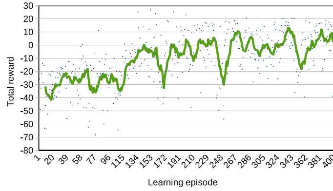
FIGURE 4.13: Total reward of the learning phase over 400 episodes of Q-Learning based Navigation Mission Manager with the trend line in green. The growth of total reward during learning indicates the evolution of the adaptation policy.
