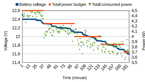
(A) System-level computing power consumption controlled by the Multi-Mission Manager
