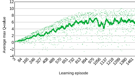
(A) Average max Q-value of Navigation Mission.
