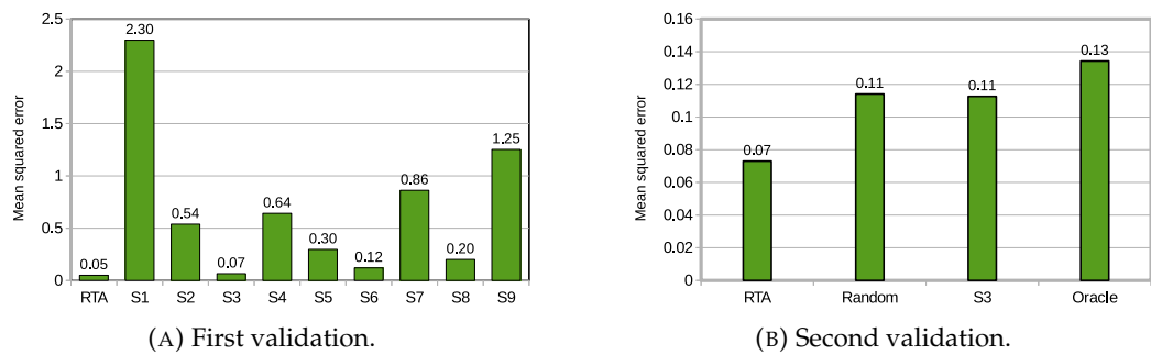
FIGURE 4.17: Mean squared error (Note: the environmental context between two validations is different).
