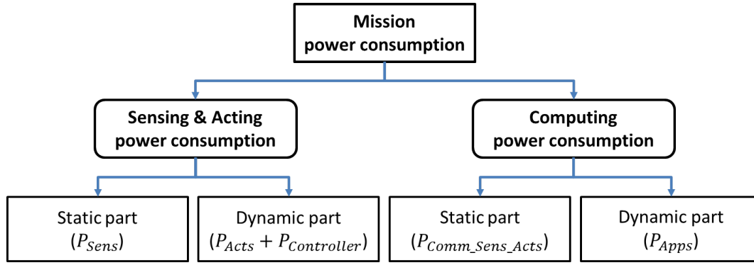
FIGURE 3.4: Mission power consumption model.
