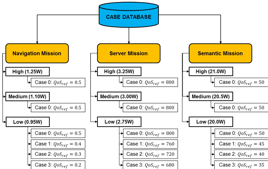
FIGURE 6.19: An initialization of the case database for the navigation mission, the server mission and the semantic mission in the real experimentation.
