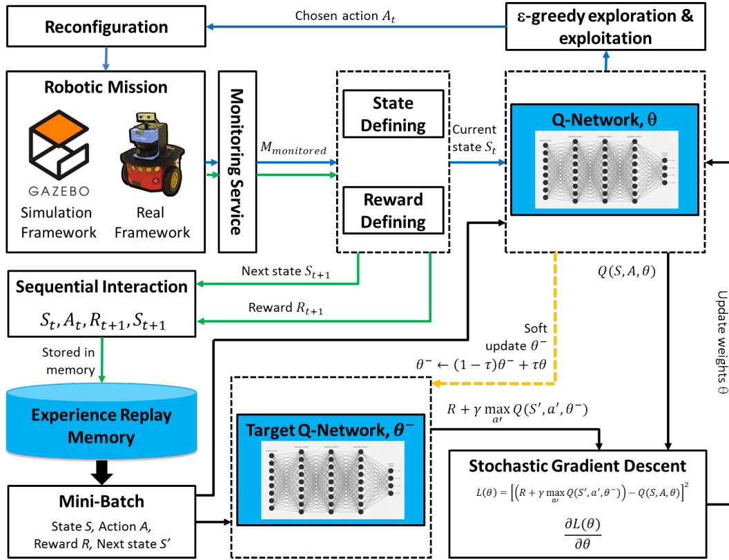
FIGURE 4.8: Deep Q-Learning implementation details.
