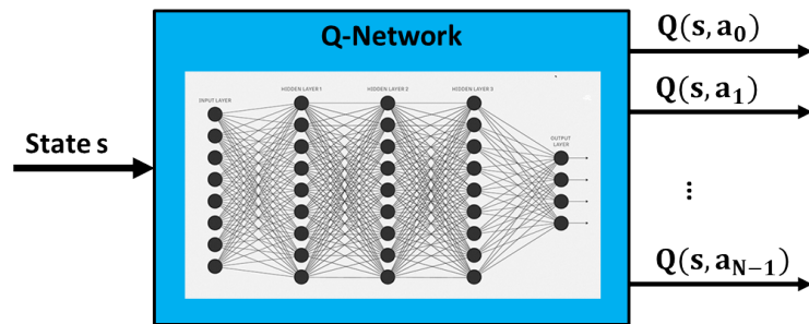
FIGURE 2.14: Deep Q-Network approach. In this approach, the state space is continuous, the action space is still discrete, and the Q-values are estimated by a Q-Network.
