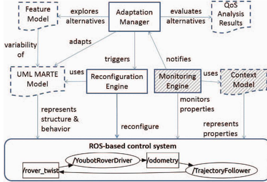
FIGURE 2.22: Model-based reconfigurable robotic systems: the architecture of the reconfiguration system (reprinted from [Brugali et al., 2018]).
