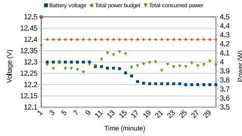
(A) System-level computing power consumption controlled by the Multi-Mission Manager
