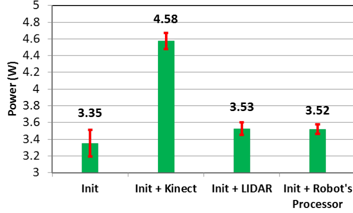
FIGURE D.3: Power consumption reserved for the communication between the Xavier board and its external devices.
