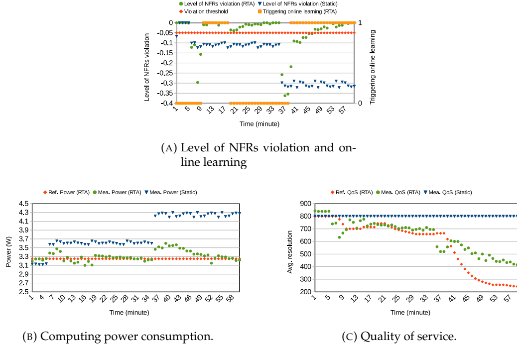
FIGURE 6.9: A comparison between run-time adaptation and static configuration of the video server mission. From 1 to 5 minutes: 1 visualization request of 512 \times 512 . From 6 to 35 minutes: 2 visualization requests of 512 \times 512 . From 36 to 60 minutes: 2 visualization requests, one of 512 \times 512 and another of 1024 \times 1024 .
