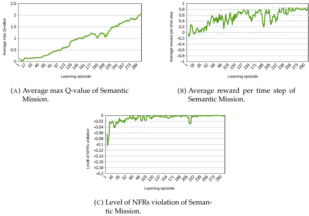
FIGURE 6.17: Learning phase results of a DQN-based semantic mission manager at the High computing power mode.
