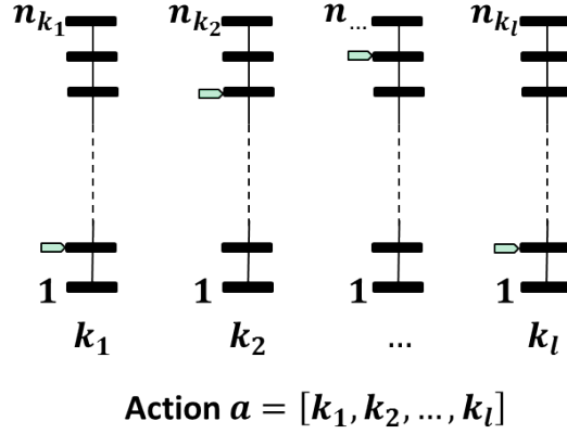
FIGURE 4.4: Action formulation for Q-Learning approach. An action space of \prod_{i=1}^l n_{k_i} actions is formulated.
