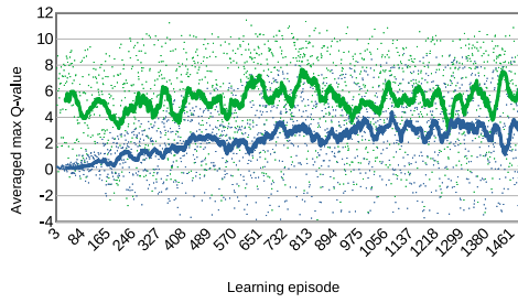
(A) Average max Q-value of Navigation Mission.
