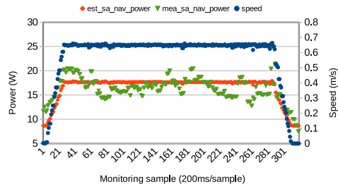
(B) At the robot speed of 0.65m/s.
