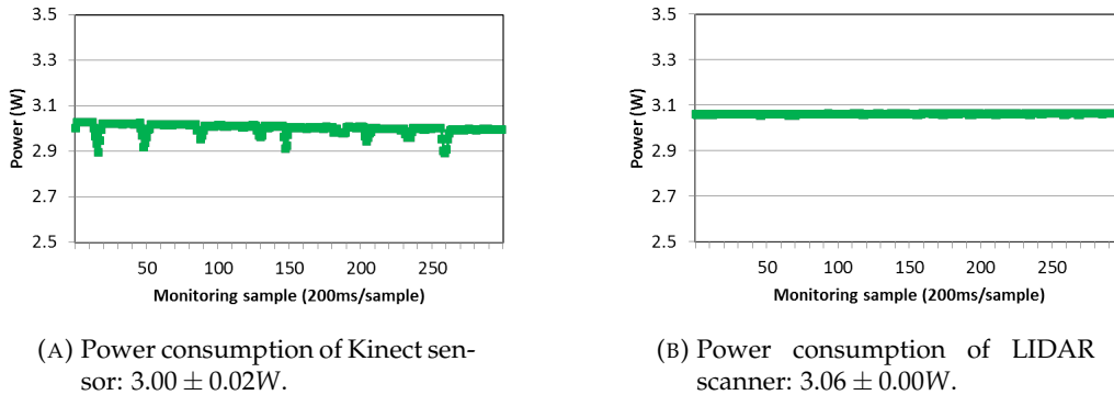
FIGURE D.2: Estimated power consumption of Kinect and LIDAR sensors using Yocto-Watt.
