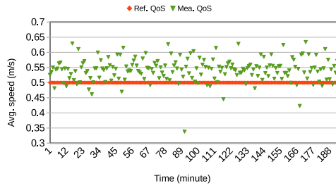
(C) Quality of service (Static).
