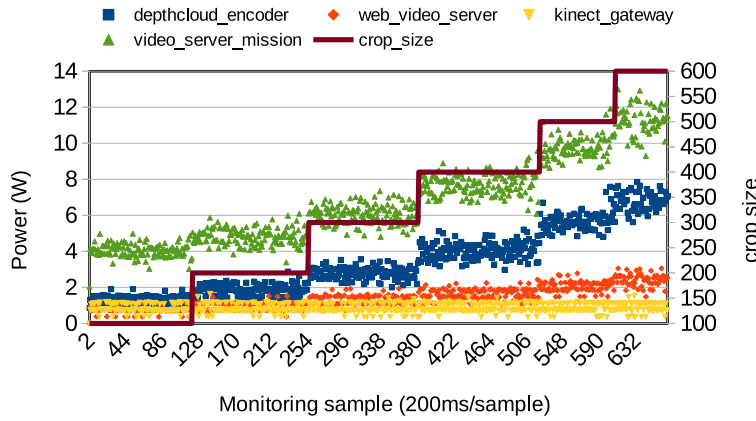
(A) crop_size vs. power consumption with 1 visualization request.
