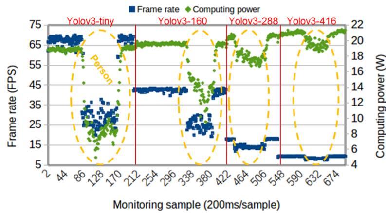
(B) YOLOv3 model vs. frame rate and power consumption in case of person appearance
