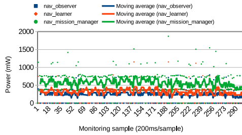
(A) Power consumption of Navigation Mission Manager: 566mW in average.
