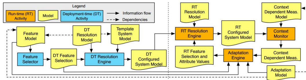
FIGURE 2.19: An overview of the model-based variability management approach (reprinted from [Gherardi and Hochgeschwender, 2015]). A set of models representing the system architecture, its variability, and the state of the context is defined at the design time and is used at run-time to implement the run-time adaptation.
