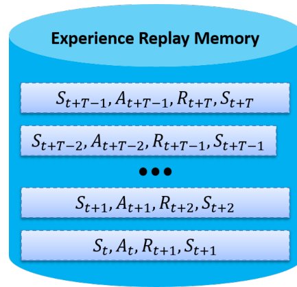
FIGURE 4.10: Experience replay memory of T transitions.
