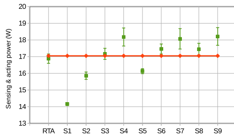
(C) Mean sensing&amp;acting power consumption.
