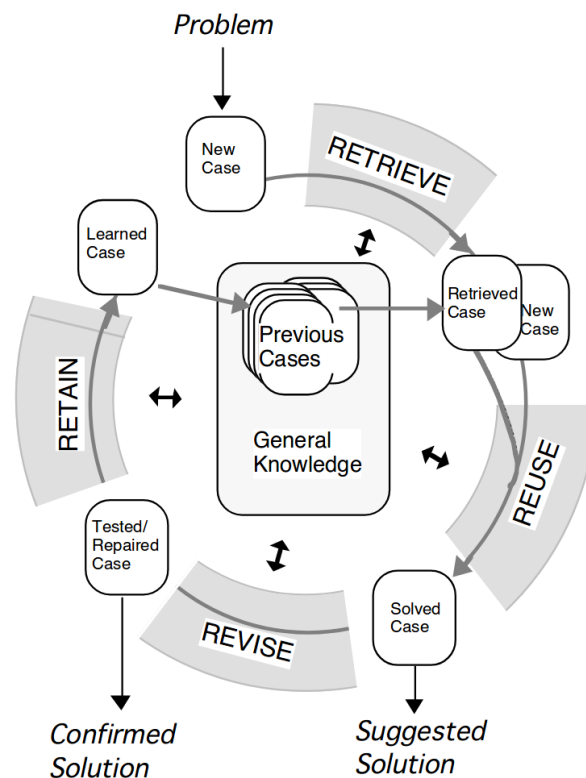
FIGURE 2.11: Case-Based Reasoning cycle uses a four-step process: Retrieve, Reuse, Revise and Retain (reprinted from [Aamodt and Plaza, 1994]).
