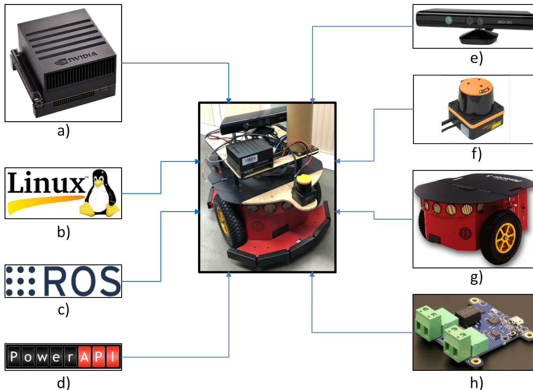
FIGURE 3.11: Our real robotic platform for experimentation: a) NVIDIA Jetson Xavier, b) Linux-based operating system, c) Robot Operating System, d) Process-level power estimation by PowerAPI, e) Kinect sensor, f) Hokuyo laser scanner, g) Pioneer-3DX mobile base and h) Power consumption measurement by Yocto-Watt.
