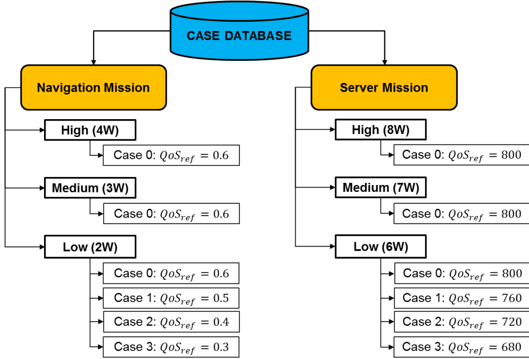
FIGURE 5.8: An initialization of the case database for the navigation mission and the server mission.
