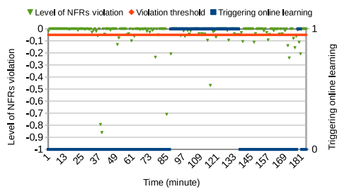
(F) NFRs violation and online learning triggering of Navigation Mission.
