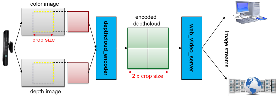
FIGURE 3.16: Video Server Mission. Its functional requirement is to provide the visual information of the working environment in the form of encoded depthclouds for the users.
