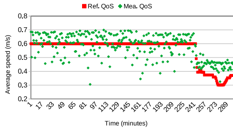
(C) Quality of service of Navigation Mission.
