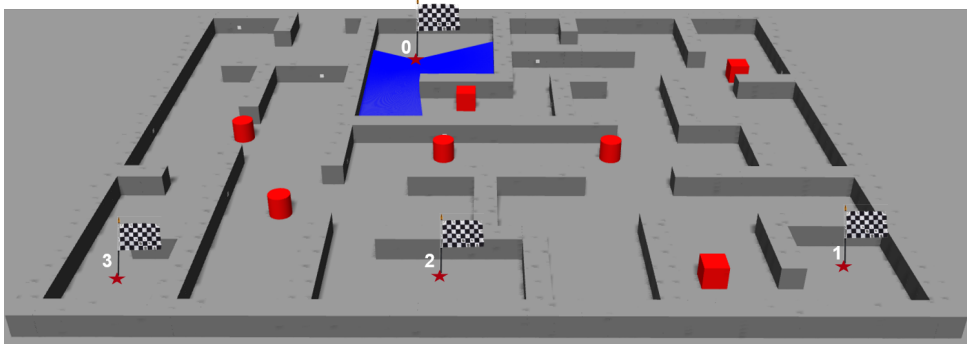
FIGURE 4.12: Example of a simulation environment in Gazebo with 7 dynamic obstacles: single box or cylinder in red models dynamic obstacles, blue area represents laser scan. The flags represent the examples of navigation waypoints.
