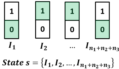
FIGURE 4.3: State formulation for the Q-Learning approach. A state space of 2^{n_1+n_2+n_3} states is formulated.
