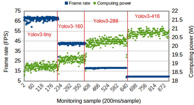
(A) YOLOv3 model vs. frame rate and power consumption
