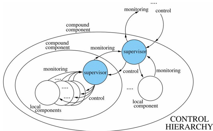
FIGURE 2.16: Component-based run-time self-adaptation: hybrid control hierarchy at local and compound robotic components (reprinted from [Hernandez-Sosa et al., 2005]).
