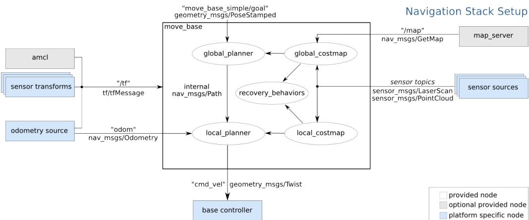
FIGURE 3.14: Autonomous Navigation Mission based on a ROS Navigation Stack. Its functional requirement is to visit a user-defined set of waypoints in the working environment based on a global map.
