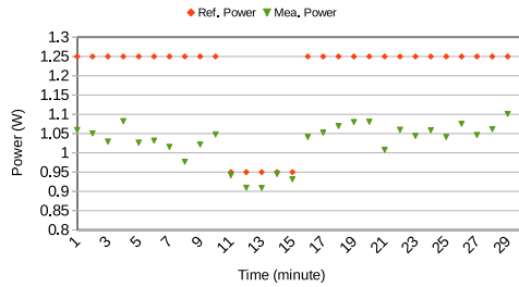
(B) Computing power consumption of Navigation Mission.
