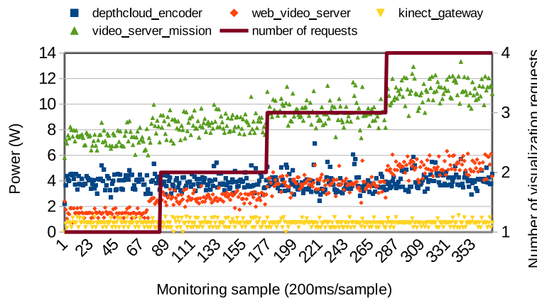
(B) visualization requests vs. power consumption with crop_size =400.
