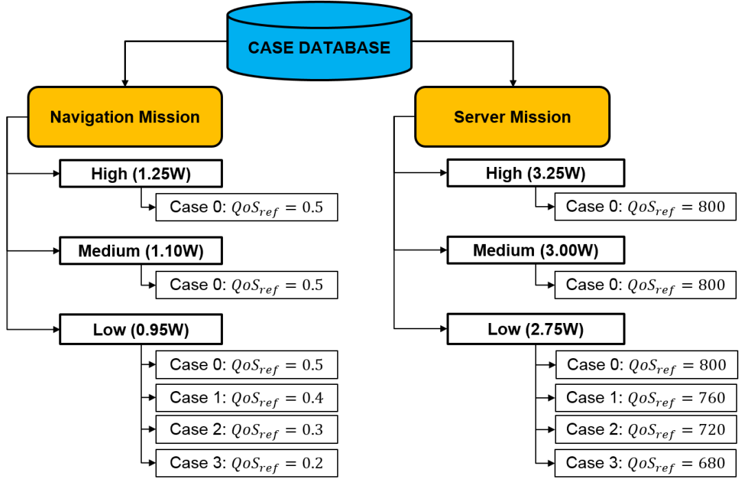
FIGURE 6.3: An initialization of the case database for the navigation mission and the server mission in the real experimentation. The learned adaptation models in the simulation framework are reused in the real experimentation.
