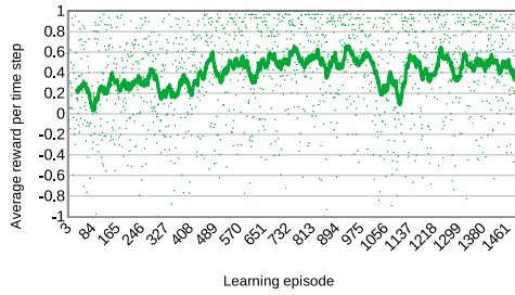
(C) Average reward per time step of Navigation Mission.
