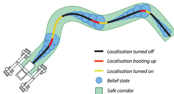
FIGURE 2.20: Scheduling perception for energy efficiency: scheduling decisions based on belief state in the safe corridor (reprinted from [Ondrúška et al., 2015]).
