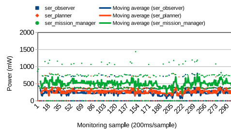
(B) Power consumption of Server Mission Manager: 510mW in average.
