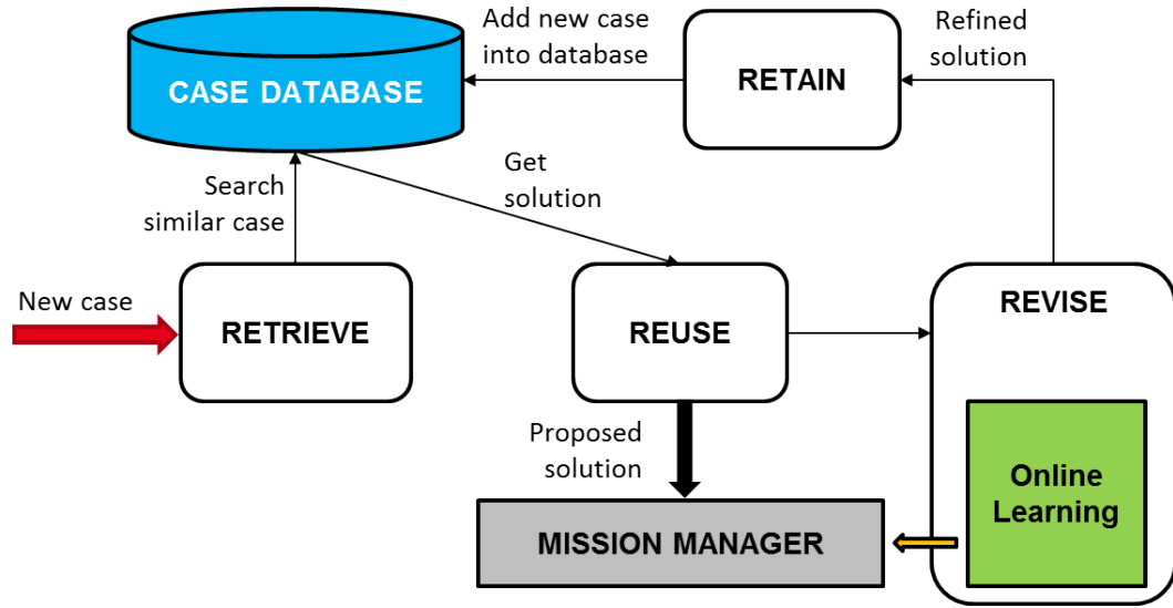
FIGURE 5.7: Case-Based Reasoning cycle for each robotic mission: Retrieve, Reuse, Revise and Retain. The online learning capability is included in the revise step.
