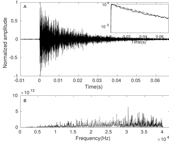
Figure 2.6: (A) Example of the Lamb waves recorded by a transducer after pulse compression of the emitted chirp signal. The source-receiver distance is about 21 cm. The inset illustrates the envelope of the intensity of the signal (solid line) and the exponential fit according to \exp(-t/\tau_a) (dashed line), as a semilog scale. The attenuation time ( \tau_a ) is 9 ms. Data at negative time gives a sense of the noise level. (B) Power spectrum of the raw signal (black) and bandpass filtered one (gray). The data is filtered between 15 kHz and 30 kHz using a Butterworth filter of 4th order.
