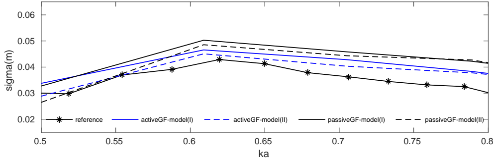
Figure 3.13: Total scattering cross-sections obtained for the cylindrical magnet of 12 mm diameter and 5 mm height for the different methods and different data. Solid line with stars, reference curve obtained by the conventional method based on direct arrivals; solid blue line, case I for the active Green’s function; dashed blue line, case II for the active Green’s function; solid black line, case I for the passive Green’s function; dashed black line, case II for the passive Green’s function.
