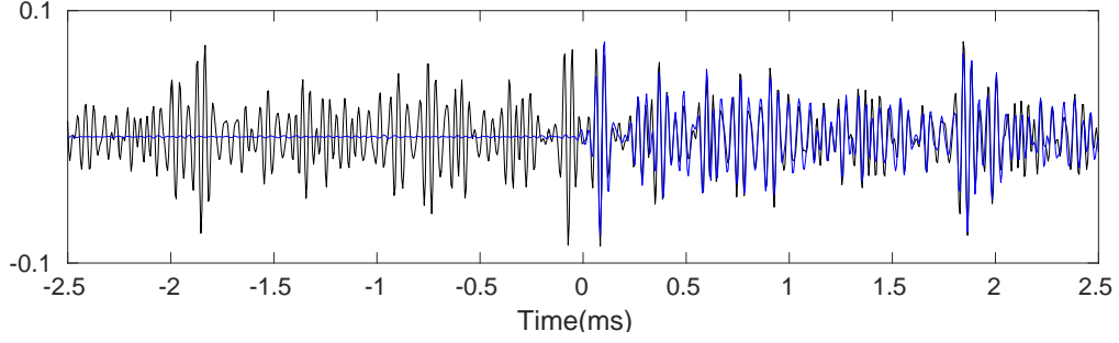
Figure 2.10: Comparison of the normalized cross-correlation averaged over all of the source positions when the sources are distributed on a circle (black), and direct measurement of the source-to-receiver 'time-integrated' impulse response (blue) in the frequency band of 15 kHz to 30 kHz.
