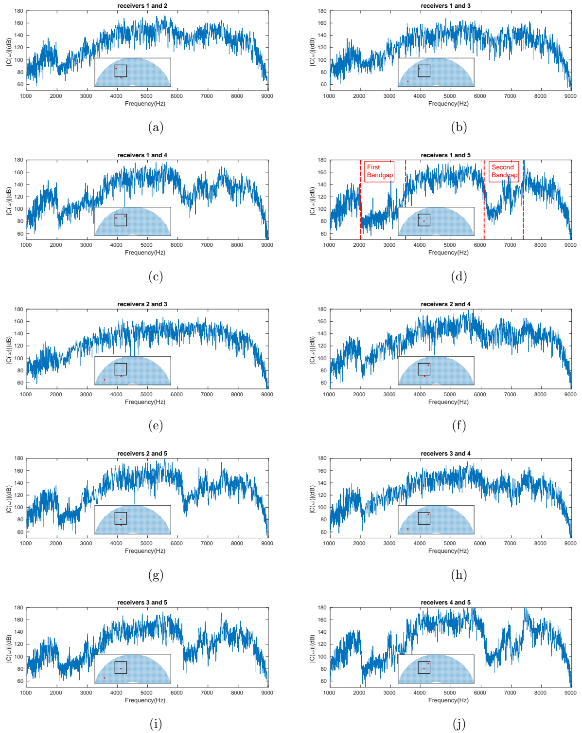
Figure 4.23: Amplitude spectra of the averaged cross-correlation (dB) over all of the possible virtual sources. Different panels correspond to different pairs of virtual receivers. Red circles mark the position of these virtual receivers.
