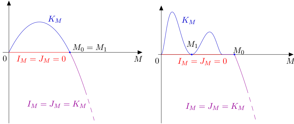
Figure 4.1: Two possible graphs representing I_M, J_M, K_M as a function of the mass M . Note that nothing ensures that these functions are differentiable as the picture might indicate. The right picture corresponds to the case where M_1 < M_0 , while M_1 joins M_0 on the left, which could be the expected situation.
