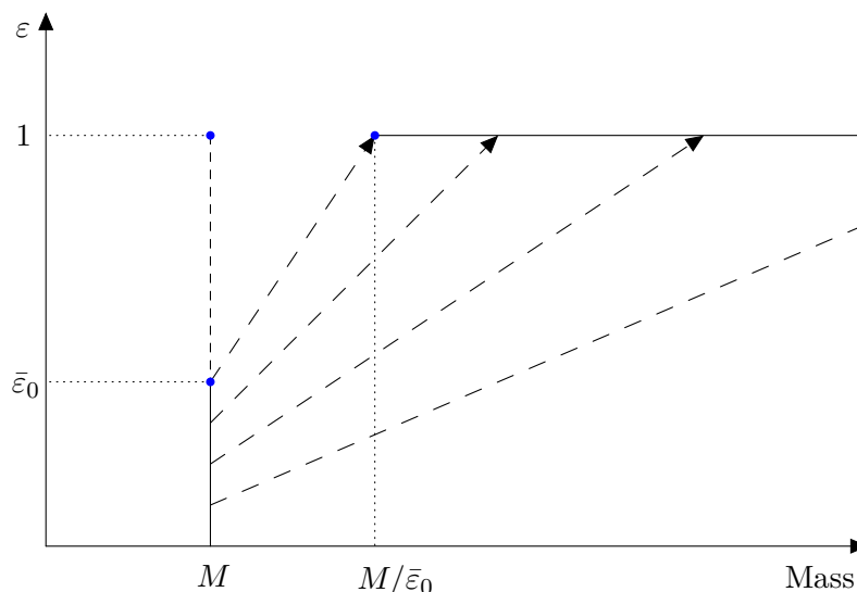
Figure 4.2: Illustration of the strategy: for the given mass M , the stability of the ground states is proved for the potentials \Sigma^\varepsilon , with 0 \leq \varepsilon < \bar{\varepsilon}_0 . By rescaling, we can go back to the potentials \Sigma^1 , and ground states with a mass larger than M/\bar{\varepsilon}_0 are stable.
