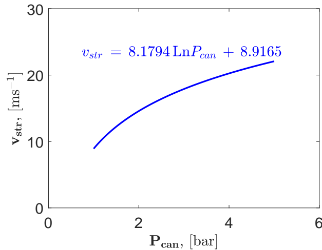
Figure 2.4 – P_{can} vs v_{str} for long striker (Pavier, 2013)
