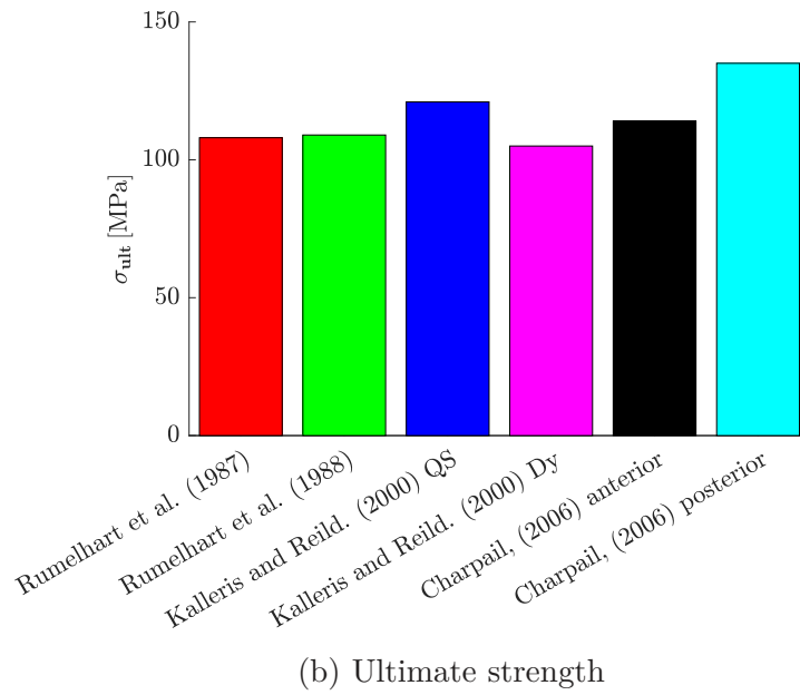
Figure 1.16 – Compressive properties of cylindrical human rib samples
