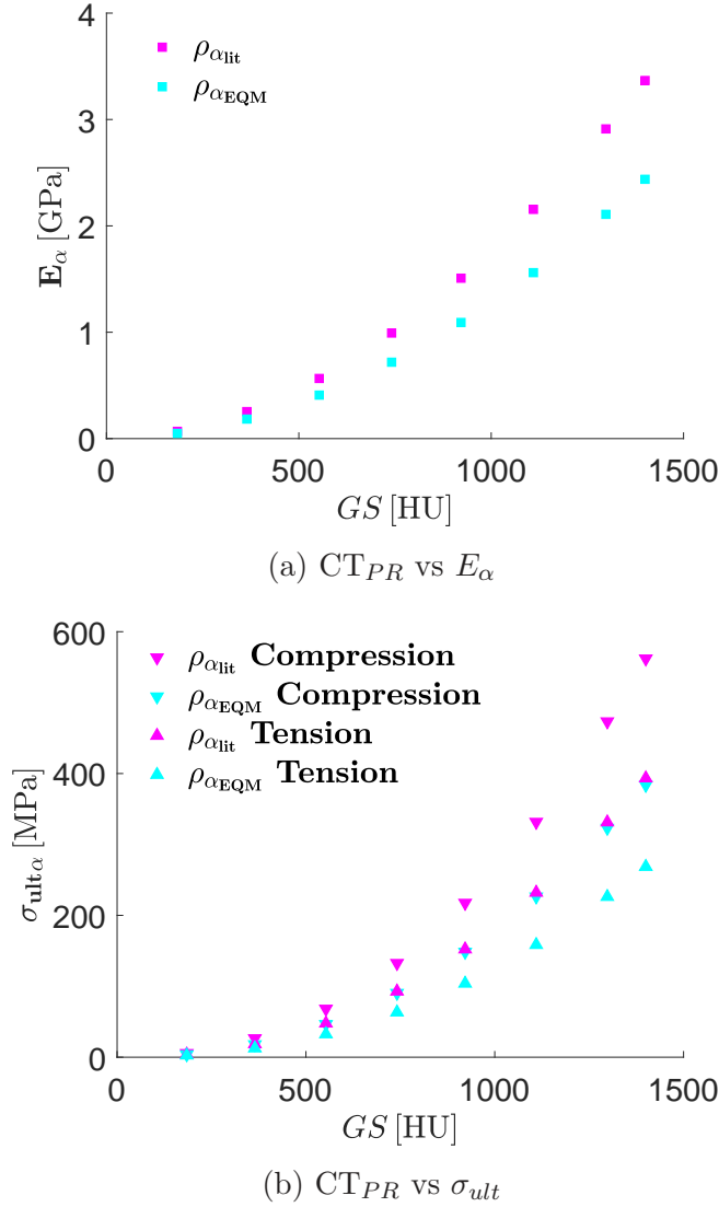
Figure 3.8 – Mechanical properties of porcine rib with \rho_\alpha
