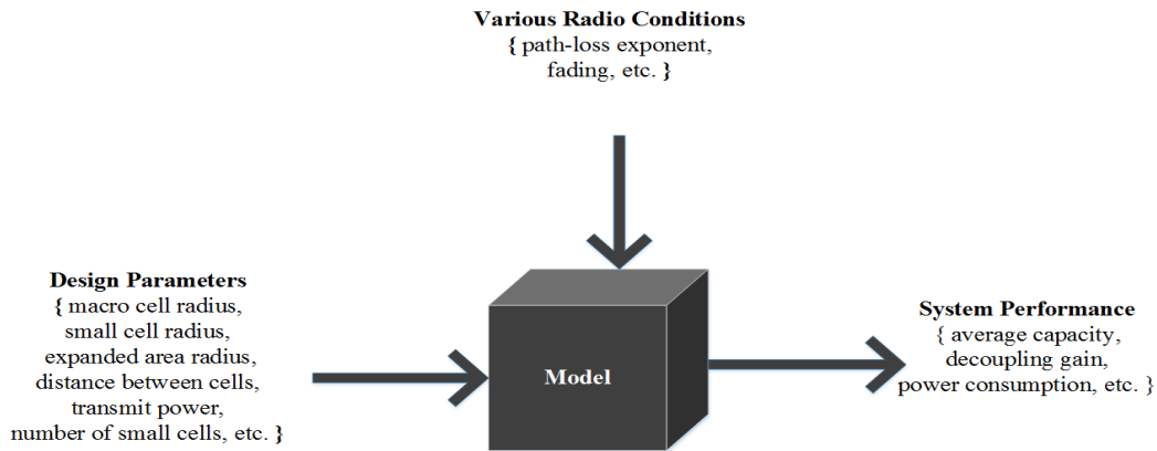
Figure 3.5: Model overview.
