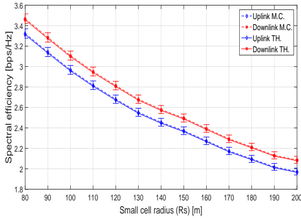
Figure 4.4: Capacity per unit bandwidth in the reference small cell as a function of small cell radius ( R_s ) with N_s = 1 , \gamma = 3 and d = 600 m.
