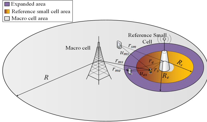
Figure 3.8: Geometrical illustration of the network model - with decoupling.
