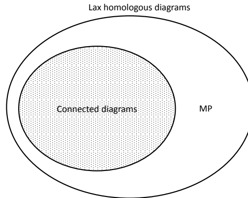
Figure 6.2 – The Multiplicity Principle happens exactly when two diagrams are lax homologous but not connected. Thus, the MP is the complement of Lemma 6.2.8.
