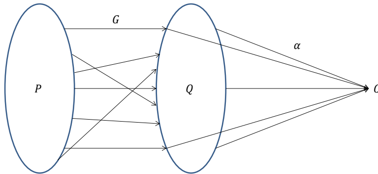
Figure 6.1 – Note that such a composition yields a cocone: a cocone Q \rightarrow \Delta(C) composed with a cluster P \rightarrow Q yields a cocone P \rightarrow \Delta(C) .
