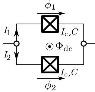
Figure 1.4 – Schematic of a symmetric SQUID. Two identical Josephson junctions are in parallel in a superconducting loop. The loop is threaded with an external DC magnetic flux \Phi_{\text{dc}} .
