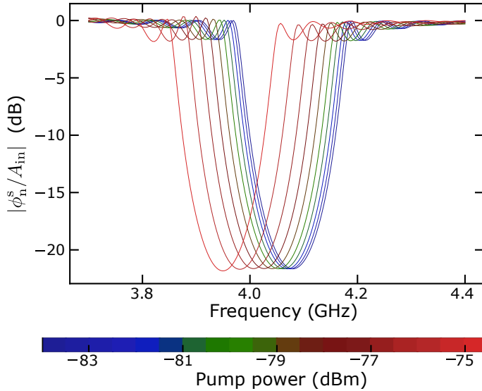
Figure 3.15 – Expected cross phase modulation of the photonic gap. Signal transmission as a function of its frequency. Color encodes the pump input power P_{\text{in}} . Pump frequency is fixed at \omega_p = 2.0 GHz. P_{\text{in}} shifts the gap position and drag it to lower frequencies as it was experimentally shown in Fig. 3.9. Between the blue and red transmission, the gap shifts more than its own width.
