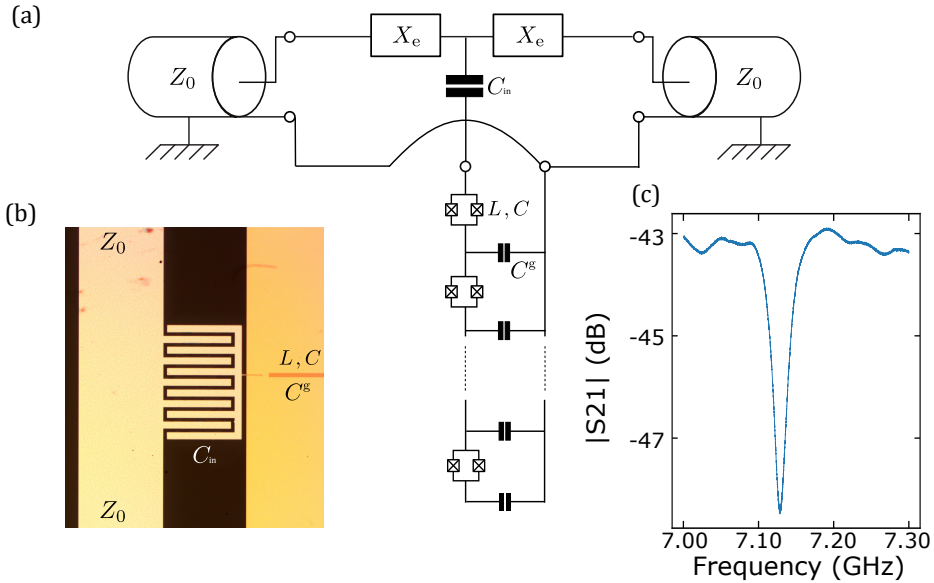
Figure 6.4 – Hanger \lambda/2 resonator with a top ground geometry. (a) Electrical circuit of the S-Res. SQUIDs are characterized by L , C^g and C . The S-Res is coupled to a Z_0 = 50 \Omega transmission line via a capacitance denoted C_{in} . The wire bonds reactance is denoted X_e . (b) Picture taken with an optical microscope: on the left side the Z_0 impedance transmission line in coplanar waveguide geometry, in the center the interdigital capacitance, and on the right the 600 SQUID long resonator covered by a 400 nm gold sheet. (c) Transmission measured with the VNA close to a resonance. Fit of such resonance allows to extract quality factors (internal and external).
