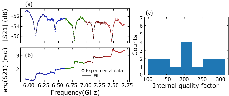
Figure 6.5 – Extraction of the quality factors. (a)-(b) Experimental scattering parameter S_{21} (amplitude (a) and phase (b)) of the S-Res and their fit close to resonances between 6 GHz and 7.75 GHz. (c) Counts of internal quality factors extracted from the fit of 14 modes as in panel (a) between 3.8 GHz and 8.46 GHz at input power P_s = -136 \text{ dBm} \pm 3 \text{ dBm} , corresponding to the single-photon level. We observe a spread of the internal quality factor of around 200 at this power.
