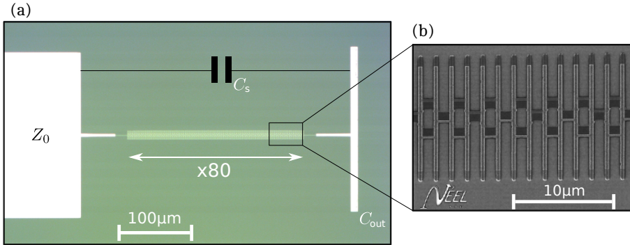
Figure 6.1 – \lambda/4 resonator. (a) Optical microscope picture. The left-most pad is the bonding pad, the right-most thin pad is the shunt capacitance denoted C_{out} . In between, there is the array of 80 SQUIDs. (b) Scanning electron microscope (SEM) picture of seven SQUIDs where a single junction has a 10.7 \mu\text{m} \times 0.37 \mu\text{m} area.
