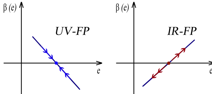
Figure 1.5: A general example of the UV stable fixed point (on the left) and the IR stable fixed point (on the right) for a beta function \beta(e) .
