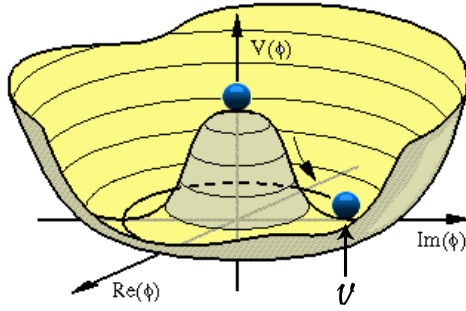
Figure 5.1: The Higgs ("Mexican hat") potential. A small perturbation transfers the system from the higher energy symmetric local maximum ( v = 0 , \phi_0 = 0 ) to the lower energy asymmetric local minimum ( v = \frac{|\mu^2|}{\lambda} , \phi_0 = \pm \frac{v}{\sqrt{2}} ).
