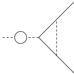
Figure 2.1: The two-loop diagram corresponding to the term -4\kappa Y_2^{ac} Y^b Y^{+c} Y^b which should not contribute to the \beta -function for the Yukawa couplings.
