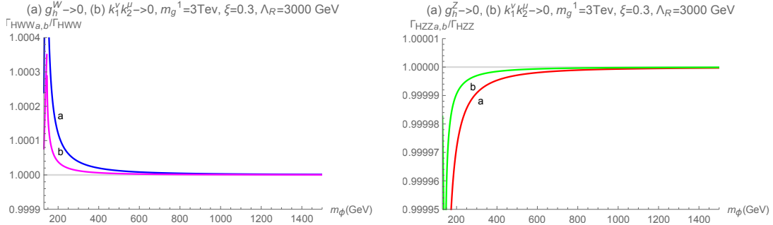
Figure 7.1: Ratio of the width without the contribution -2g_h^{W,Z} (\eta^{\mu\nu} p_1 \cdot p_2 - p_1^\nu p_2^\mu) (a) and without the contribution 2g_h^{W,Z} p_1^\nu p_2^\mu (b) to the full widths expression, for the processes H \rightarrow WW (on the left) and H \rightarrow ZZ (on the right). As we can see, for all cases this ratio is very close to 1.
