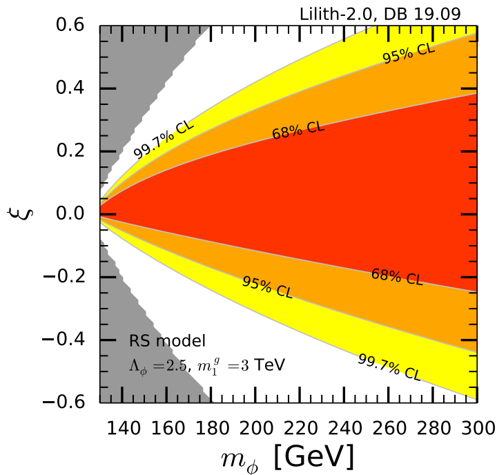
Figure 7.2: Constraints on the radion mass and parameter \xi in the (\xi, m_\phi) plane for \Lambda_\phi = 2.5 \text{ TeV} and m_1^g = 3 \text{ TeV} . The red, orange and yellow filled surfaces correspond to the allowed 68%, 95% and 99.7% CL regions, respectively.
