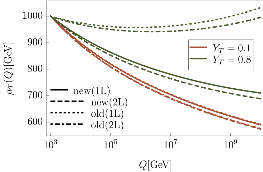
Figure 3.2: The running mass \mu_T of the vector-like top partners at one- and two-loop level for two different choices of the Yukawa coupling Y_T . Here, we show the results using the incorrect ('old') expressions in literature as well as our derived expressions ('new'). The other parameters are set to \lambda_{HS} = 0 , \lambda_S = 1 , \kappa_{HS} = \kappa = 1 TeV.
