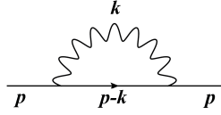
Figure 1.1: 1-loop electron self energy -i\Sigma(p, m) .
