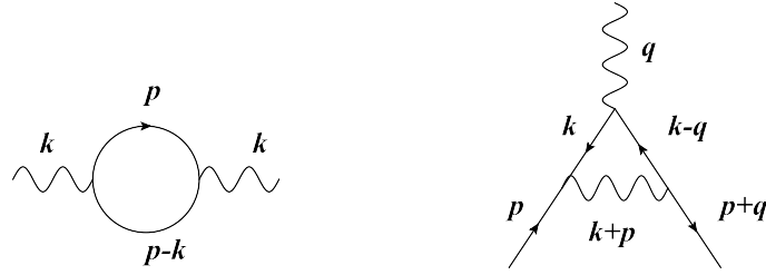
Figure 1.4: Vacuum polarization \Pi_{\mu\nu} (left) and vertex correction \Lambda_\mu (right) diagrams at one-loop.
