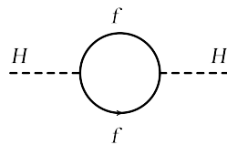
Figure 5.3: One-loop correction to the Higgs squared mass parameter m_h^2 with a massive fermion loop.
