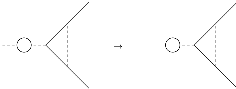
Figure 3.1: Two-loop diagram which does not contribute to the \beta -function for the Yukawa couplings (on the left) and, consequently, for the fermion mass when replacing the external scalar by a dummy field (on the right). A (non-zero) contribution corresponding to the tadpole diagram on the right hand side was included in Ref. [12]. It should be replaced by (A.3).
