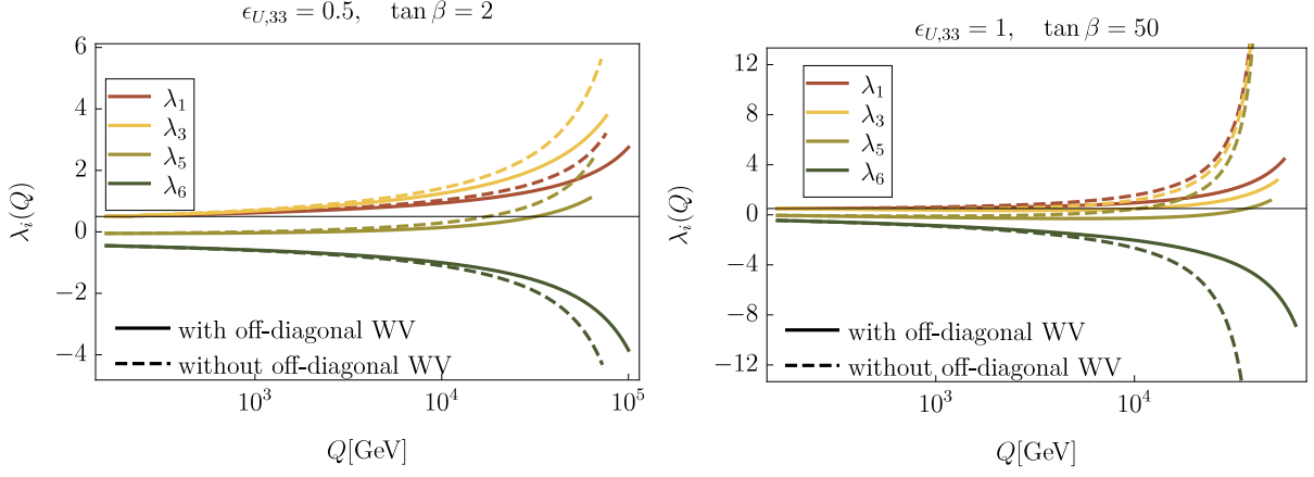
Figure 3.3: The running of different quartic couplings in the THDM-III with and without the contributions of off-diagonal wave-function renormalization to the \beta -functions of the quartic couplings. Here, we have used the input parameters \lambda_1 = \lambda_3 = \lambda_4 = 0.5 , \lambda_5 = -0.05 , \lambda_6 = \lambda_7 = -0.45 , \tan \beta = 2 and M_{12} = 500^2 GeV ^2 at Q = m_t . On the left, we have used \epsilon_{U,33} = 0.5 , \lambda_2 = 0.5 , \tan \beta = 2 , and on the right \epsilon_{U,33} = 1 , \lambda_2 = 0.15 , \tan \beta = 50 . All other \epsilon_i are zero.
