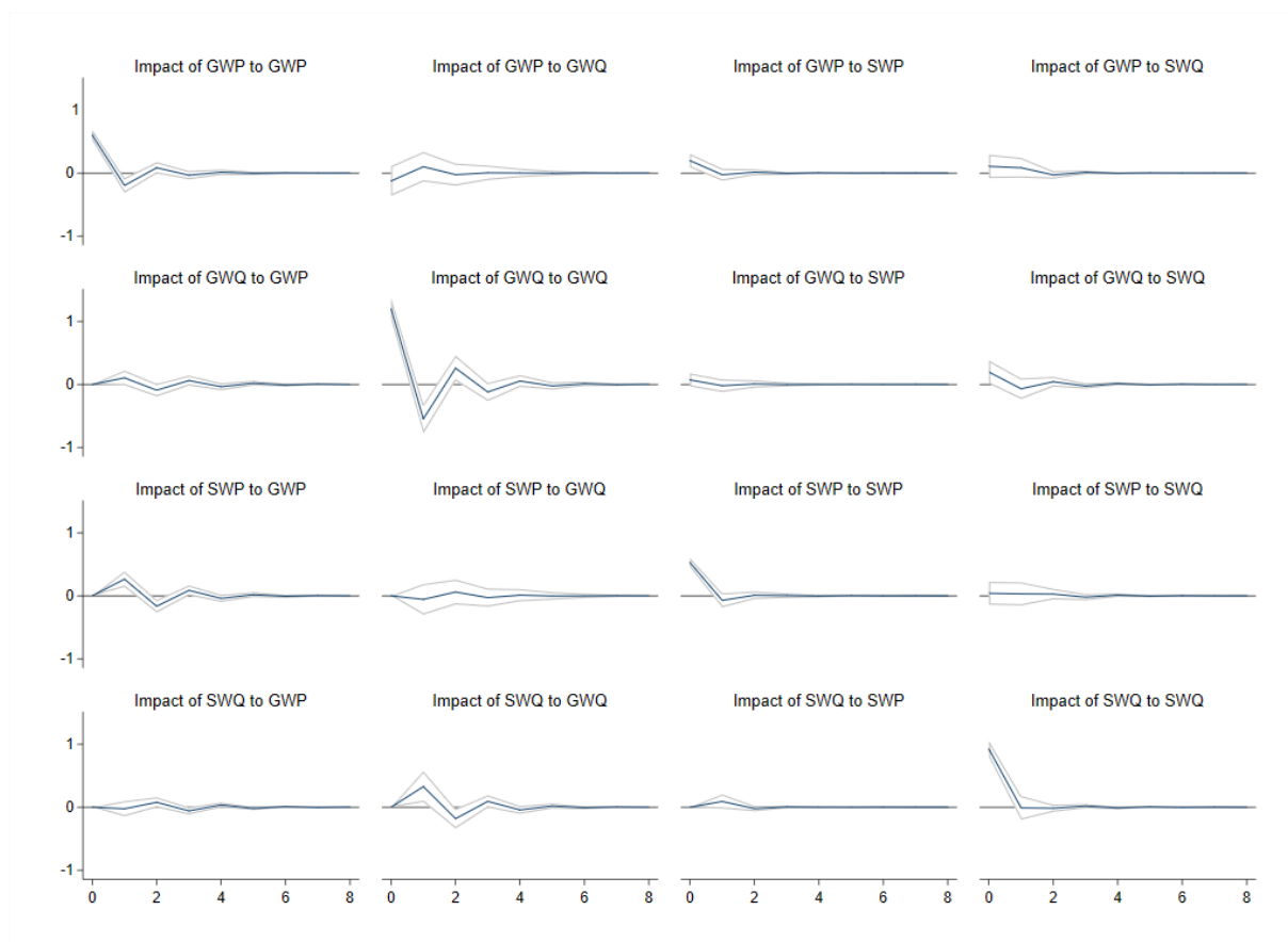
Figure B1: Orthogonalized Impulse-Response Functions and 5% confidence interval following the VARX(1) estimation in the Murrumbidgee temporary surface and groundwater markets, 2008-2018
