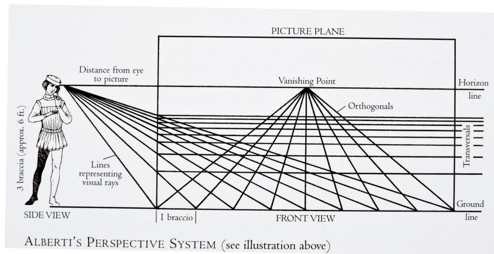
Figure 17.2: One-point linear perspective with horizon
