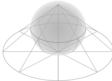
Figure 17.1: Stereographic projection of a sphere
