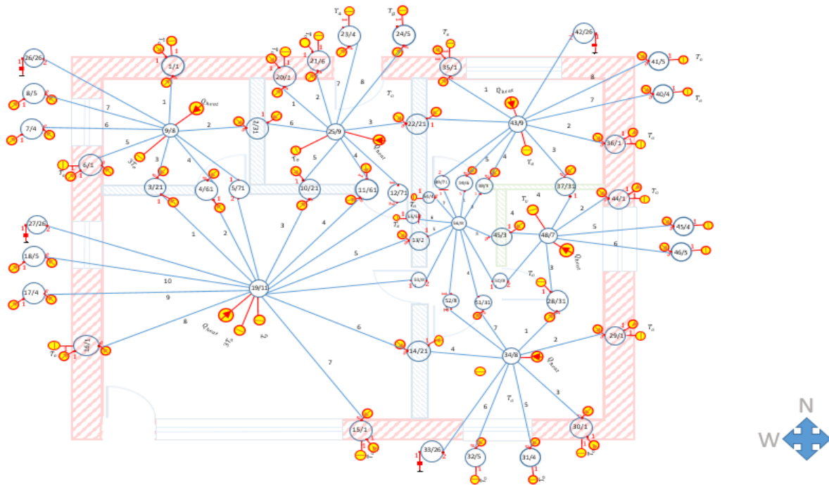
Figure 6.11: Thermal circuit diagram for all zones of twin house
