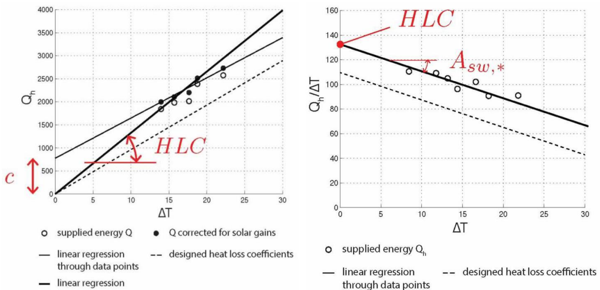
Figure 3.6: Estimation of H and Solar aperture, using simple linear regression [46]
