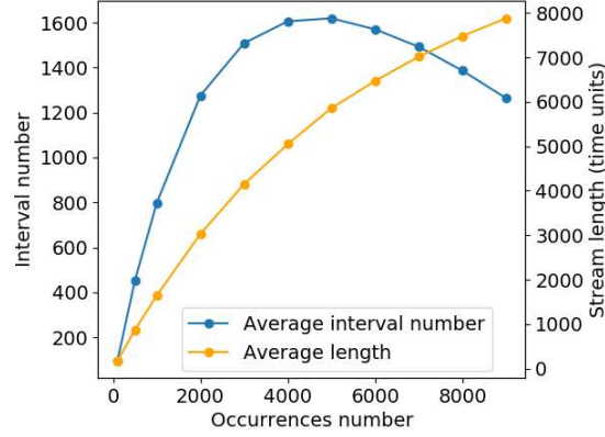
Figure 8.3.3: Average stream length and interval number with respect to occurrence number in the Linear trajectory datasets described in Table 8.3.1
