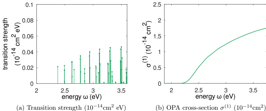
Figure 5.3.3: Transition strength and one-photon absorption cross-section versus photon energy \omega (eV) at HF level for edge length L = 9.0 nm. The calculations were done by using the parameter set 1. For the broadening of the transition lines, \Delta E_0 = 0.1 eV and \Delta L/L = 12\% .
