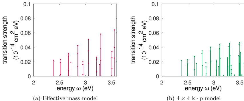
Figure 5.4.10: Transition strength at HF level versus transition energy \omega for CsPbBr 3 of edge length L = 9.0 nm in the effective mass model (left) and 4 \times 4 k · p model (right). The basic parameters are from parameter set 1. Note the higher density of the transitions in the case of 4 \times 4 k · p model.
