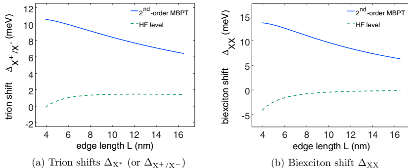
Figure 4.3.4: The calculated biexciton and trion shifts versus edge length L for \text{CsPbBr}_3 . Dashed green line: HF level, solid blue line: second-order MBPT. The dashed lines show that the biexciton or trion shifts equal to almost zero at HF level, which remains true for any mean-field method [113]. The nonzero \Delta_{\text{X}^*} and \Delta_{\text{XX}} are essentially the result of correlation energy.
