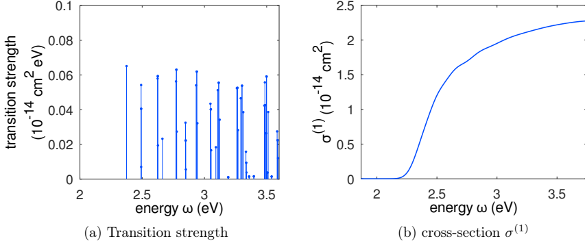
Figure 5.4.8: Transition strength and cross-section \sigma^{(1)} versus transition energy \omega for CsPbBr 3 nanocrystal with edge length L = 9.0 nm in the 4 \times 4 k-p model. The calculations were done at HF level plus first-order vertex correction with \delta E_{\min} = 20 meV. The basic parameters are given in parameter set 1.
