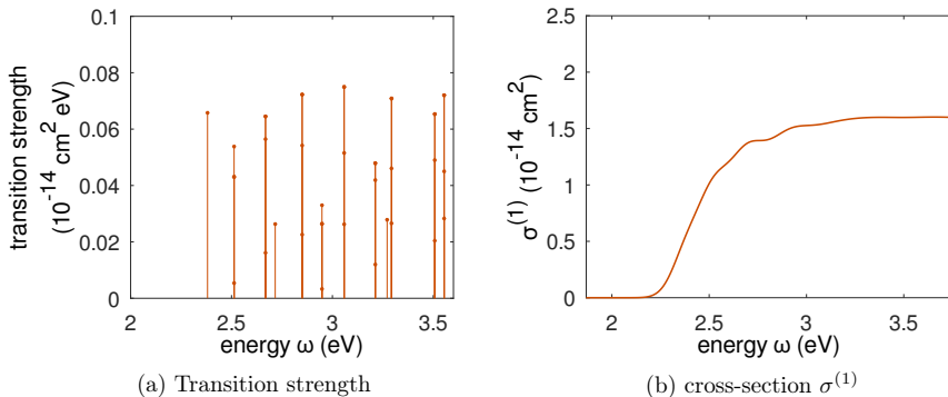
Figure 5.4.9: Transition strength and cross-section \sigma^{(1)} versus transition energy \omega for CsPbBr 3 nanocrystal with edge length L = 9.0 nm in the effective mass model. The basic parameters are given in parameter set 1, except there is no \text{k} \cdot \text{p} coupling between the conduction and valence bands by setting E_p = 0.0 eV. The energy lower bound for vertex correction is \delta E_{\text{min}} = 20 meV.
