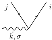
Figure 5.1.2: The electron-photon interaction vertex.
