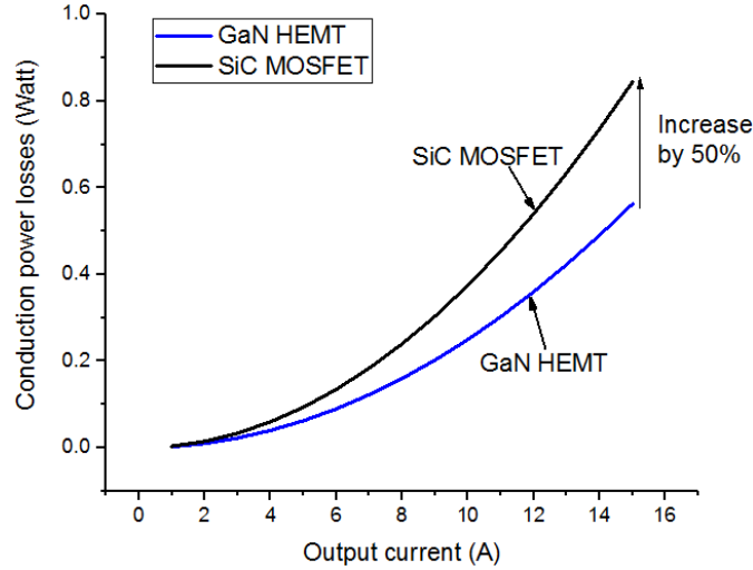
Fig. 2.13: Simulated conduction power losses comparison between GaN HEMT (GS66508P), SiC MOSFET (SCT2120AF).
