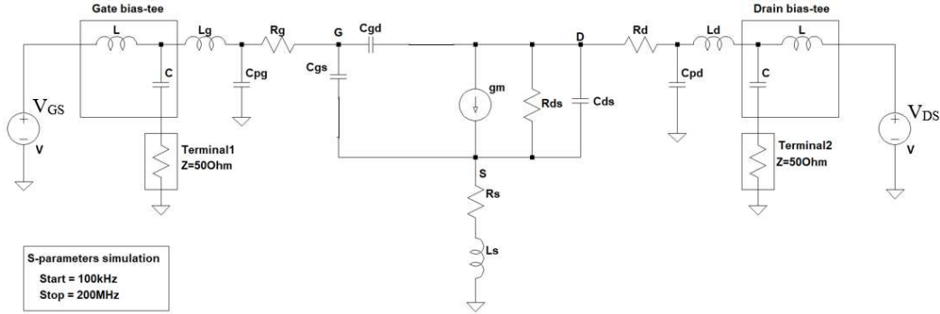
Fig. 4.19: S-parameter simulation setup at Q P4 bias point.
