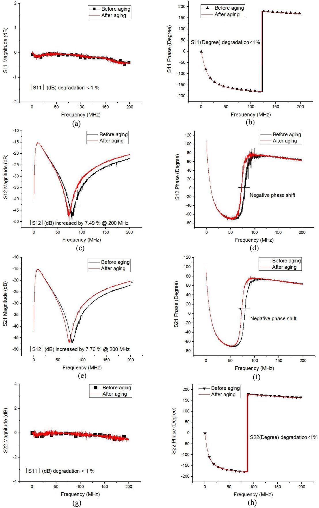
Fig. 5.9: Evolution of the S parameters during 720 h of aging: (a) S_{11} Magnitude, (b) S_{11} Phase, (c) S_{12} Magnitude, (d) S_{12} Phase, (e) S_{21} Magnitude, (f) S_{21} Phase, (g) S_{22} Magnitude, (h) S_{22} Phase.
