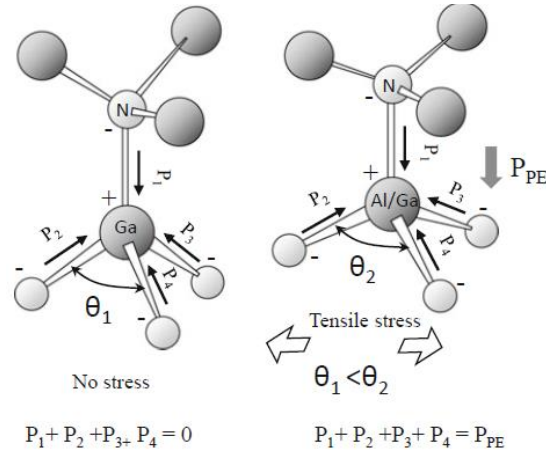
Fig. 2.23: Generation of the GaN piezoelectric polarization [36].
