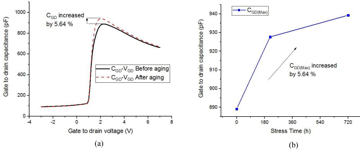
Fig. 5.6: (a) Evolution of C_{GD}-V_{GD} characteristic before and after aging; (b) Evolution of C_{GD(Max)} during aging.
