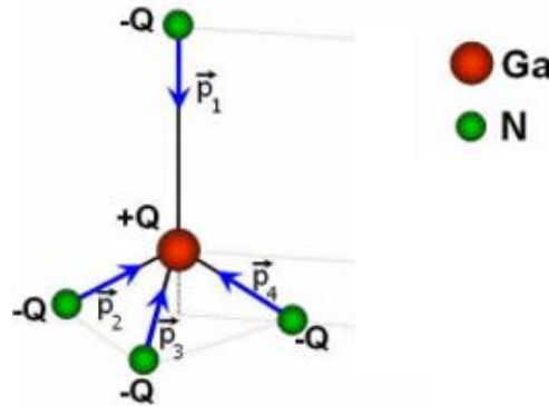
Fig. 2.22: Generation of the GaN spontaneous polarization [35].
