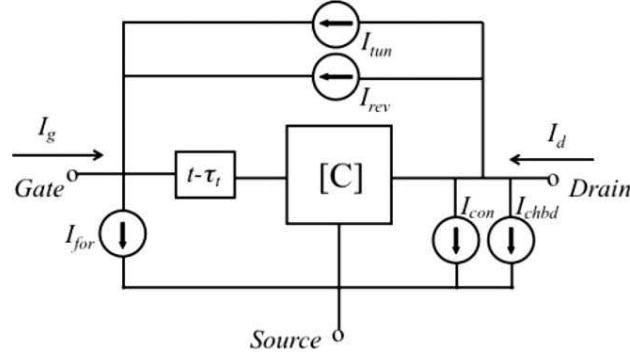
Fig. 2.31: Compact physical GaN HEMT model [94].
