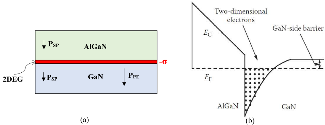
Fig. 2.24: AlGaIn/GaN heterostructure: (a) cross section (b) Band diagram [37].
