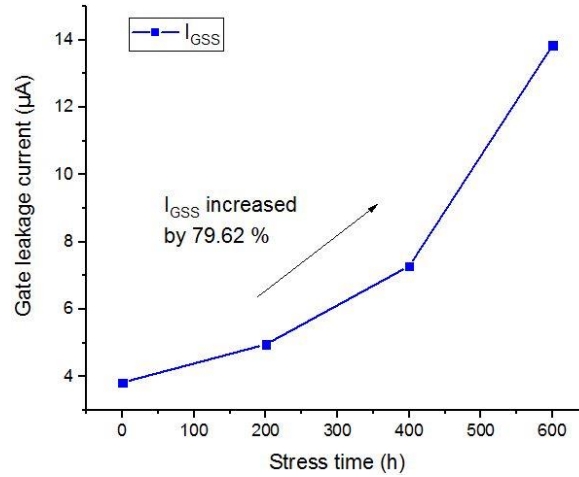
Fig. 5.12: Evolution of I_{GSS} current at V_{GS} = 6 V during on-state stress.
