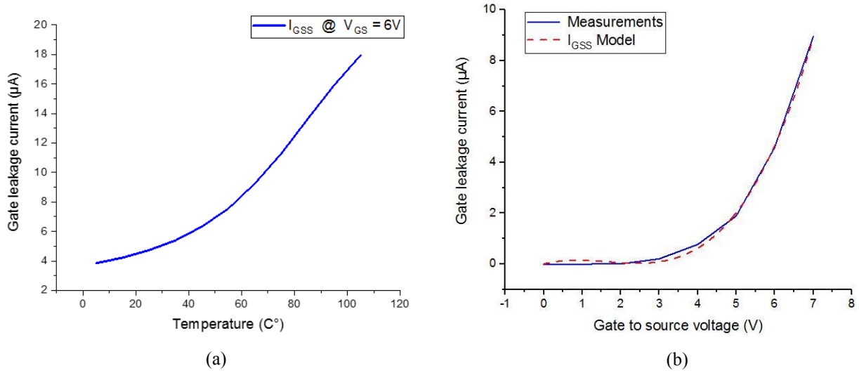
Fig. 3.30: Gate leakage current: (a) temperature dependency at V_{GS} = 6V ; (b) I_{GSS} Model as a function of V_{GS} at 25 °C.
