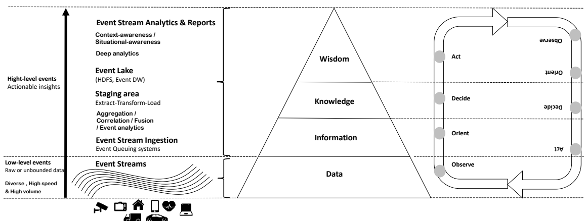
Figure 1.13 – Event Stream Processing Chain
