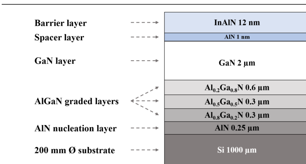
Figure 29: Schematic of HEMT growth structures.
