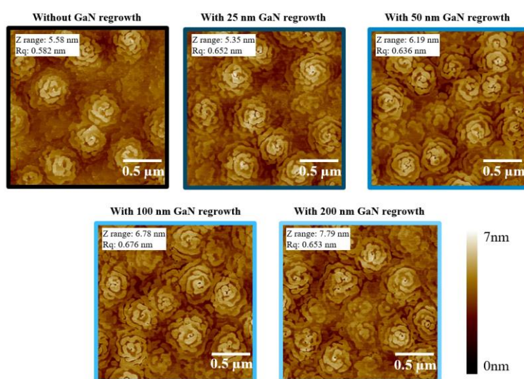
Figure 80: 2 \mu m x 2 \mu m AFM scans of set C.
