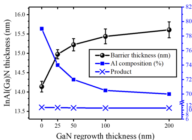
Figure 54: Barrier thickness measured by XRR (black line), Al composition in barrier (blue line/□) and the product (blue line/X): versus GaN regrowth thickness.
