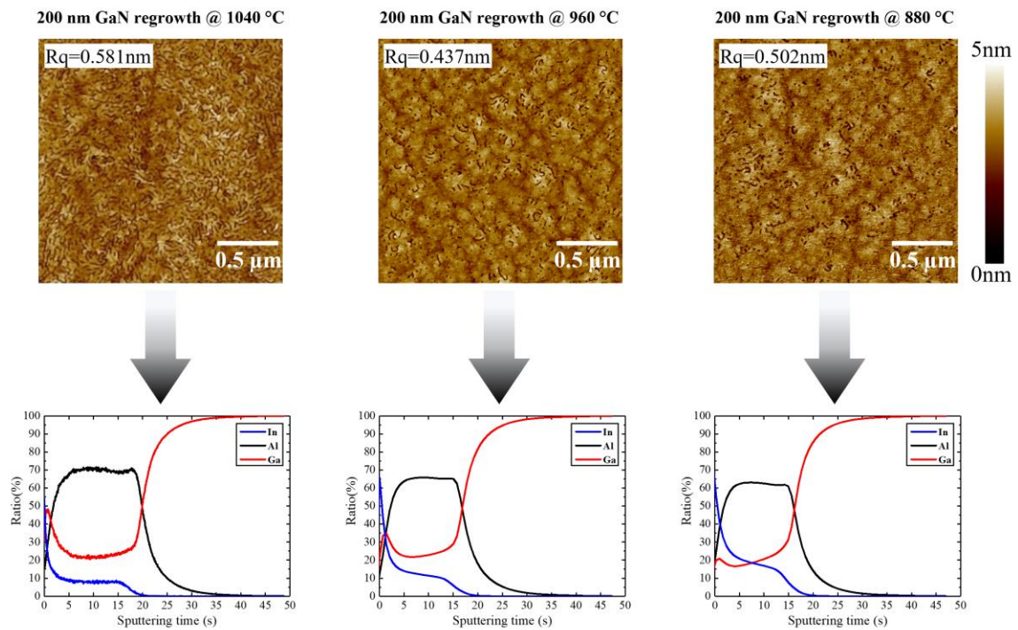
Figure 105: 2\mu\text{m} \times 2\mu\text{m} AFM scans with PP-TOFMS measurements of the 1040 °C, 960 °C and 880 °C GaN regrowth samples.
