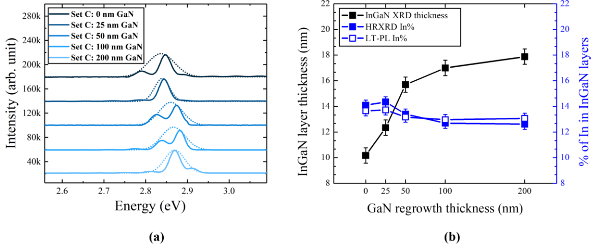
Figure 81: (a) LT-PL spectra: InGaN normalized intensity as function of photon energy at 6K (solid lines) and the fitted data (dash lines). (b) InGaN layer thickness and In% in InGaN layers as deduced from XRD and LT-PL.
