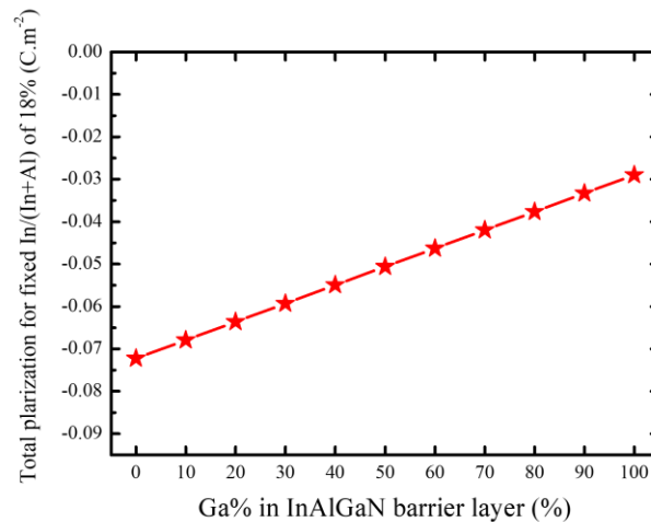
Figure 11: Total polarization in InAlGaIn barriers for increased Ga% and fixed In/(In+Al) ratio of 18%.
