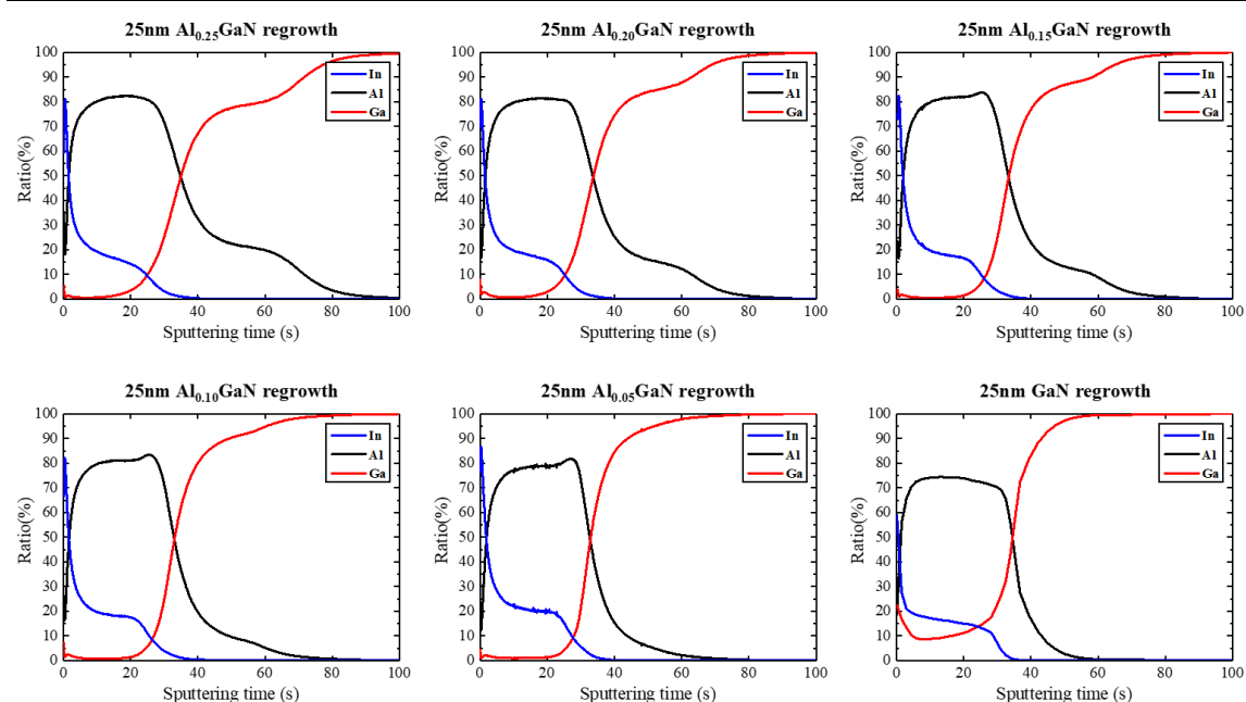
Figure 91: PP-TOFMS measurements for samples grown with 25 nm of AlGaIn with different Al% and GaN.
