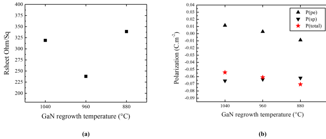
Figure 106: (a) R_{sheet} measurements and (b) calculated barrier polarizations of the 1040 ^{\circ}\text{C} , 960 ^{\circ}\text{C} and 880 ^{\circ}\text{C} GaN regrowth samples.
