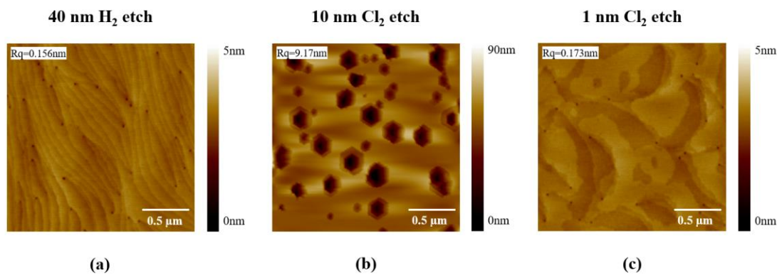
Figure 62: 2\mu\text{m} \times 2\mu\text{m} AFM scans showing GaN surface morphology after performing (a) 40 nm \text{H}_2 etch, (b) 10 nm \text{Cl}_2 etch and (c) 1 nm \text{Cl}_2 etch.
