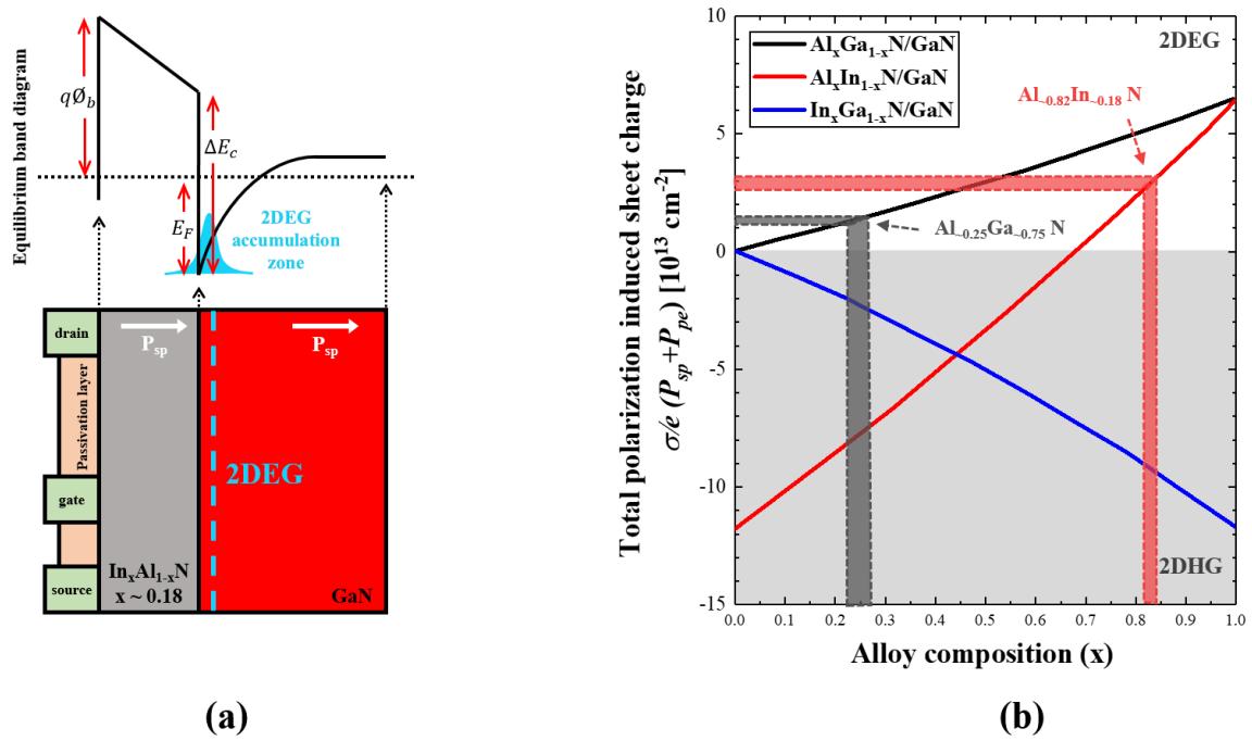
Figure 6: a) III-N HEMT heterostructure, with the equilibrium band diagram ( V = 0 Volts) of the InAlN/GaN heterostructure above b) total polarization induced sheet charge \sigma/e (P_{sp} + P_{pe}) bound at the interfaces of Ga-face AlGaN/GaN, AlInN/GaN and InGaN/GaN heterostructures, versus alloy composition of the top layer [38].
