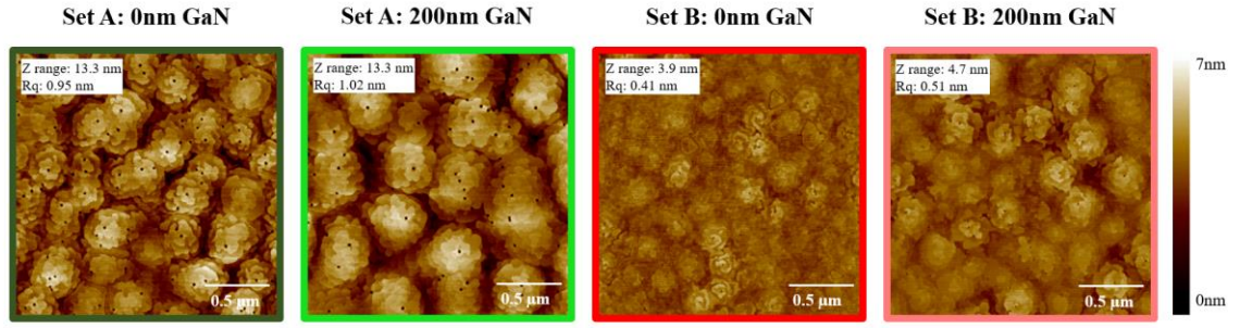
Figure 75: 2\mu\text{m} \times 2\mu\text{m} AFM scans of set A (TMGa as Ga source) and B (TEGa as Ga source).
