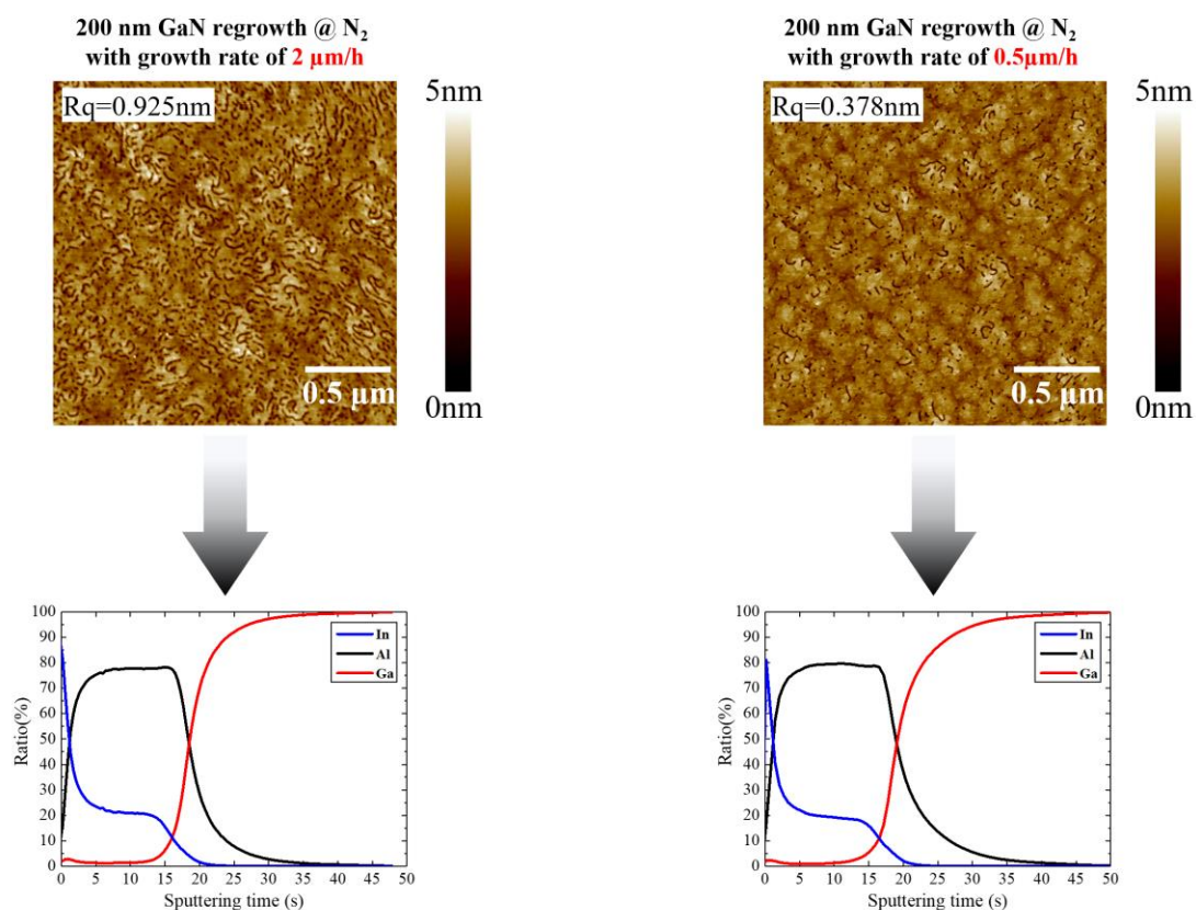
Figure 110: 2 \mu\text{m} \times 2 \mu\text{m} AFM scans with PP-TOFMS measurements for the 200 nm GaN regrowth samples under N_2 with different growth rates.
