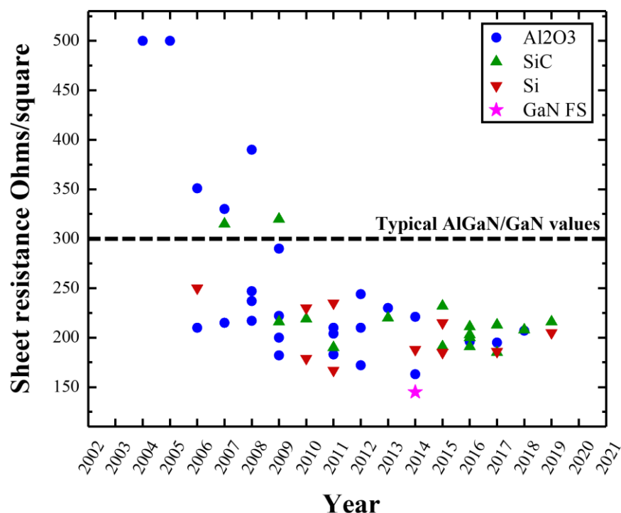
Figure 10: InAlN/GaN sheet resistance values for different substrates in function of years of development, and black dashed line present typical AlGaIn/ GaN R_{\text{sheet}} values. [64, 65, 66, 67, 68, 69, 70, 71, 72, 73] [74, 75, 76, 77, 78, 79, 80, 81, 82, 83] [84, 85, 86, 87, 88, 62, 89, 90, 91, 92] [93, 94, 95, 63, 96, 60, 97, 98, 99, 100] [101, 102, 103, 104, 105, 106, 61, 107, 108, 109] [110, 111, 112]
