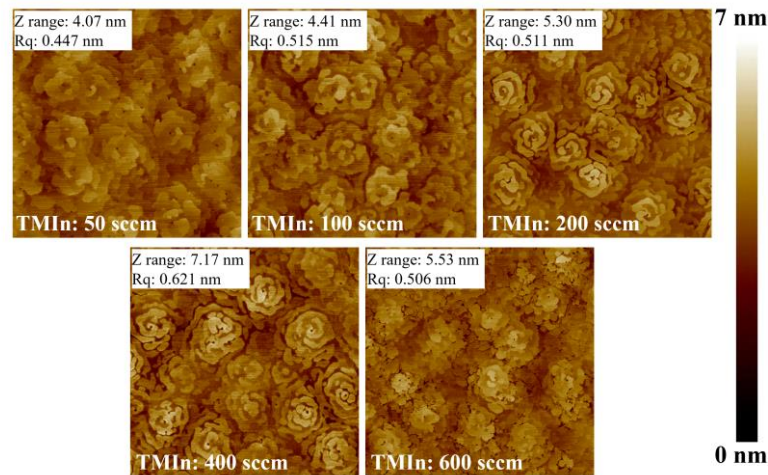
Figure 84: 2\mu\text{m} \times 2\mu\text{m} AFM scans of samples grown in cleaned reactor of set D and one sample of set C (TMIn: 400 sccm).
