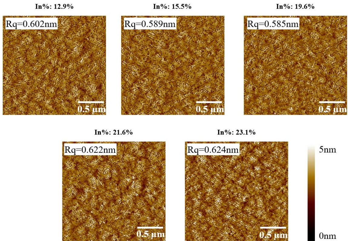
Figure 68: 2μm x 2μm AFM scans of all InAlN barrier layers with different In%.
