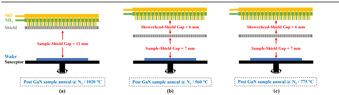
Figure 93: Diagram showing growth chamber during the nitridation step for sample (a), (b) and (c).
