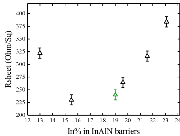
Figure 69: R_{sheet} measurements of the 5 InAlN samples grown onto 5nm H_2 etched GaN templates with different In% (in black) and in green the first 5 nm H_2 etched sample that we have shown in Figure 63 (b).
