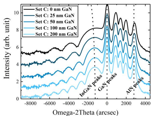
Figure 78: (0002) XRD \omega -2 \theta measurements of set C.
