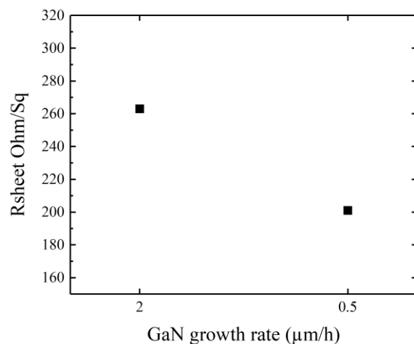
Figure 111: R_{\text{sheet}} measurements for the 200 nm GaN regrowth samples under N_2 with different growth rates.
