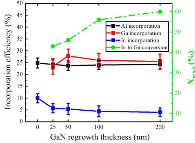
Figure 58: Incorporation rates for Al, Ga and In and X_{\text{react}} . X_{\text{react}} is calculated for a fixed In incorporation rate of 10%.
