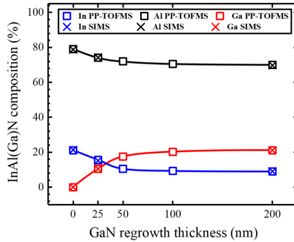
Figure 52: InAl(Ga)N barriers composition of as a function of regrown GaN thickness.
