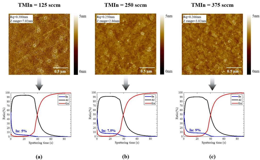
Figure 70: 2μm x 2μm AFM scans with PP-TOFMS measurements of InAlN/AlN/GaN heterostructures with different TMIn growth flows.
