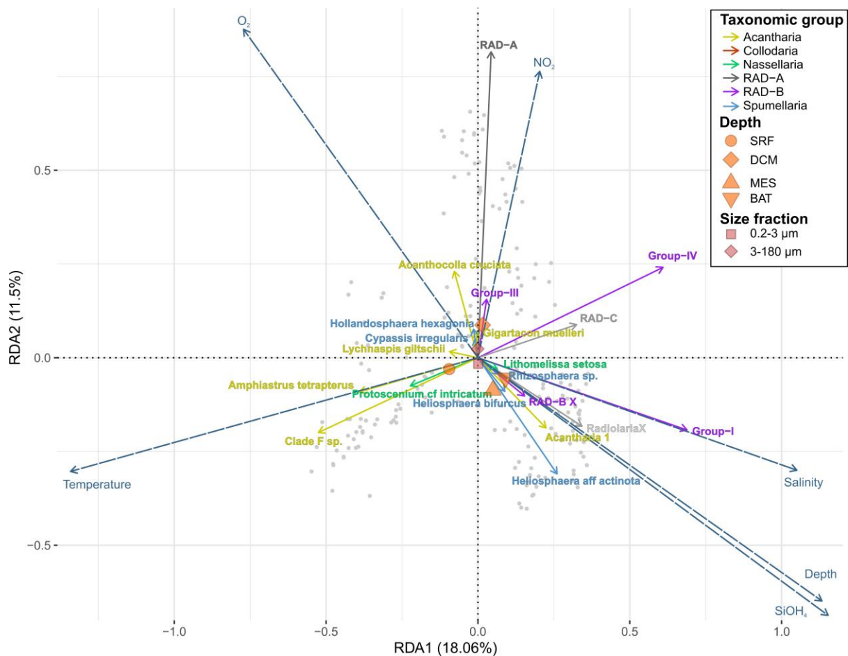
Figure 5. Redundancy analysis (RDA) triplot showing the impact of environmental variables on the distribution of the 41 Esoufier-selected taxa (only most relevant shown) for MOOSE-GE expedition on the samples collected by Niskin Bottle. The adjusted R-squared of the analysis is of 42.15% (46.94% unadjusted).
