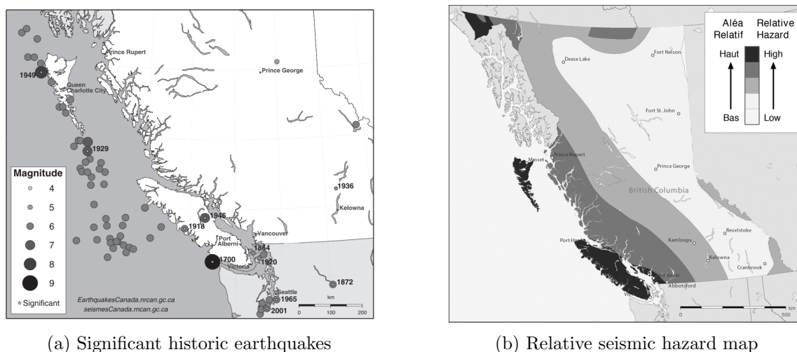
Figure 1.1: Seismic hazard in British Columbia (B.C.) (Earthquakes Canada, 2020)
