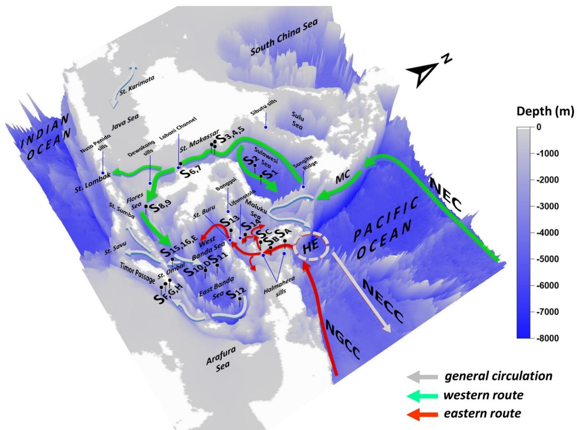
Figure 3.1 Schematic of the general circulation in the Indonesian seas and its surrounding waters with basins and some restricted features (straits, channel, and sills) toponymal on the topography provided by ETOPO; the locations of repeated profiling CTD casts (black pins, S_1 - S_{16} ) and VMP stations (black pins, S_A - S_H ). The North Pacific water masses flow in the Indonesian seas through the western route of ITF (green arrows), which is forced by the north equatorial current (NEC) that bifurcates southward as Mindanao Current (MC). The South Pacific water masses flow in the Indonesian seas through the eastern route (red arrows), which is forced by New Guinea coastal current (NGCC) originating at the bifurcated current of the Halmahera eddy (HE) and the north equatorial counter current (NECC).
