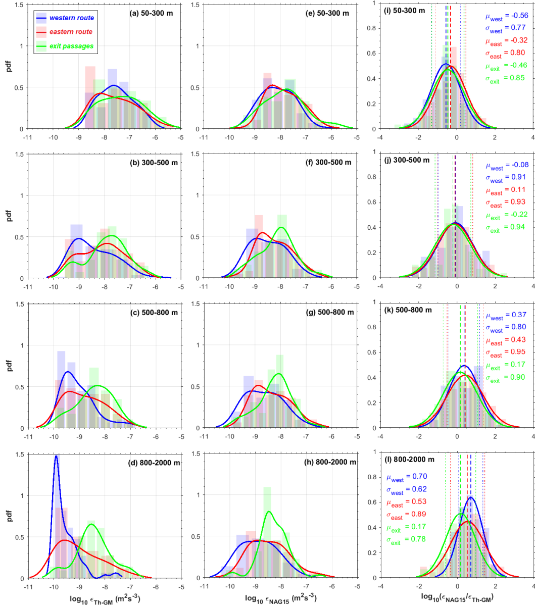
Figure 3.11 PDF histogram of the dissipation rate from historical data set, \epsilon_{Th-GM} (a, b, c, d) and those from NAG15 model, \epsilon_{NAG15} (e, f, g, h), inferred from the spatially gridded cells of the historical data sets for four depth ranges, plotted with the number of bin based on the Freedman-Diaconis rule, with respected kernel distribution estimates. The western route (SLA, MAK, FLO), eastern route (MAL, HAL, BAN) and exit passages (LES) regions are presented in blue, red and green colors, respectively. The PDF histogram ratio of the model to the observed dissipation rate, \epsilon_{Th-GM} with respected normal distribution fits is displayed in (i, j, k, l). The mean and standard deviation are also indicated with dashed and dotted lines, respectively. Note that, only the dissipations of the model at the grid cells where the observation grid cells exist are taken into account.
