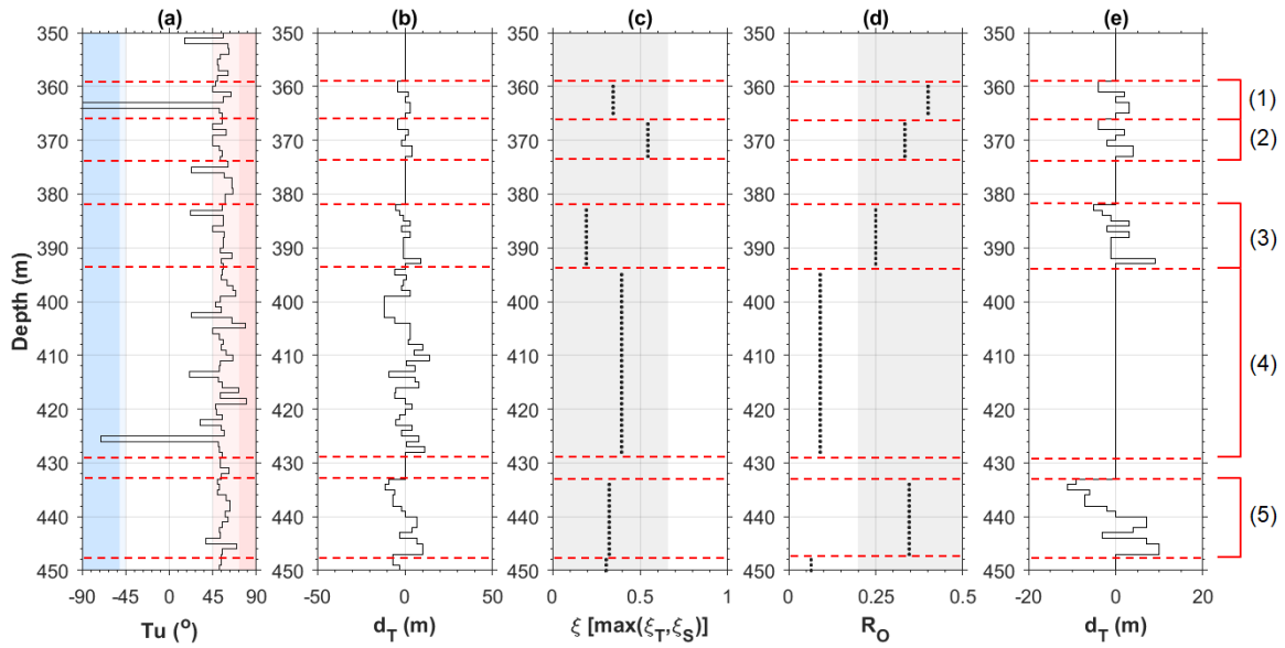
Figure 3.18 An example of overturn selection criterion applied in this study: (a) vertical profile of Turner angle with shaded regions of strong ( -90^{\circ} \leq Tu \leq -51^{\circ} ) and weak diffusive convection ( -51^{\circ} \leq Tu \leq -45^{\circ} ) potential (dark and light blue, respectively); strong ( 72^{\circ} \leq Tu \leq 90^{\circ} ) and light salt fingering ( 45^{\circ} \leq Tu \leq 72^{\circ} ) potential (dark and light red, respectively). (b) Observed vertical displacements, (c) T/S tightness test with \xi < 0.66 threshold (gray shaded region), (d) overturn ratio criteria with R_o > 0.2 thresholds (gray shaded region). (e) Remaining overturn considered as turbulent event. The types of turbulent according to Tu criterion give: (1) turbulence occurrence in double diffusive favorable conditions, (2, 3, 5) turbulent within salt fingering favorable condition and (4) spurious turbulent.
