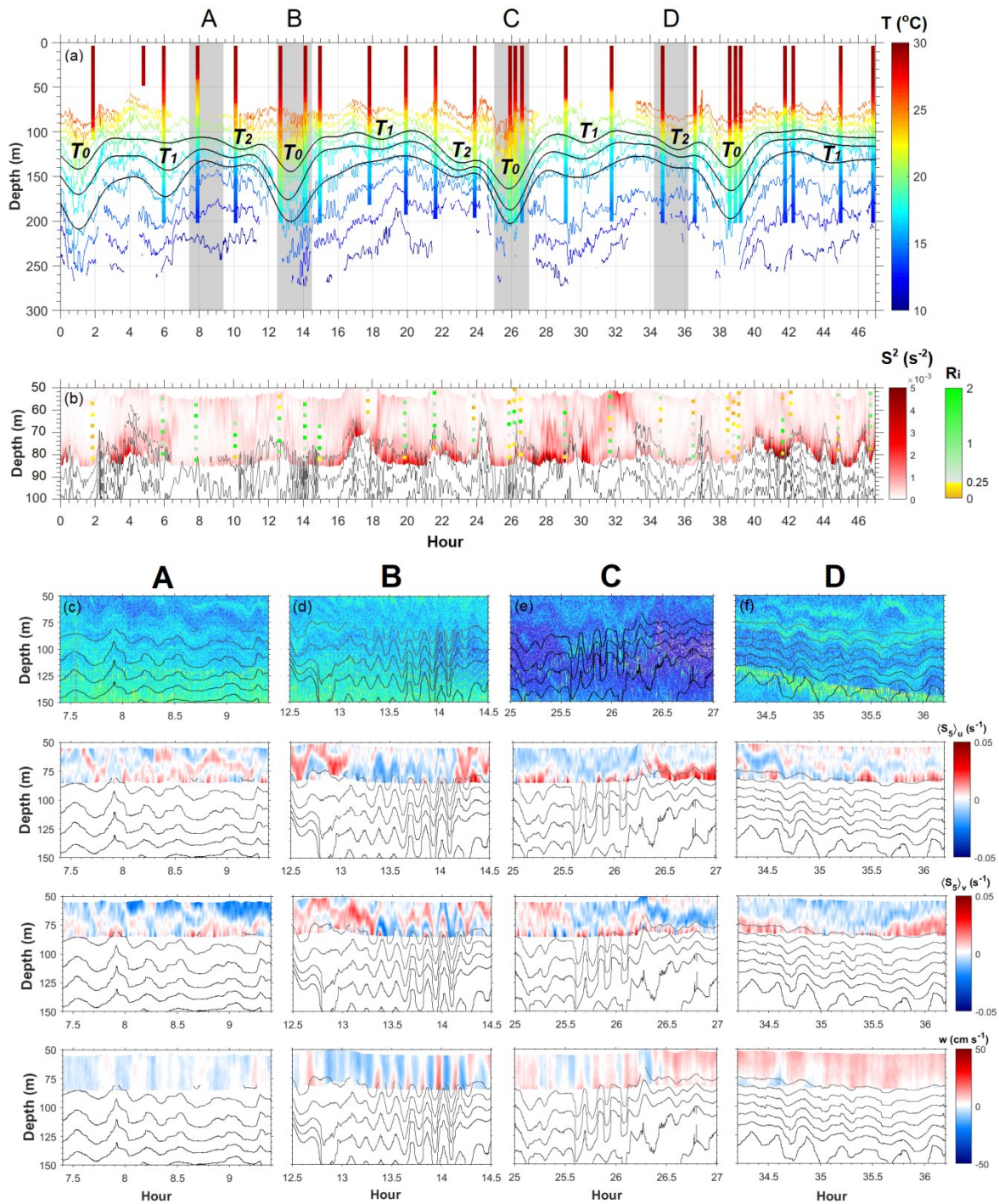
Figure 5.6 (a) Isotherm contours inferred from RBR sensors and temperature profiles from CTD casts. The black line is M2 low pass filtered for isotherm 18, 20, and 22°C. (b) is squared shear superimposed isotherms and Richardson number, Ri . (c, d, e, f) is the enlarged view of shaded area A, B, C and D in (a) for echosounder image in the first upper panel, zonal shear, (S_z)_u , meridional shear (S_z)_v , and vertical current w . Note that the vertical range of the valid current measurements is only between ~50-85 m. Enlarged images for annotated area A, B, C, D denote the appearance of fast period internal waves (B, C) and low period internal waves (A, D). T_0 and (T_1, T_2) is the large and the small trough, an indication of M2 and higher harmonic signals (M4, M6).
