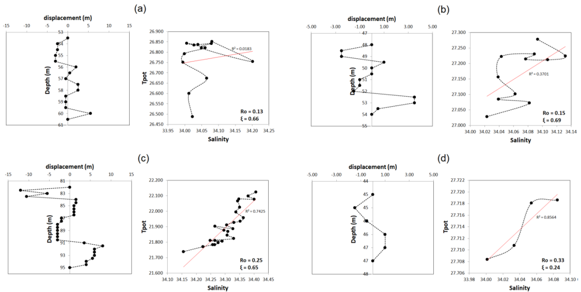
Figure 4.18 Some overturns that fail to pass the overturn selection criteria ( Ro < 0.2 and \xi > 0.66 ) (a, b); and overturns that pass the criterion (c, d).
