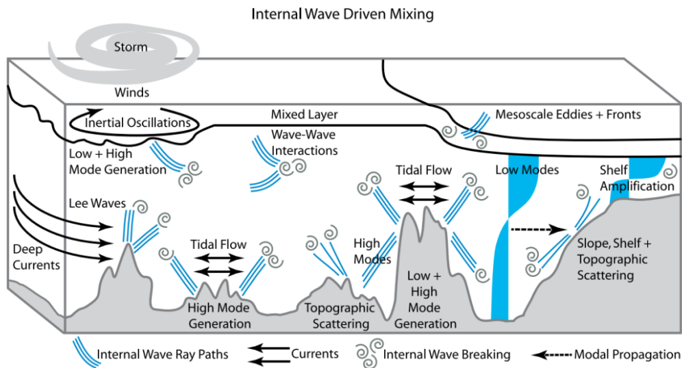
Figure 2.1 A sketch showing some of the features related to ocean turbulence. High-mode internal waves and low-mode internal waves are generated as tides interact with topographic features. The lee waves are formed as the deep currents flow over topography. Atmospheric phenomena such as storms produce inertial oscillations in the mixed layer, which can also generate both low- and high-mode internal waves. Such waves can interact in the open ocean. Approaching boundary regions, internal waves can amplify or scatter and eventually break, leading to energy dissipation (from MacKinnon et al., 2017).
