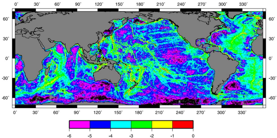
Figure 2.5 Global distribution of the energy flux in \log_{10} scale ( W m^{-3} ) from the diurnal M2 tidal component to internal waves. The black color means less than 10^{-6} W m^{-2} (from Nycander, 2005).
