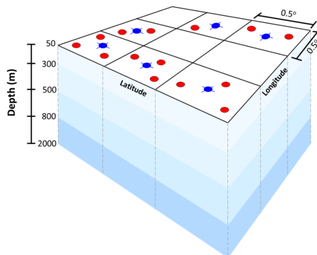
Figure 3.14 Spatial horizontal grid averaging method with 0.5^\circ degree longitude and latitude; and vertical layer averaging for several layer depths: 50-300 m, 300-500 m, 500-800 m, 800-2000 m. Red and blue dots represent vertical profile of CTD stations available in each grid and their mean profiles, respectively.
