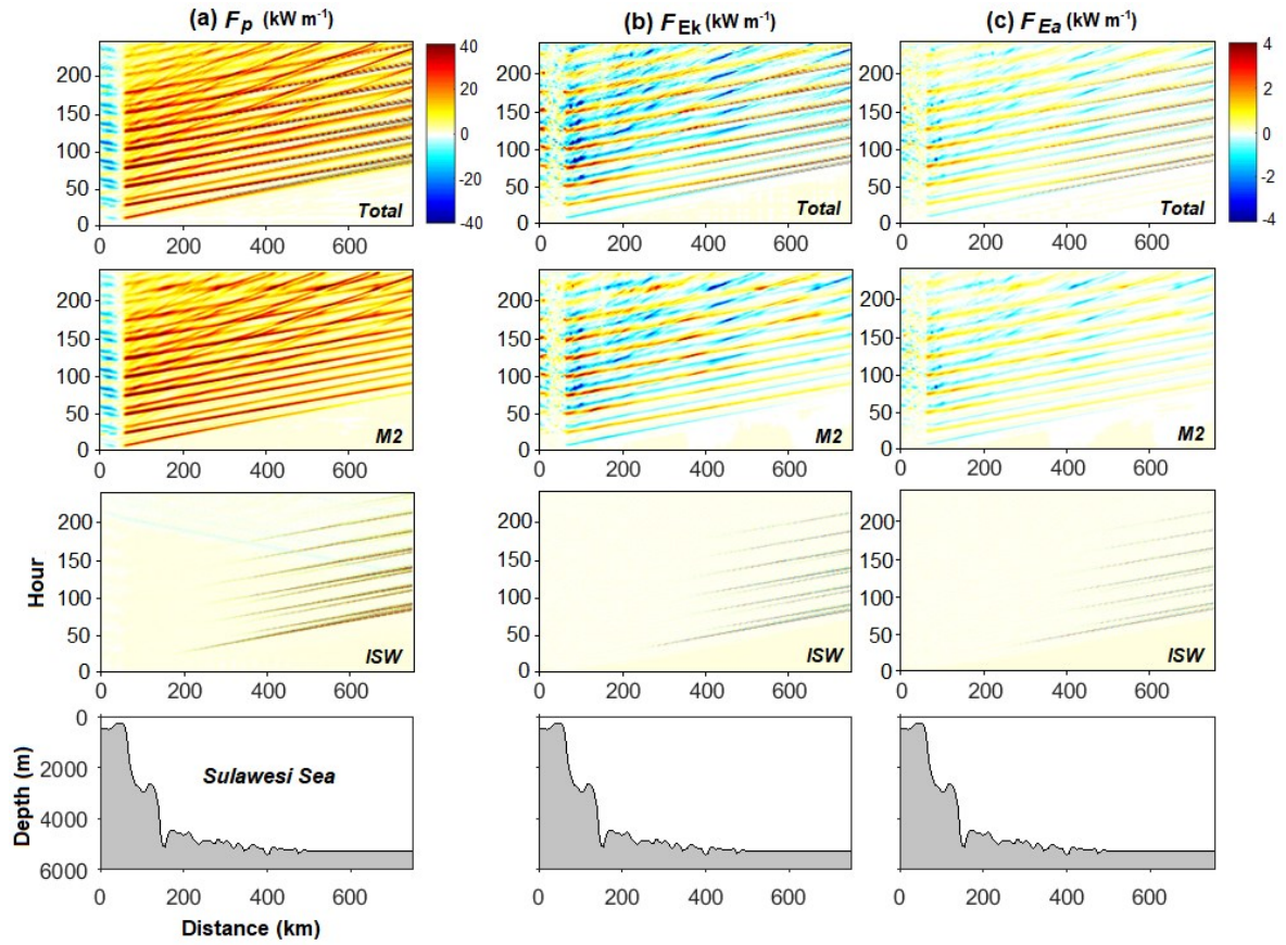
Figure 4.7 The time-space plots of depth integrated energy flux from the contribution of: (a) pressure perturbation flux, F_p = u'p' ; (b) kinetic energy flux, F_{Ek} = u'E_k and (c) potential energy flux, F_{Ea} = u'E_a . The first (upper), second and third panel is the total, low frequency/tidal and high frequency/ISW components, respectively.
