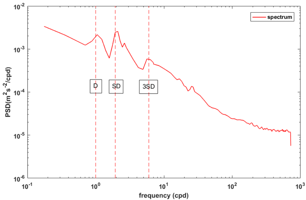
Figure 4.10 Power spectra of measured velocities, in the Manado Bay. The dashed red lines depict three tidal frequencies, the diurnal, D, the semi-diurnal, SD, and the third diurnal, 3SD .
