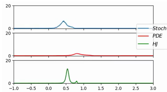
(c) t = 216
