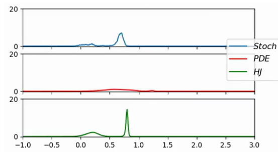
(b) t = 198
