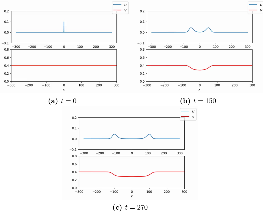
Figure 8.1 – v_0 = 0.4
