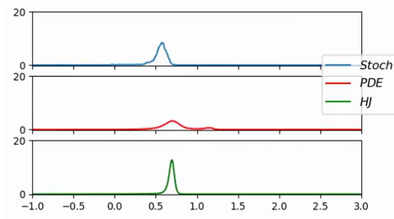
(a) t = 167
