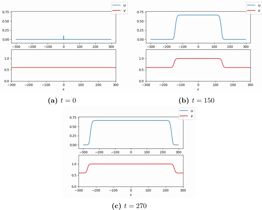
Figure 8.2 – v_0 = 0.6
