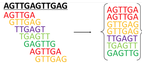
Figure 2.1: An illustration of how a read can be broken down into k -mers, in this case k = 6 ; Source: Hua and Zhang (2019)
