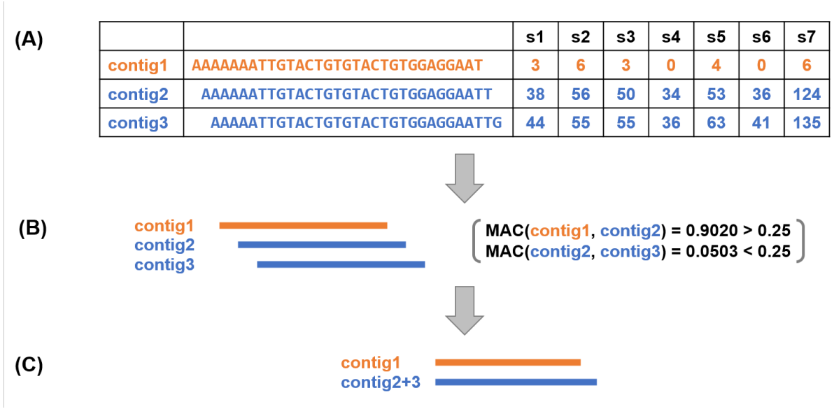
Figure 7.2: Merging procedure of 3 example contigs: A. Count table of contigs in samples. Both pairs (\text{contig1}, \text{contig2}) and (\text{contig2}, \text{contig3}) have good overlaps shifting by only one nucleotide, but the sample count vectors of contig1 and contig2 are not compatible. B. Merging intervention considering sample count compatibility between contigs. The Mean Absolute Contrast (MAC) is calculated for each pair, and merging of (\text{contig1}, \text{contig2}) is rejected due to a MAC value exceeding threshold. C. The resulting contigs are the initial contig1 and the merged contig from the initial (\text{contig2}, \text{contig3}) pair.
