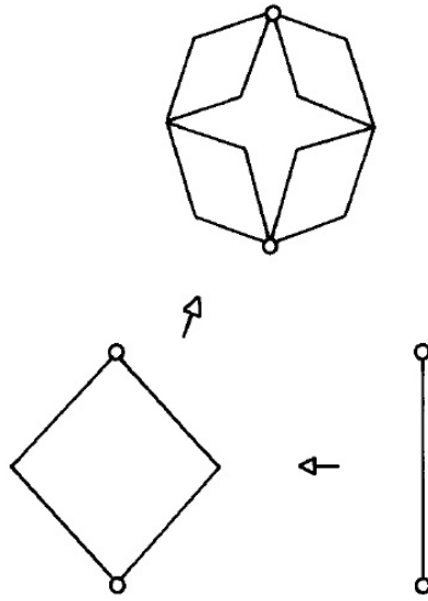
Figure 4.3 Hierarchical diamond lattice
