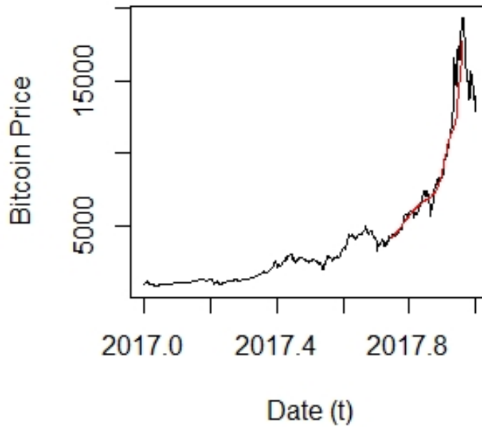
Figure 4.6 LPPPL fitting Bitcoin market prices
