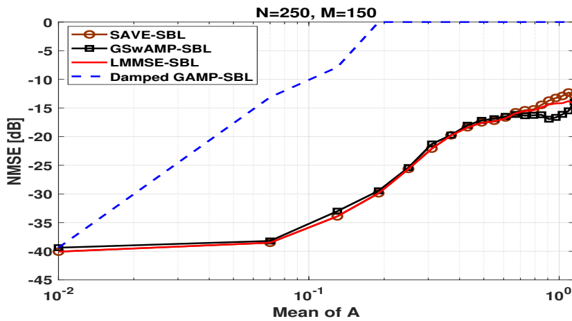
Figure 9.7: NMSE vs the mean of A .
