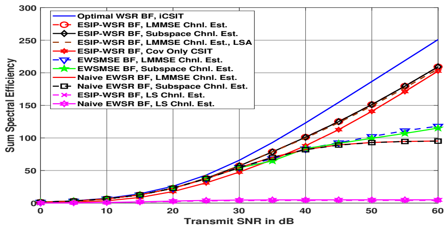
Figure 7.6: EWSR for C = 4 cell, K_i = 7, \forall i , So, K = 28 users, M = 64 , L = 2 , \tilde{\sigma}^2 = 0.1 . subspace channel estimators converge to the same performance at high SNR in the simulations which is also analytically proved in the chapter.
