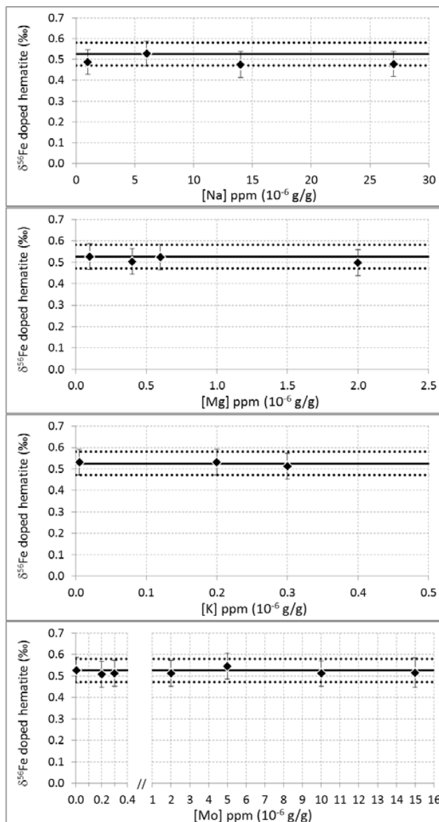
Figure 4. \delta^{56}\text{Fe} of hematite (200ppb natural Fe) doped with variable amounts of Na, Mg, K and Mo. Diamonds are the averages of duplicate measurements. Error bars are 2 standard deviations of the duplicate measurements or the long term internal precision (2SD) of our instrument (0.06‰), whichever the greatest. The horizontal black lines show the \delta^{56}\text{Fe} of pure (un-doped) hematite measured during the same analytical session; mean value (solid line) \pm 2 standard deviations (dotted lines).
