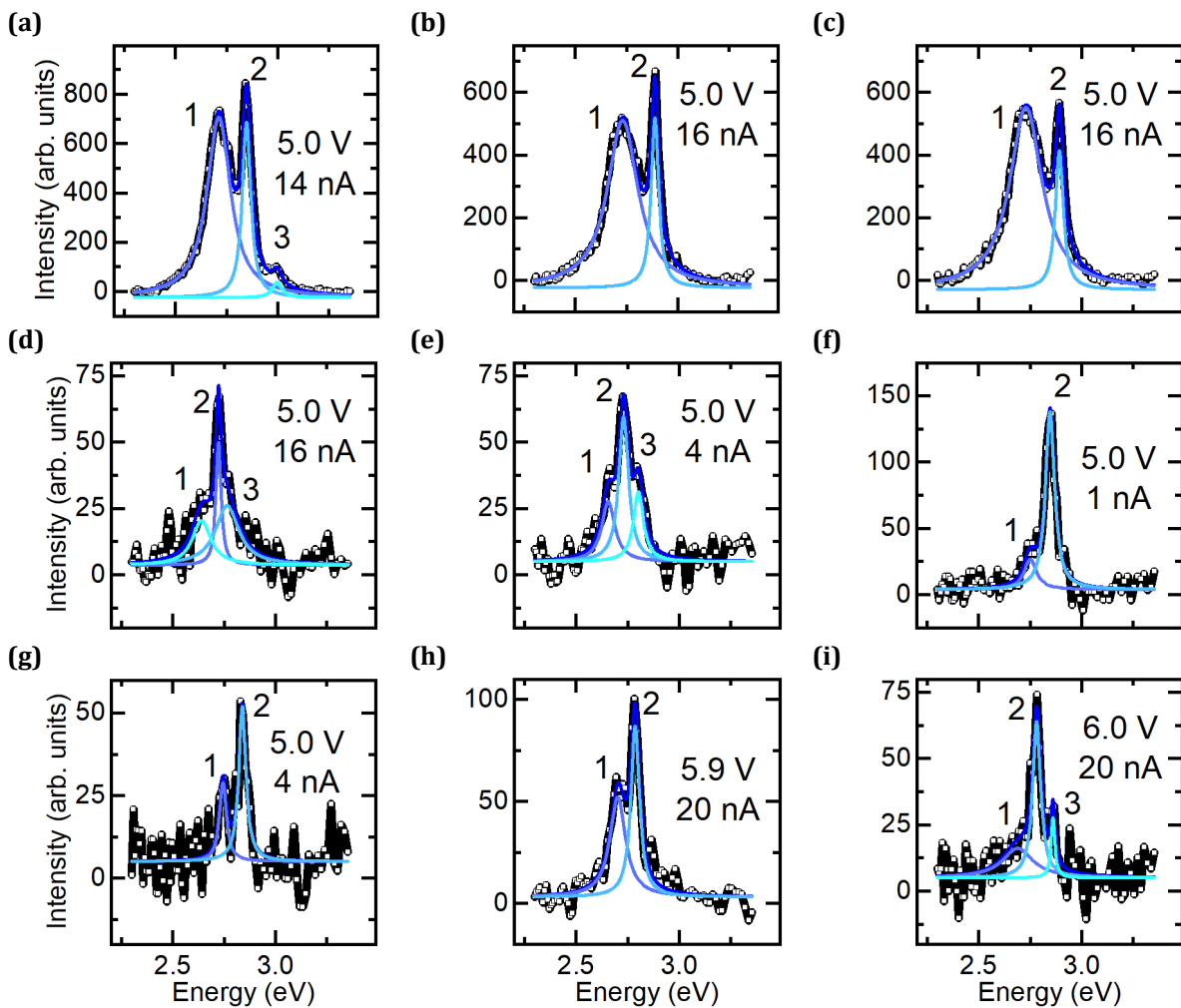
Figure 3.22: Selection of spectra with narrow emission peak from different measurement sets on the S10 sample. (a)-(c) Isolated narrow high energy peak separated from a broad low energy emission band. (d)-(f) Main narrow emission line with at least one (narrow) contribution at lower intensity.
