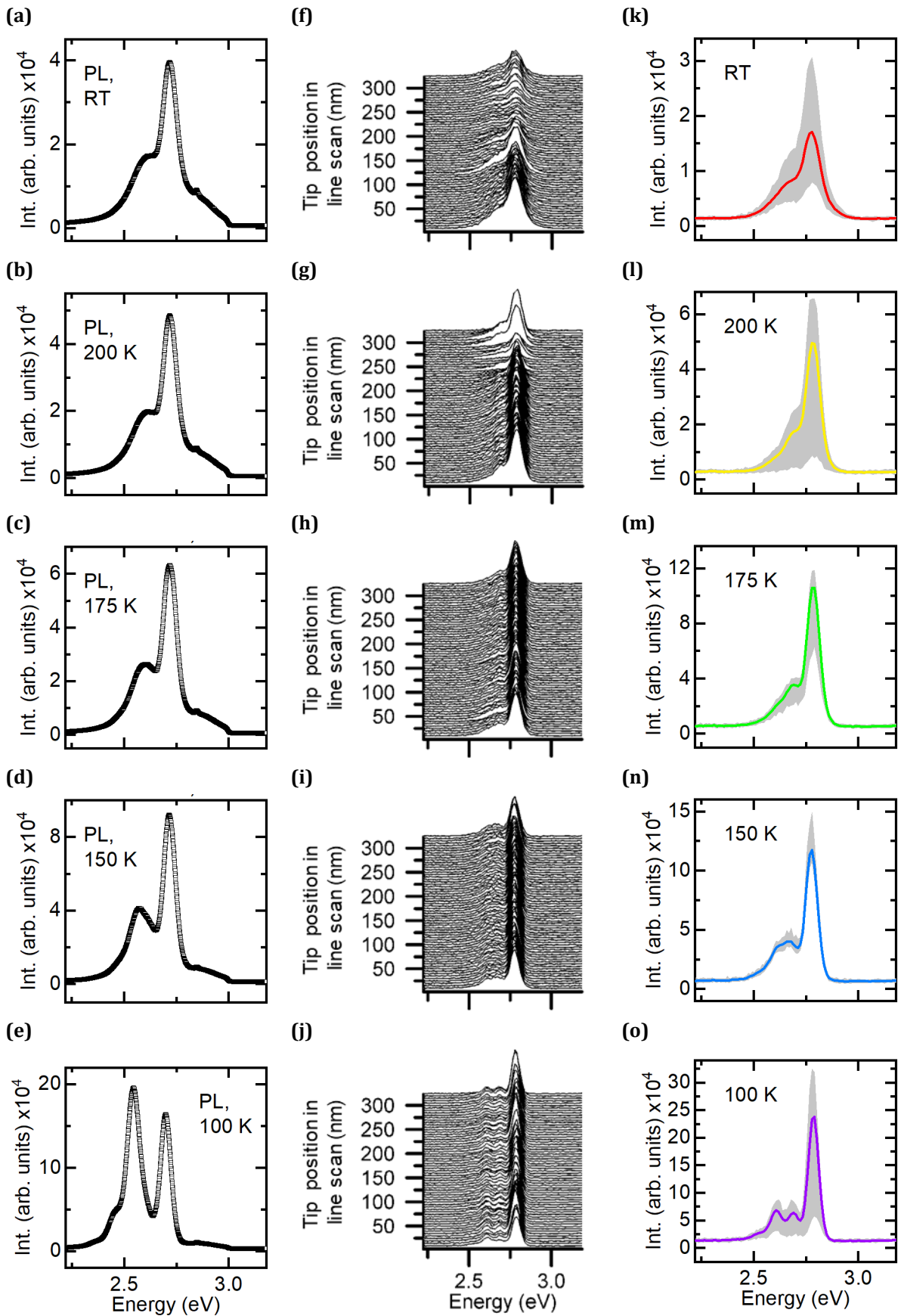
Figure 4.3: Summary of temperature dependent p-type DQW: (a)-(e) PL spectra, (f)-(j) STL line scan and (k)-(o) average value of spectrum in envelope of mean and maximum value at the respective temperature steps of RT, 200 K, 175 K, 150 K, 100 K.
