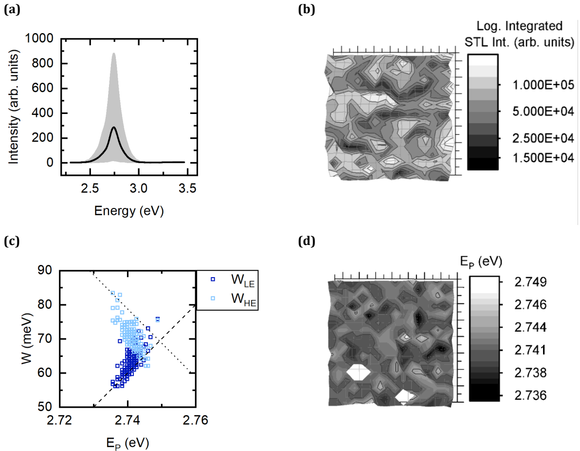
Figure 4.9: 64 nm x 64 nm STL map measurement on a flat area of the Soraa Inc. p-type sample surface. The tunneling bias and current are 4.5 V and 4 nA. The spectra are recorded at the nodes of a grid of 4 nm mesh size. (a) Averaged spectrum over the map. The grey envelope is delimited by the minimum and maximum intensity for each emission energy. (b) Integrated STL intensity map in logarithmic scale (c) Peak energy against W_{LE} and W_{HE} deduced after the data treatment of the map spectra (as described in Appendix A ). Dashed line has a slope of 1 whereas the dotted line has a slope of -1. (d) E_P emission peak energy map.
