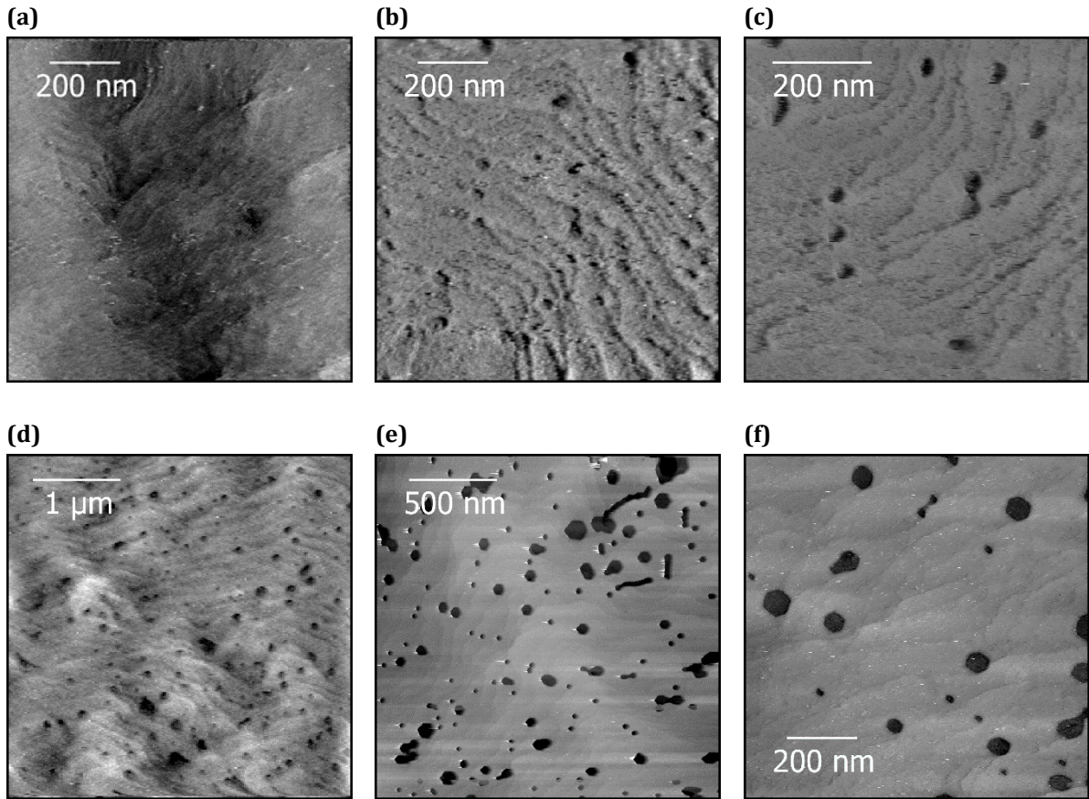
Figure 3.4: Topography with different false color scales for S10 (a) , (b) 1000 nm x 1000 nm (c) 700 nm x 700 nm; S90 (d) 4000 nm x 4000 nm (e) 2000 nm x 2000 nm (f) 1000 nm x 1000 nm.
