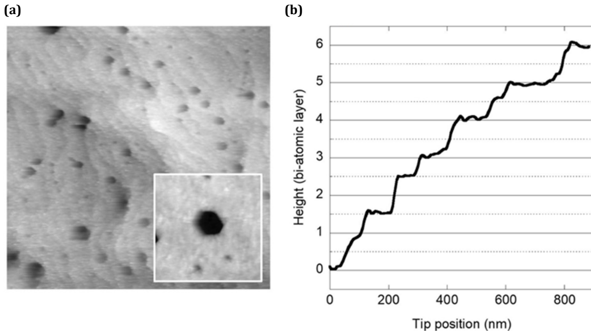
Figure 2.7: (a) 2.5 \mu\text{m} \times 2.5 \mu\text{m} STM topography of a GaN surface. The inset shows a zoom on a 0.5 \mu\text{m} \times 0.5 \mu\text{m} area around a hexagonal etch pit. (b) Surface profile showing terraces separated by bi- and mono-atomic steps [43].
