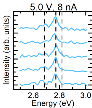
Figure 3.23: (a) Averaged STL emission spectra of the spectra shown in (b)-(d) at 5.0 V with 8 nA, 16 nA and 32 nA. Position of peak energy marked and labeled E_A = 2.684 eV, E_B = 2.772 eV, E_C = 2.819 eV.
