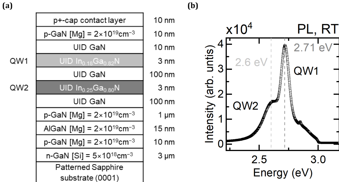
Figure 4.1: (a) Detailed structure of the p-type DQW sample heterostructure. (b) PL spectrum of p-DQW sample recorded at 300 K with an excitation at \lambda=373 nm pf about 5 mW.
