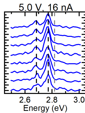
Figure 3.23: (a) Averaged STL emission spectra of the spectra shown in (b)-(d) at 5.0 V with 8 nA, 16 nA and 32 nA. Position of peak energy marked and labeled E_A = 2.684 eV, E_B = 2.772 eV, E_C = 2.819 eV.
