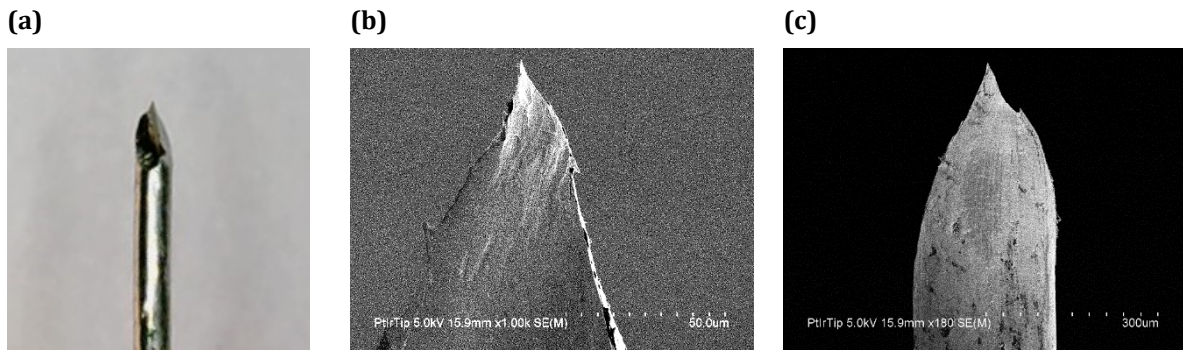
Figure 2.12: Pt-Ir STM tip made by the cut-and-pull technique (a) taken with an optical microscope. (b)-(c) Taken by a SEM. (a), (b) Front side of the tip. (c) Backside of the tip.
