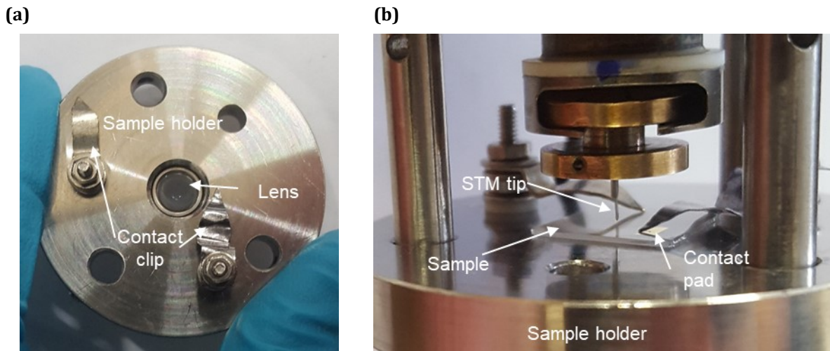
Figure 2.5: (a) Homemade sample holder containing a collecting lens with short focal length and contact clips. (b) sample placed on its holder and contacted via contact clips with STM tip close to its surface.
