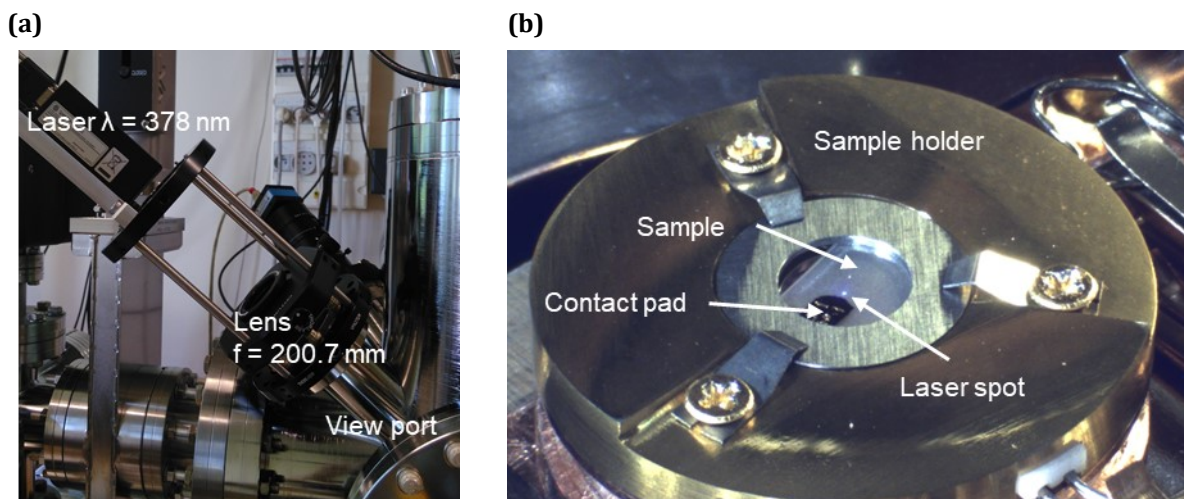
Figure 2.10: (a) Adaptation for in-situ photoluminescence characterization: focused laser light is injected through a view port onto the sample. (b) Focused laser light on sample.
