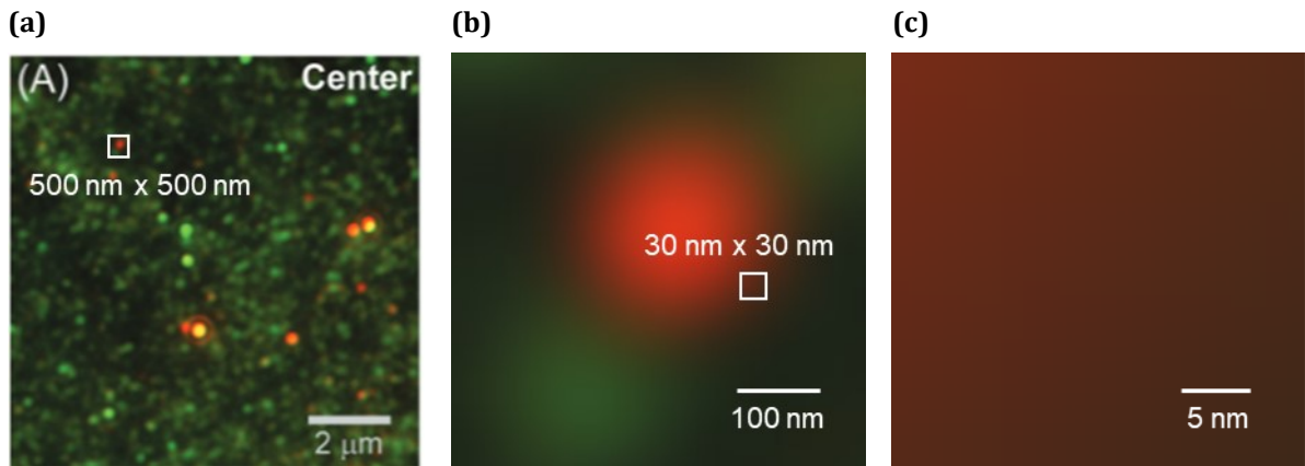
Figure 1.5: Spectrally resolved photoluminescence microscopy on InGaN/GaN QW. Gradual zoom into marked area from original size in (a) to 500 nm x 500 nm in (b) to 30 nm x 30 nm in (c). Reprint from [55].
