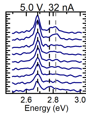
Figure 3.23: (a) Averaged STL emission spectra of the spectra shown in (b)-(d) at 5.0 V with 8 nA, 16 nA and 32 nA. Position of peak energy marked and labeled E_A = 2.684 eV, E_B = 2.772 eV, E_C = 2.819 eV.
