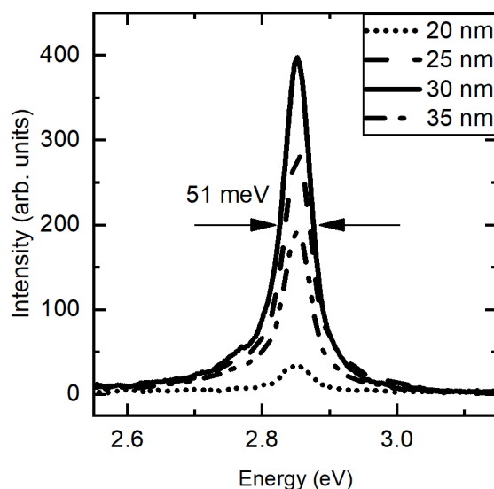
Figure 3.9: Evolution of the measured narrow emission lines (taken from Figure 3.8 at different positions of the line scans). The narrowest emission line of this series has a FWHM of 51 meV.
