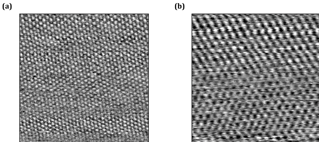
Figure 2.13: STM topography of HOPG recorded with 2 different tips revealing atomic resolution. (a) 7 nm x 7 nm, (b) 6 nm x 6 nm.
