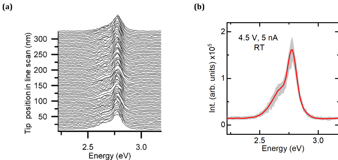
Figure 4.2: (a) STL line scans at room temperature (RT), (b) average spectrum over the line scan (red line) and envelope of maximum and minimum values along the line scan (grey envelope).
