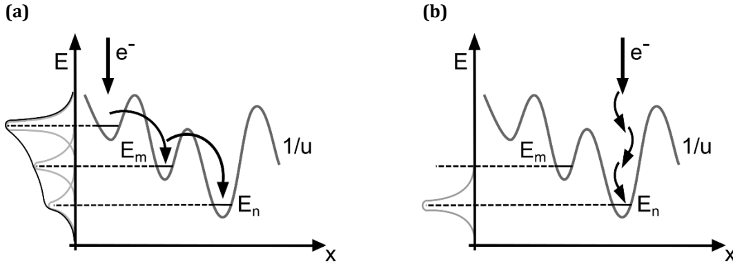
Figure 3.17: Sketch of the in-plane transport of electron injected in the effective potential 1/u of the localization landscape theory before recombining for (a) a high energy region and (b) a low energy region.
