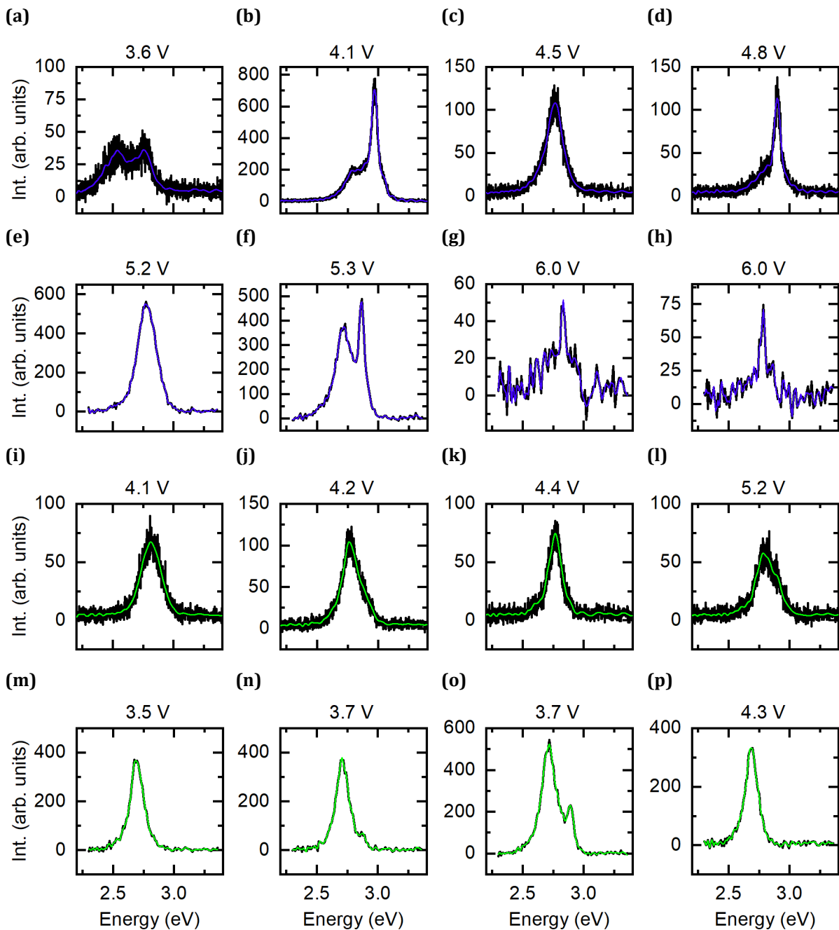
Figure 3.7: Local tunneling electroluminescence spectra measured under local electron injection on (a-h) S10 sample at (a-d) 2 nA and (e-h) 20 nA, and on (i-p) S90 sample at (i-l) 2 nA and (m-p) 20 nA. The applied tunneling bias voltage is indicated on top of each spectrum. The black curves are the background-corrected raw data. The colored curves are the spectra obtained after the smoothing procedure explained in the Appendix A.
