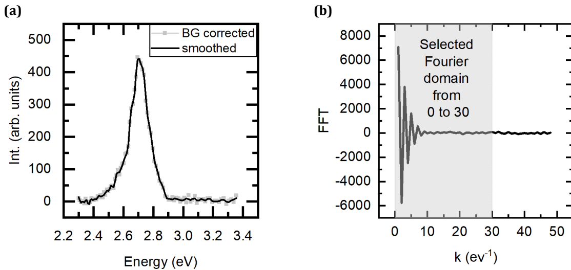
Figure A.4: (a) STL spectrum before (grey dots) and after (black line) fast Fourier Transform (FFT) filtering. (b) FFT of spectrum energy ( k ) the spectrum with the selected filtering interval.
