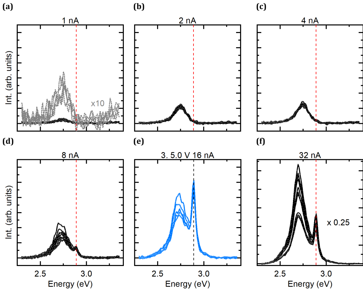
Figure 3.20: Variation of the local tunneling electroluminescence spectrum as a function of the tunneling current injected at the same tip position with constant tunneling bias voltage of 5.0 V. The narrow high-energy peak is tagged by a vertical dashed line.
