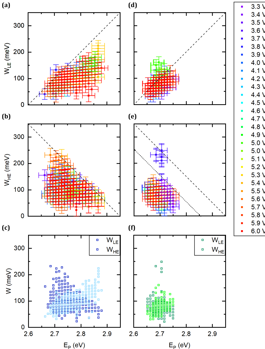
Figure 3.16: Variations of W_{LE} and W_{HE} against E_p for line scans recorded on (a-c) S10 and (d-f) the S90 samples with applied bias varying from 3.3 V to 6.0 V at 20 nA injected current. In (c) and (f) all data of W_{LE} (light colors) and W_{HE} (dark colors) are superimposed. The dashed lines have a slope 1 in (a) and (d) and a slope -1 in (b) and (e) .
