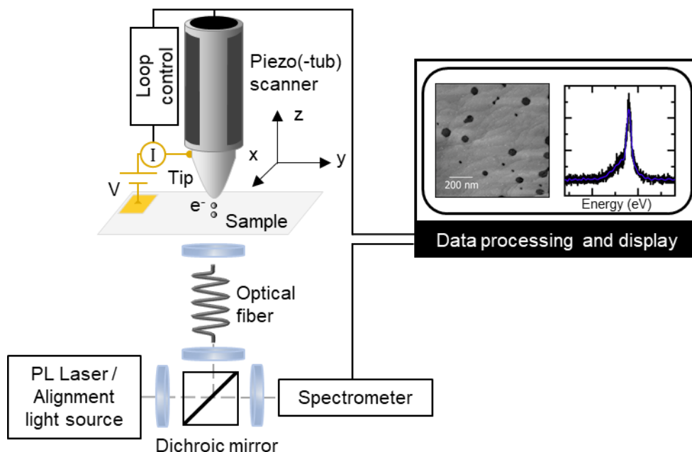
Figure 2.6: Schematic of our complete STL setup, including the photoluminescence (PL)/alignment line and data processing.
