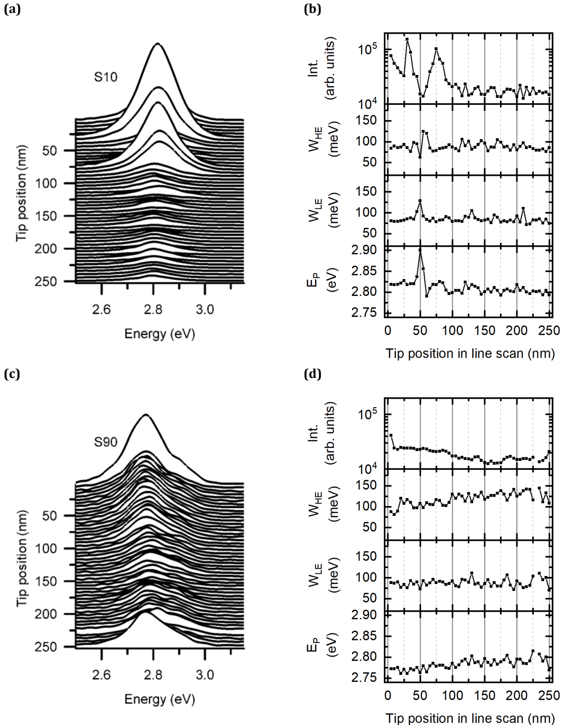
Figure 3.13: Line scans measured at low injection current of 2 nA on S10 (a) – (b) and S90 (c) – (d) at a bias of 4.2 V. The spectra are taken with a spacing of 5 nm on line scans of length 250 nm. (a) (respectively (c) ) Spectra of the line scan, and (b) (respectively (d) ) Data treatment of those spectra for S10 (respectively S90).
