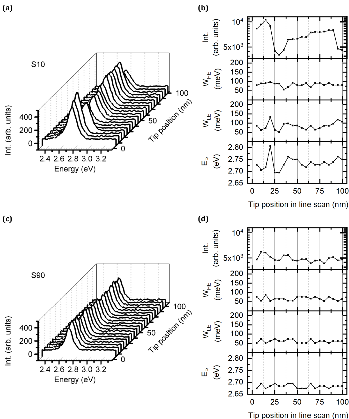
Figure 3.15: Line scans measured at high injection current of 20 nA on S10 (a) – (b) and S90 (c) – (d) at a bias of 4.3 V. Spectra are taken with a spacing of 5 nm. (a) (respectively (c) ) Spectra of the line scan. (b) (respectively (d) ) Data treatment of those spectra for S10 (respectively S90).
