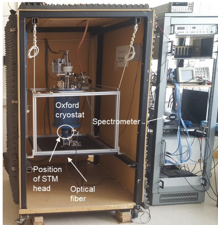
Figure 2.4: Omicron CRYOSXM STL in ambient conditions (air) setup free swinging inside the isolation box with homemade adaptations and spectrometer on the right-hand side.
