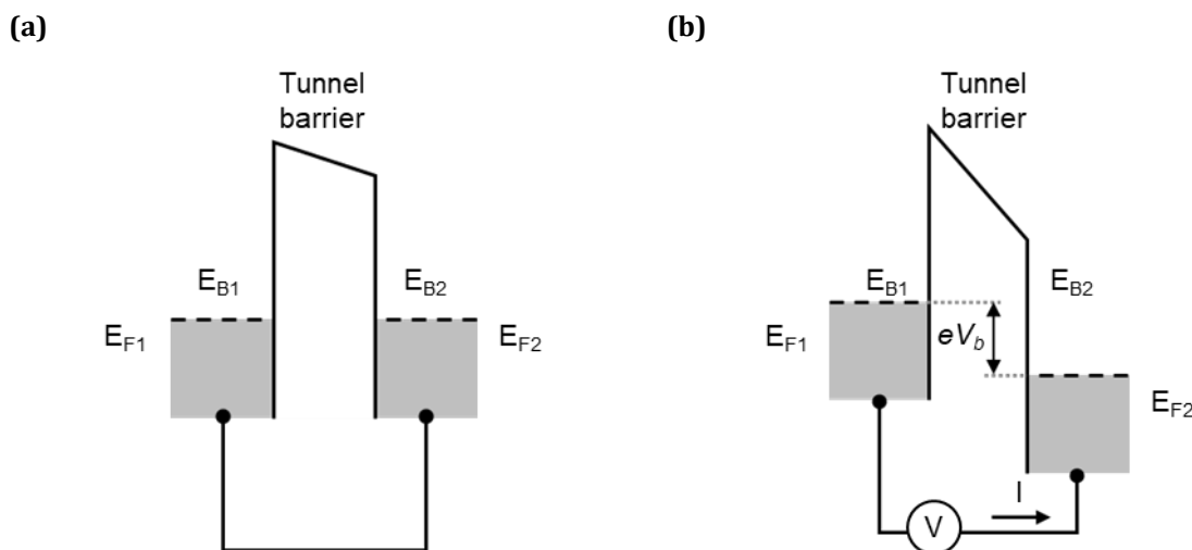
Figure 2.1: Tunneling through a barrier between two conducting solids with different work function. (a) Without applied bias voltage and (b) with applied bias voltage.
