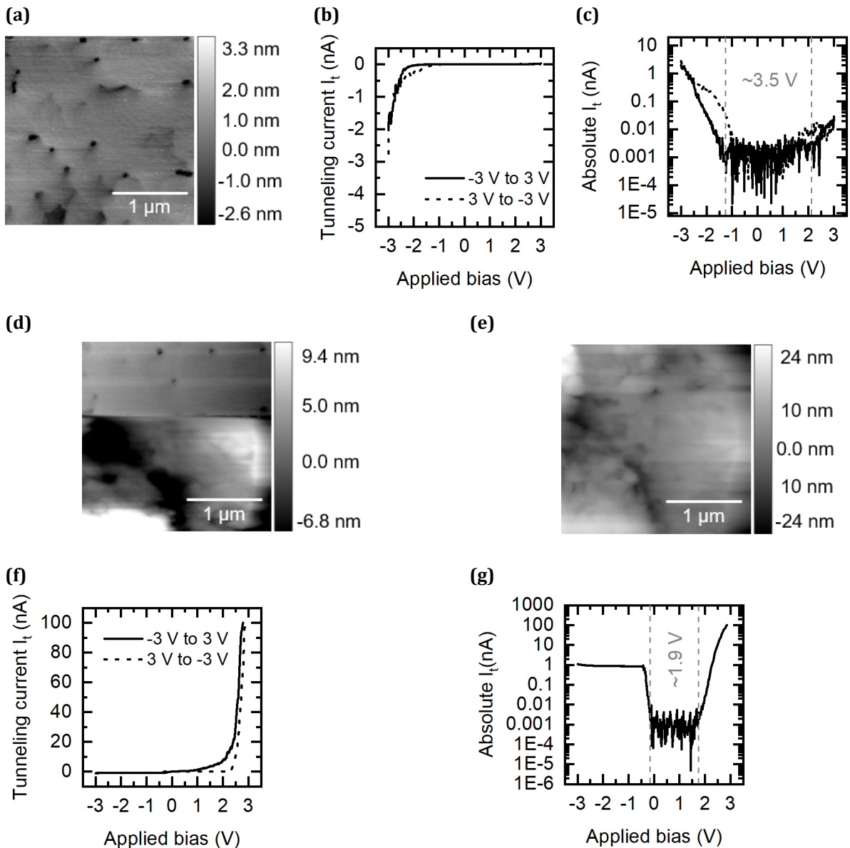
Figure 4.12: Topography of the n-type sample at -2.8 V and -1 nA (a) without charge accumulation with corresponding IV-characteristic (b) in linear scale and in logarithmic scale (c) . (d) Topography image of the same area with sudden switch in the surface due to charge accumulation and (e) fully charged surface of the same area. IV-characteristic of charge accumulation in (f) in linear scale and (g) in logarithmic scale.
