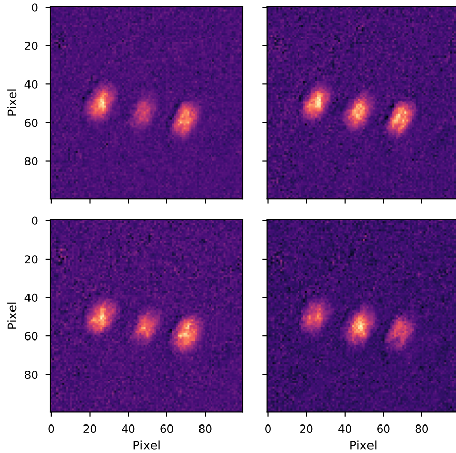
Bose Einstein condensate after Stern-Gerlach separation
