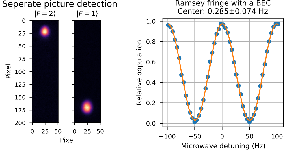
Figure 4.5: Left: separate images of the BEC output state of a microwave pulse sequence. First, atoms in |F=2\rangle are observed and subsequently removed. Then a second image is taken \sim 5 ms after which detects atoms in |F=1\rangle . Right: through the analysis of set of images, one can reconstruct Ramsey fringes.
