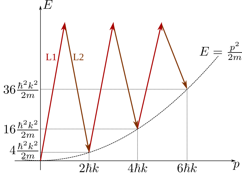
Figure 2.8: Energy momentum diagramm of repeated Raman transitions in the same internal state.
