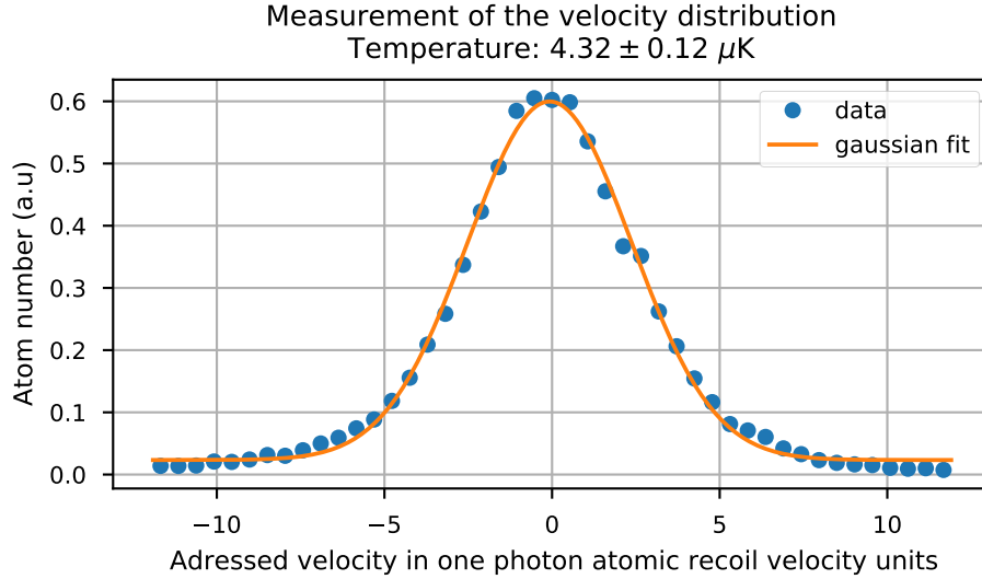
Figure 3.7: Velocity distribution at the output of the molasse stage. Data (blue dots) was taken by scanning the addressed velocity of an elevator-selection sequence (see section 3.3) and measuring the atom number at its output. Data is fitted by a gaussian (orange line), from which we extract a 1/e velocity width of \sim 3.5 one photon recoil velocity. This corresponds to a temperature of \sim 4.3 \mu\text{K} .
