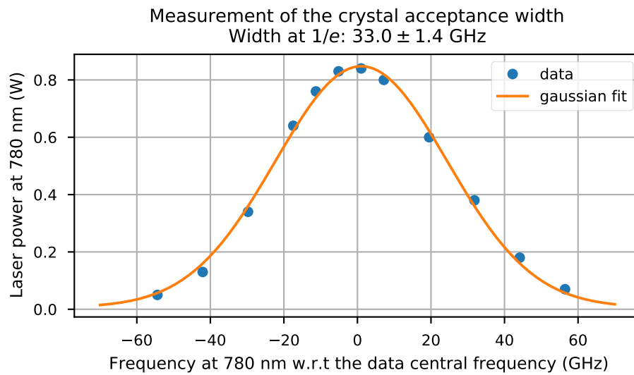
Figure 3.12: Output power of the amplifier-doubling module as a function of the seeder frequency (converted to 780 nm). The temperature of the doubling crystal is constant, such that this figure represent the width of the crystal acceptance.
