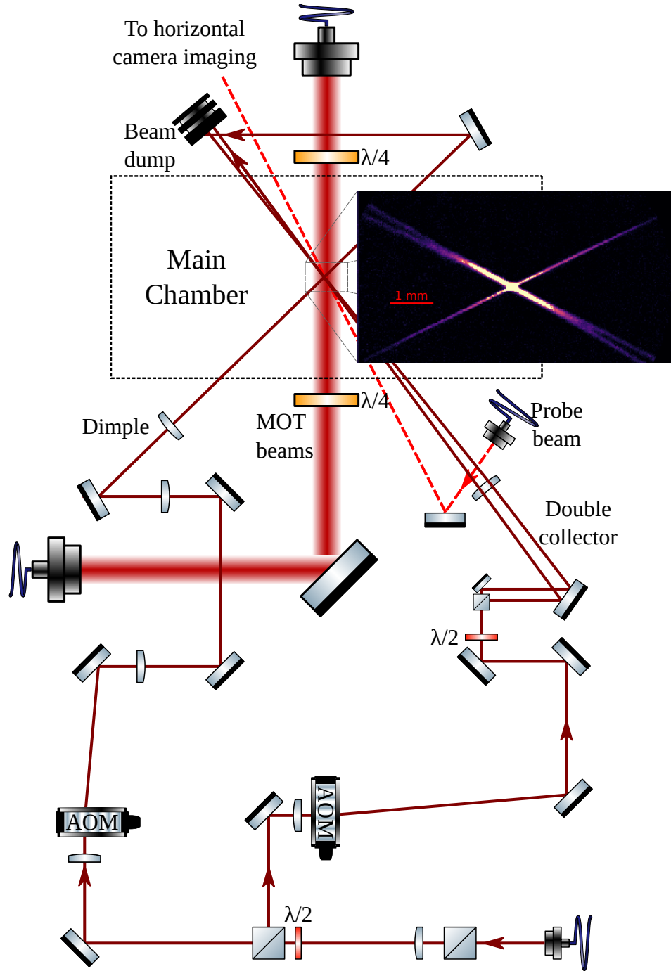
Figure 3.9: Schematic representation of the optical tables surrounding the main chamber (top view). The setup mainly correspond to the dipole beam setup for evaporative cooling (dark red lines), but also contains the horizontal MOT beams (large red) and the horizontal camera path (dashed red lines). Inset: image of the three dipole beams through the observation of atoms that are trapped at very short time of flight (1 ms). The image is saturated so that the tails of the trap are distinguishable.
