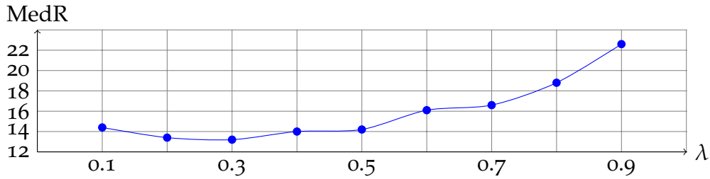
Figure 2.8 – MedR scores for different values of \lambda , responsible for weighting the semantic regularization cost \mathcal{L}_{sem} of AdaMine , calculated over 5 bags of 10.000 validation samples.
