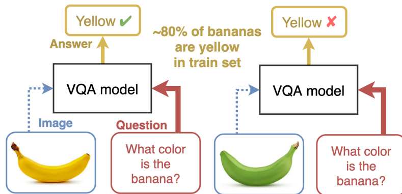
Figure 4.1 – Current VQA models often rely on unwanted statistical correlations between the question and the answer instead of using both modalities. A biased model will answer yellow without looking at the image, because it learned that the presence of the words what , color and banana is highly predictive of the answer yellow .
