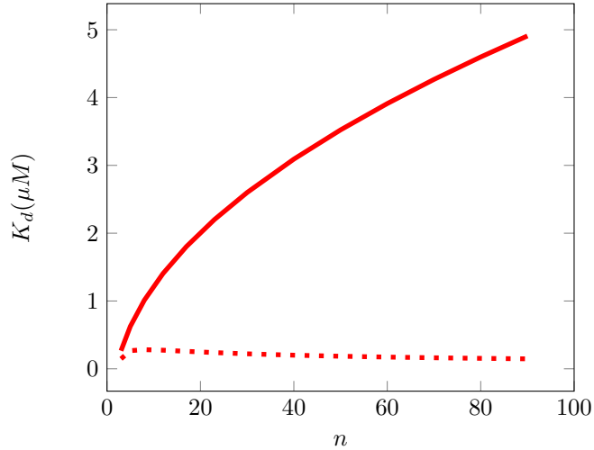
FIGURE 2.8 – The dissociation constant K_d determined from (2.33) (solid line) and (2.34) (dashed line), depending on the p62 oligomer size n . Ubiquitin and p62 oligomer concentrations from Figure 2.6 at the onset of aggregation : [Ubi] = 1.6\mu M , [p62_n] = 0.4\mu M .
