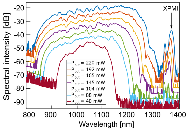
Fig. 4. SC evolution for different pump powers while pumping at 45° from the two axes (power offset for clarity).
