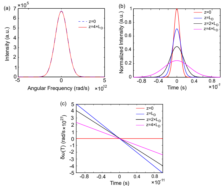
Figure 2.7: (a) Calculated spectrum of a 1 ps Gaussian pulse before and after propagating a distance z = 4 \times L_D , demonstrating the preservation of its spectral shape. (b) Normalized intensity |A|^2 , showing the temporal pulse broadening and (c) frequency chirp \delta\omega/\delta t as a function of time for z = 0 , z = L_D , z = 2 \times L_D , and z = 4 \times L_D .
