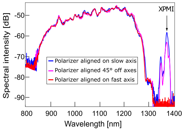
Fig. 5. SC evolution for different polarizer orientations while pumping at 45° from the two axes.
