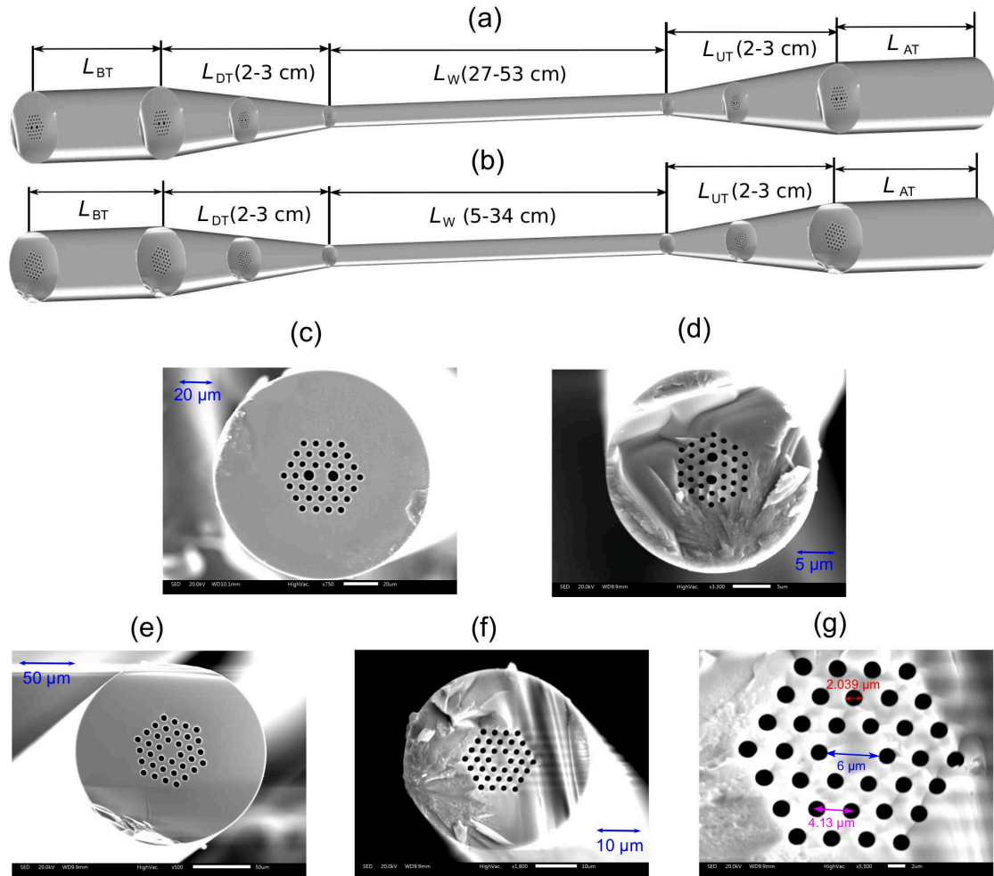
Figure 4.8: (a) & (b) Schematic of longitudinal sections of As_{38}Se_{62} PM-PCF tapers and Ge_{10}As_{22}Se_{68} PCF tapers, respectively: length before taper ( L_{BT} ), length of down-taper section ( L_{DT} ), length of uniform taper-waist section ( L_W ), length of up-taper section ( L_{UT} ), and length after taper ( L_{AT} ). (c) & (d) Cross-section images of normal section and taper-waist section of As_{38}Se_{62} PM-PCF with respective outer diameter ( d_{out} ) of 162 \mu m and 28.74 \mu m and respective core diameter ( d_{core} ) of 10 \mu m and 1.77 \mu m . (e) Cross-section image of normal section of Ge_{10}As_{22}Se_{68} PCF with d_{out} of 166.5 \mu m and d_{core} of 14.59 \mu m . (f) Cross-section image of taper section of Ge_{10}As_{22}Se_{68} PCF with d_{out} of 68.47 \mu m and an expanded view of the taper waist region in (g) showing d_{core} = 6 \mu m , d_{SA} = 2.039 \mu m , and \Lambda = 4.131 \mu m .
