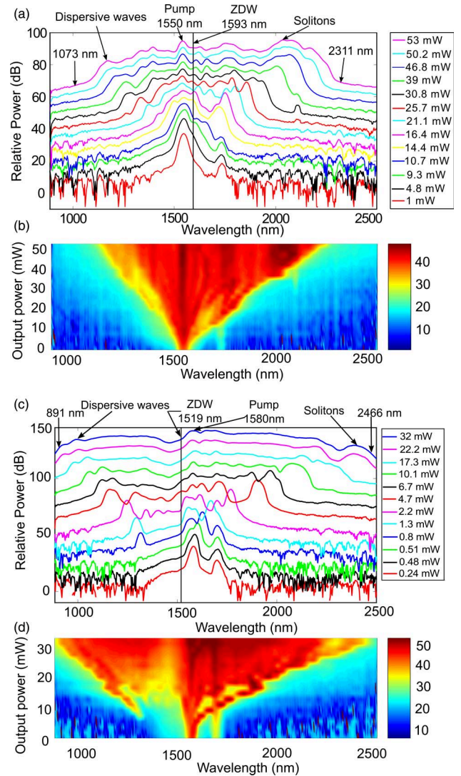
Fig. 5. Supercontinuum spectra generated in two SC-PCF samples with 200 fs pulses pumped at 1550 nm and 1580 nm, respectively, as a function of mean output power. (a) and (c) Generation of SC spectra through spectral broadening, soliton ejection, and dispersive wave generation in two fiber samples, NL44C2a and NL44C5c, respectively. (b) and (d) Evolution of SC spectrum with the fiber output power for SC-PCF samples NL44C2a and NL44C5c.
