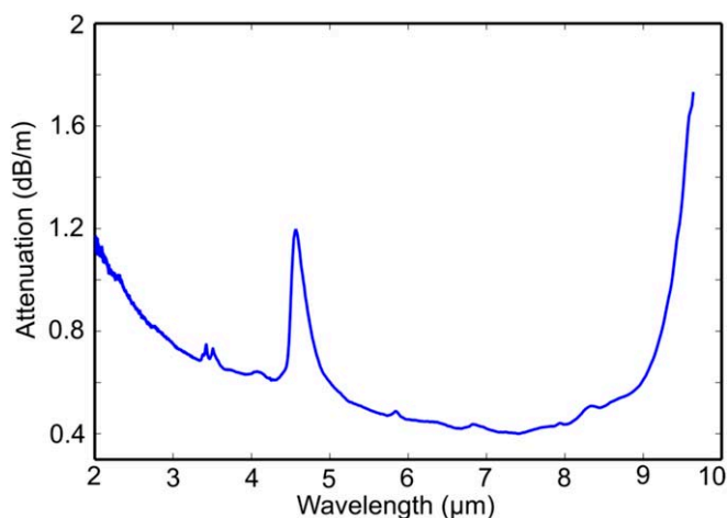
Figure 1. Attenuation spectrum of bulk \text{As}_{38}\text{Se}_{62} glass.
