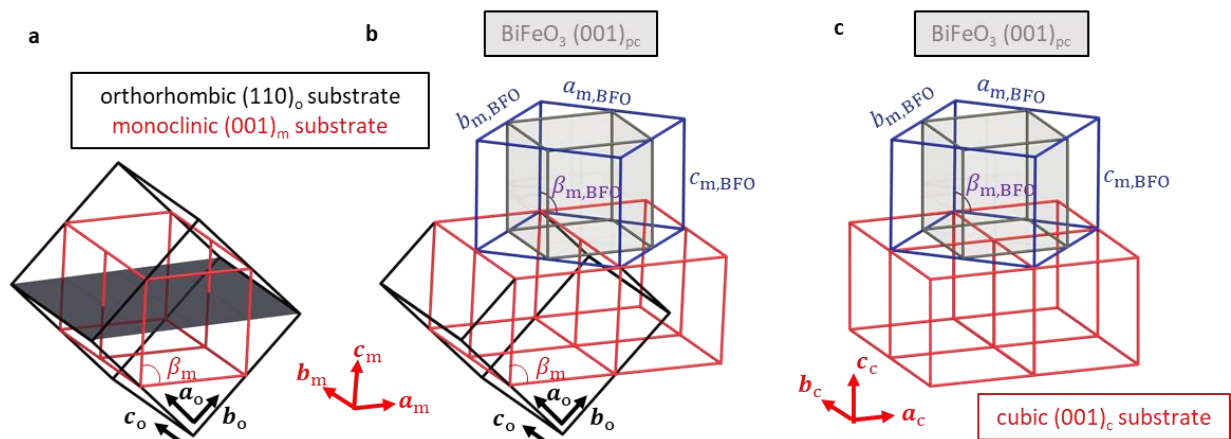
Figure 19 : a Relation between the orthorhombic (110)_o unit cell (black lines) and the monoclinic (001)_m one (red lines). b Growth of the \text{BiFeO}_3 film on this substrate. The monoclinic \text{BiFeO}_3 (001)_m unit cell is shown in blue, the pseudo-cubic \text{BiFeO}_3 unit cell in grey. c Very similar scenario for \text{BiFeO}_3 growth on cubic (001)_c substrates (red).
