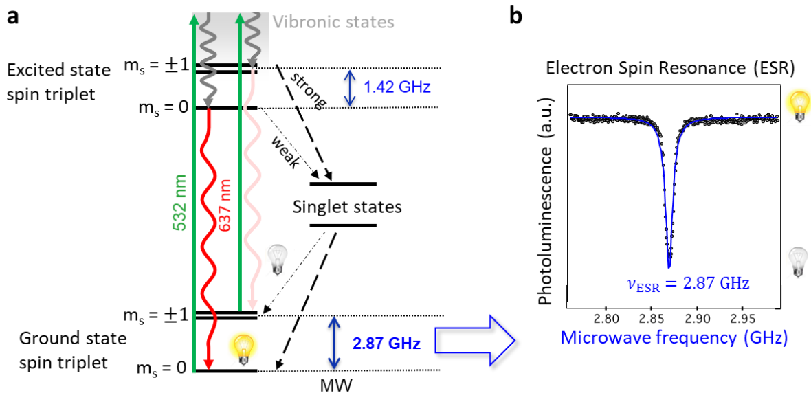
Figure 40 : Optically detectable magnetic resonance (ODMR) explained with a , the electronic level structure of the NV centre and b , the optical detection of the electron spin resonance spectrum.
