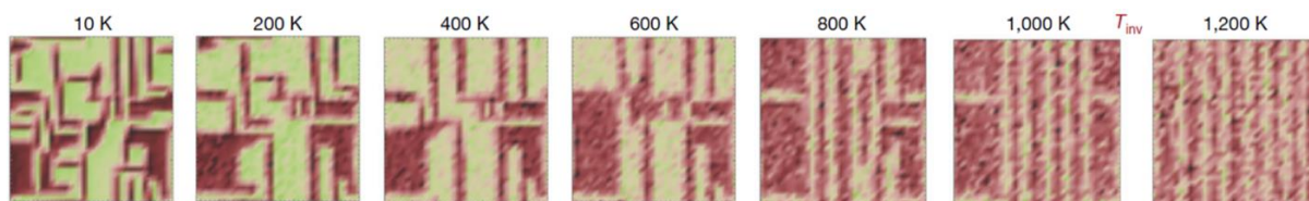
Figure 70 : Calculated inverse phase transition in a \text{BiFeO}_3 thin film under -0.16\% compressive strain. Adapted from reference [131].
