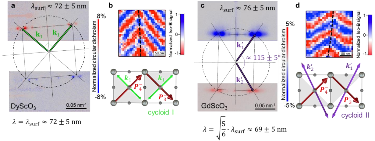
Figure 84 : The two types of spin cycloids in real and reciprocal spaces. a, c X-ray resonant magnetic scattering at the Fe L-edge for BiFeO 3 grown on DyScO 3 and GdScO 3 , respectively. b, d Corresponding NV magnetometry image zoomed in, with the propagation vectors sketched for both polarization variants. Figure adapted from reference [136].
