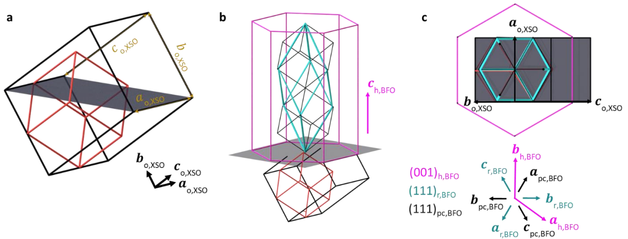
Figure 20 : a \text{XScO}_3 (011) orthorhombic substrate (black lines) with the construction of a pseudo-cubic cell in red. b Sketch of a \text{BiFeO}_3 film growing along the pseudo-cubic (black) (111)_{pc} , rhombohedral (turquoise) (111)_r direction and the hexagonal (pink) (001)_h direction on top of it. c Top view on the (011)_o orthorhombic plane.
