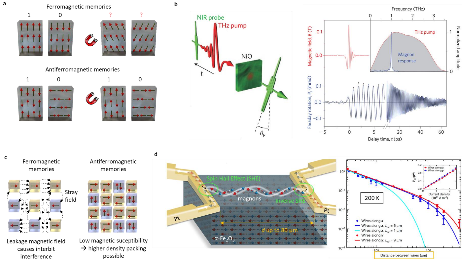
Figure 1 : Advantages of antiferromagnets for spintronics: a Insensitivity to spurious magnetic fields. Figure adapted from reference [1]. b Fast magnetization dynamics in the THz range as illustrated in NiO (adapted from reference [1]). c Possibility for higher density packing due to the absence of magnetic stray fields. d Long distance spin transport, shown in an example adapted from reference [1] in \alpha\text{-Fe}_2\text{O}_3 single crystals.
