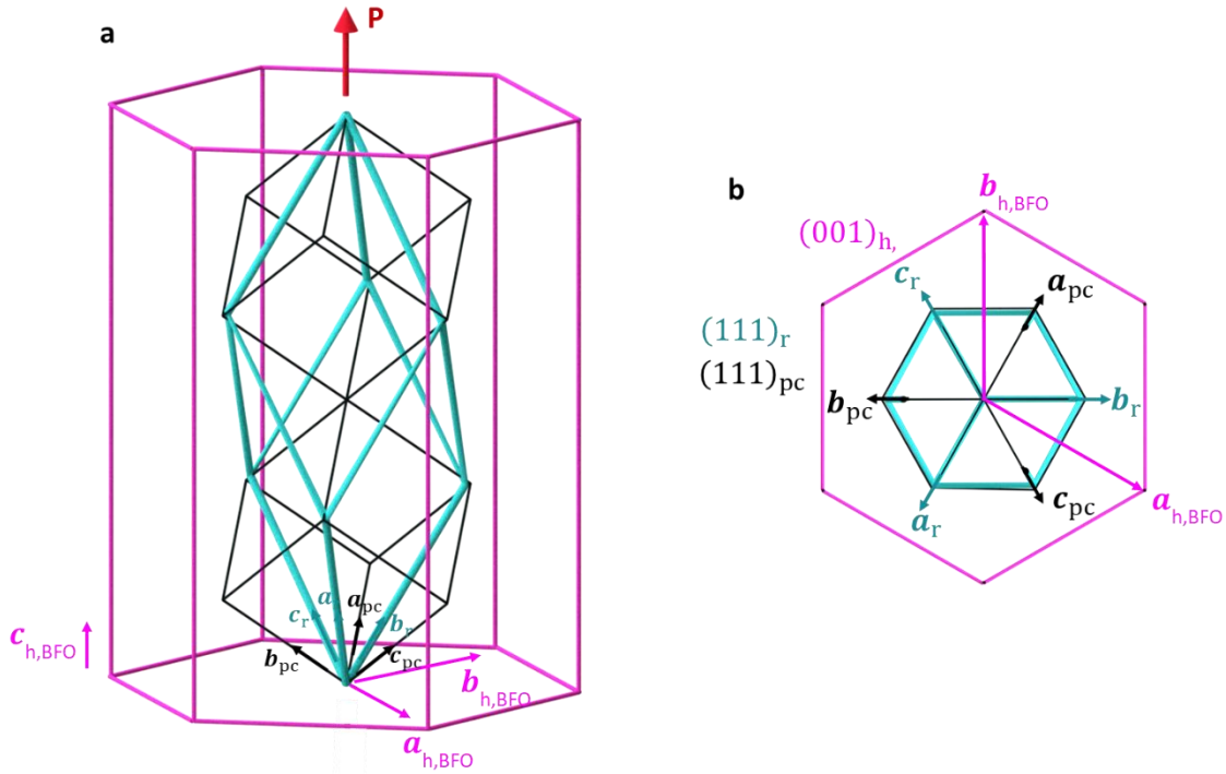
Figure 18 : Hexagonal (pink), rhombohedral (turquoise) and pseudo-cubic (black) unit cell of \text{BiFeO}_3 in a the side 3D-view and b the top view on the (001) hexagonal plane.
