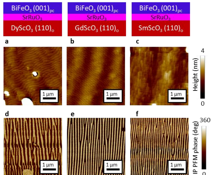
Figure 56: BiFeO 3 thin film growth on various substrates as sketched in the upper panel. a-c Topography, d-f in-plane PFM phase.
