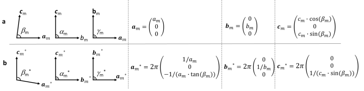
Figure 24 : Lattice vectors of a monoclinic unit cell in a real space and b reciprocal space.
