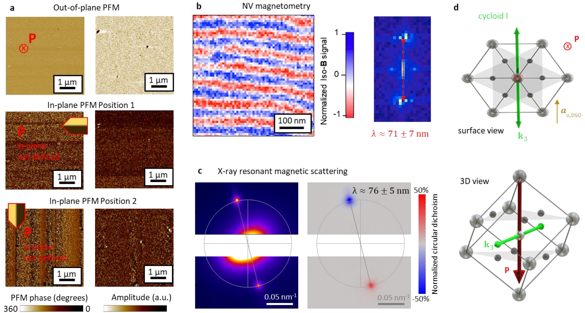
Figure 91 : Analysis of the electric and magnetic landscapes in a \text{BiFeO}_3 (111)_{pc} sample grown on \text{DyScO}_3 (011)_o . a Vectorial PFM analysis, showing a vertical polarization, pointing downwards. b Scanning NV magnetometry image with its Fourier transformation, c resonant elastic X-ray scattering pattern at the Fe L edge and the corresponding circular dichroism pattern and d sketches for the corresponding configuration of the polarization \mathbf{P} and cycloid propagation direction \mathbf{k} .
