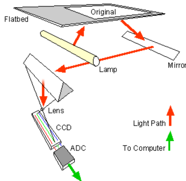
Figure 2-4: Basic scanning mechanism [25].
