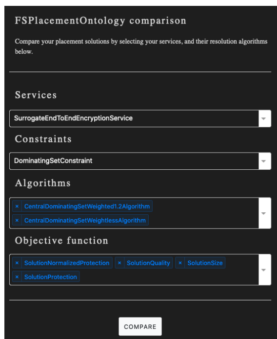
FIGURE 4.9 – Panneau de configuration de CSPS.
