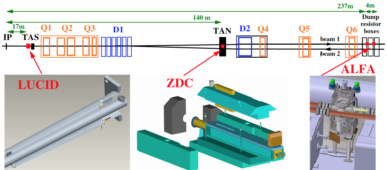
Figure 4.9: ATLAS forward detectors
