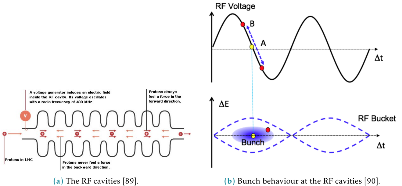
Figure 3.3: Bunching at RF cavities
