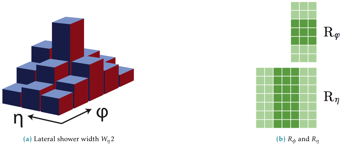
Figure 5.3: Shower shapes in the second layer of the electromagnetic calorimeter
