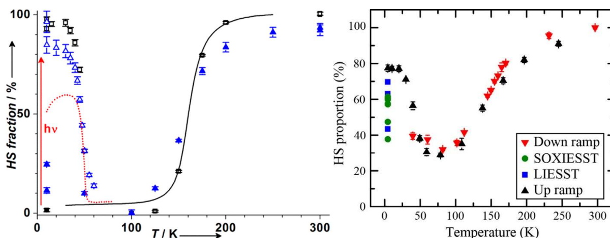
Figure 1-18. (a) HS fraction vs temperature for [\text{Fe}(\text{H}_2\text{B}(\text{pz})_2)_2(2,2'\text{-bipy})] evaporated as submonolayer on Au(111). 113 All values of HS fraction are derived from the linear interpolation of the XAS spectra for the bulk compound before (filled black squares) and after illumination (empty black squares) and the 300 nm thick film before (filled blue triangles) and after illumination (empty blue triangles) compared to the magnetometric results on the bulk compound before (full line) and after illumination (red dotted line). (b) HS fraction vs temperature for \text{Fe}[\text{HB}(3,5\text{-(Me}_2\text{)pz})_3] assembled as monolayer on Au(111). 115 HS fraction as a function of temperature as cooling down the sample from 300 to 4.4 K (red down triangles), exposing it with the illumination of soft X-ray (eight green points) and blue light (three blue square), and warming it up to 250 K (labeled as black up triangles).
