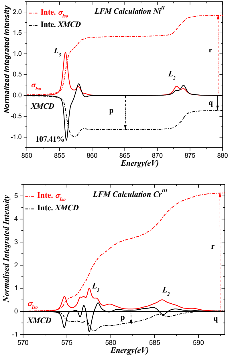
Figure II-3. Calculated Spectra applied magneto-optical sum rules for Ni II and Cr III site located in Cs I Ni II Cr III @HOPG. All the applied CF parameters in atomic multiplet calculations are listed in Table 3-1. For Ni II ions, it is carried out by the linear combination with C 4v in 48% and O h in 52% while for Cr III ions they are in purely octahedral symmetry.
