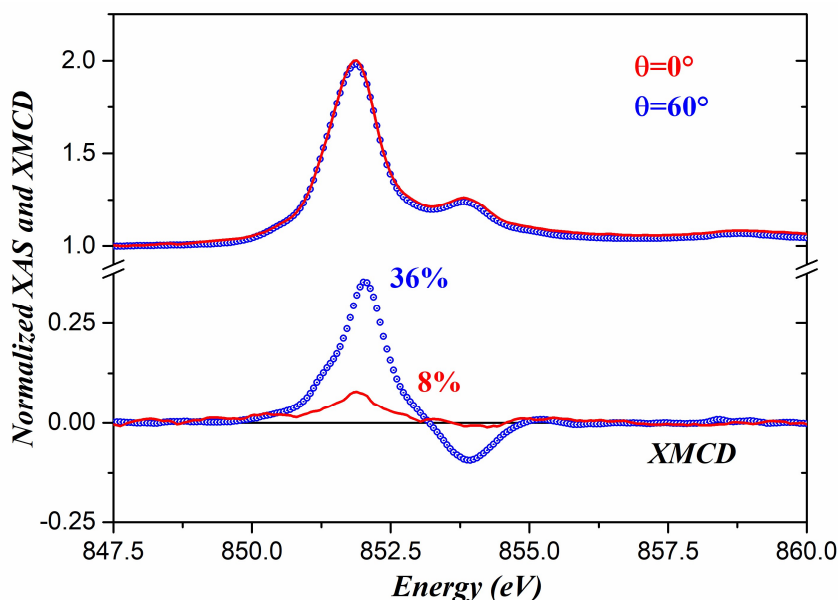
Figure 3-15. XMCD signals for remnant magnetization of \text{Ni}^{\text{II}} ions recorded between 0^\circ and 60^\circ at 2 K.
