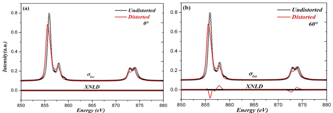
Figure 3-5. Simulated X-ray absorption spectra at the L_{2,3} edges of \text{Ni}^{\text{II}} obtained from different symmetries carried out by LFM calculations, including pure O_h (Undistorted) and C_{4v} (Distorted). Figure 3-5(a) is for the calculated XAS spectra at \theta = 0^\circ , while Figure 3-5(b) is for calculated spectra at \theta = 60^\circ . All CF parameters are listed in Table 3-1 .
