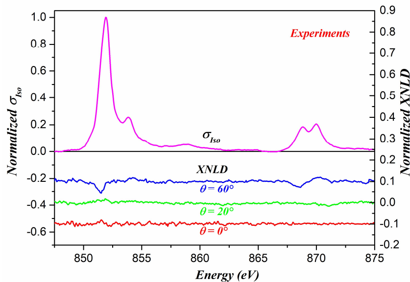
Figure 3-4. Experimental spectra among XAS and XNLD recorded at the L_{2,3} edges of \text{Ni}^{\text{II}} sites. All spectra are normalized so that the maximum of the L_3 edges is “1”. Magenta solid line is the normalized isotropic spectrum, XNLD signals are reported for 0^\circ (red), 20^\circ (green) and 60^\circ (blue) solid lines.
