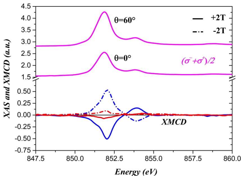
Figure 3-14. Angular dependence of the remnant XMCD signals for \theta = 0^\circ and \theta = 60^\circ at T = 2 K; +2T (-2T) indicate the initial value of the external magnetic field. The (\sigma_{\text{Right}} + \sigma_{\text{Left}})/2 cross-sections are raw data and have not been normalized at the difference of Figure 3-15 .
