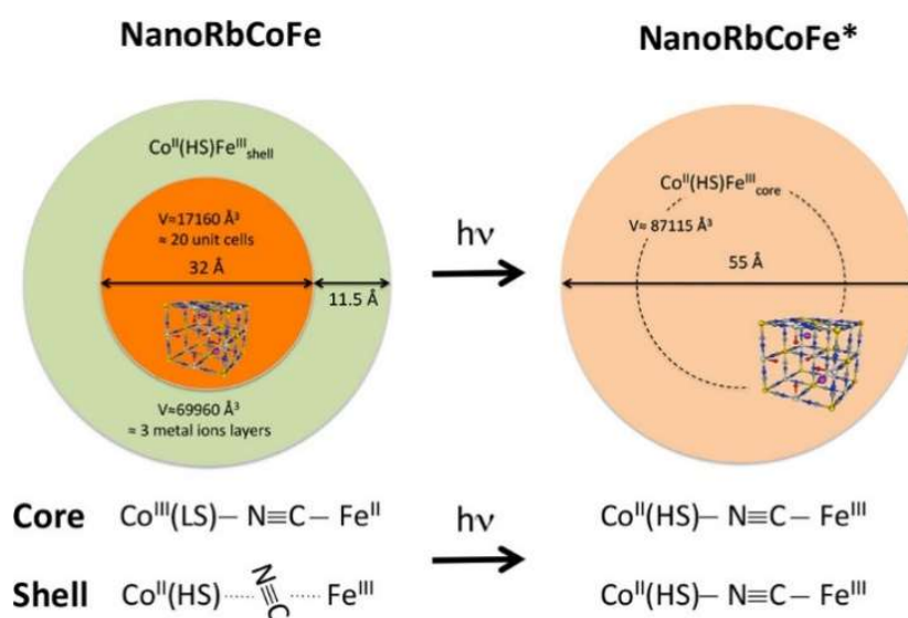
Figure 1-10. Structure of NanoRbCoFe before and after irradiation. Typical irradiation conditions are as follows: 10 K, \lambda = 635 nm, PW = 50 \text{ mW} \cdot \text{cm}^{-2} , 30 min. 83
