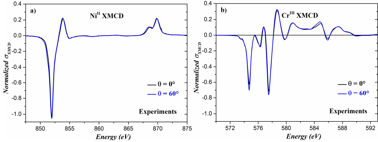
Figure 3-10. Angular dependence of XMCD for \theta = 0^\circ and \theta = 60^\circ : (a) at the \text{Ni } L_{2,3} edges, (b) at the \text{Cr } L_{2,3} edges. For both ions, the intensity of the isotropic spectra at the L_3 edge has been normalized to 1, T = 2 \text{ K} and B = 2 \text{ T}
