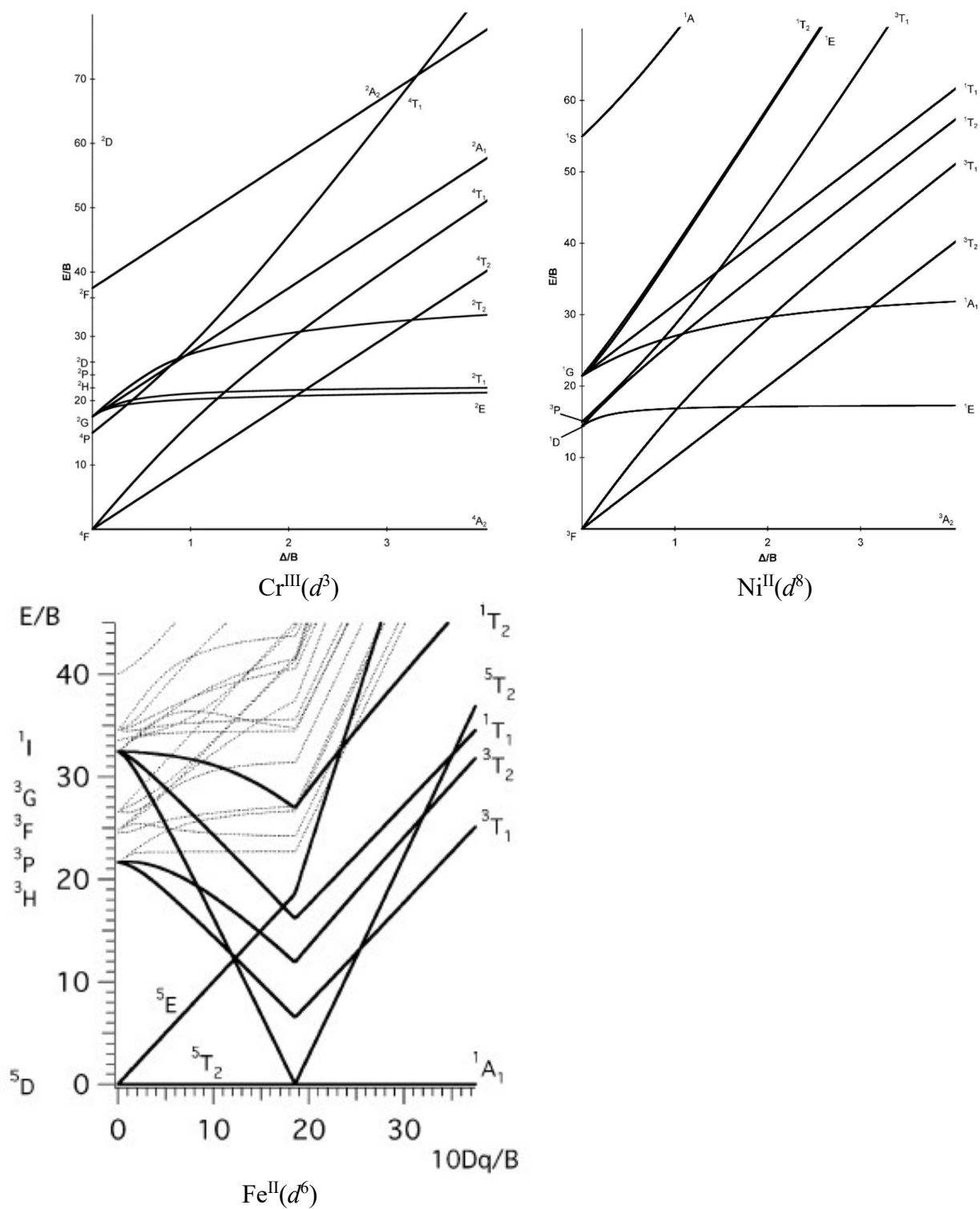
Figure I-1 Tanabe-Sugano diagrams for Cr, Ni and Fe ions. 2
