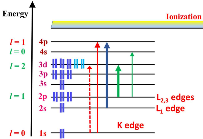
Figure 2-1. Nomenclature of the X-rays absorption transitions.
