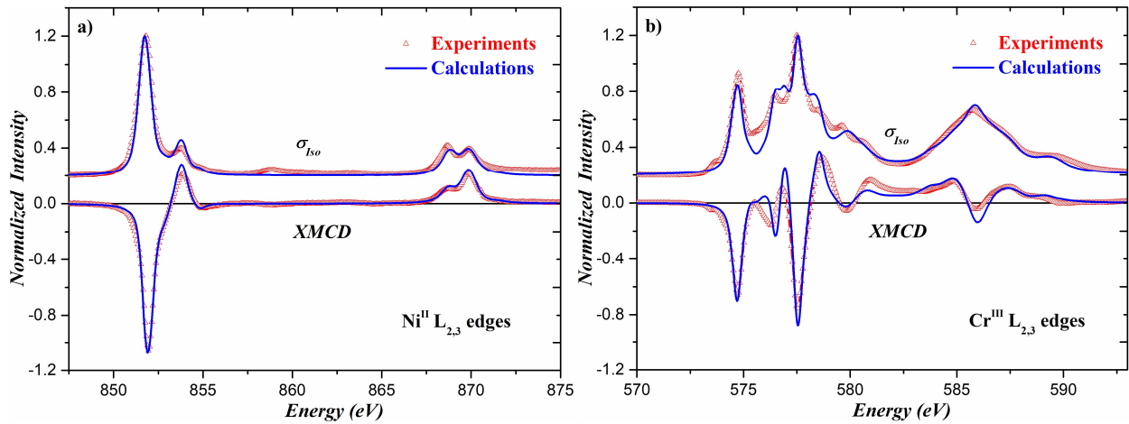
Figure 3-11. Comparison between theoretical and experimental isotropic cross-sections and XMCD signals for \theta = 60^\circ : (a) at the \text{Ni}^{\text{II}} L_{2,3} edges, (b) at the \text{Cr}^{\text{III}} L_{2,3} edges. The isotropic cross-sections have been artificially shifted upwards.
