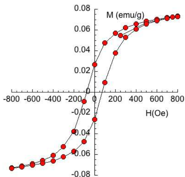
Figure II-2. SQUID measurements for \text{Cs}^{\text{I}}\text{Ni}^{\text{II}}\text{Cr}^{\text{III}}[\text{CN}]_6 NCs in powder at 2K
