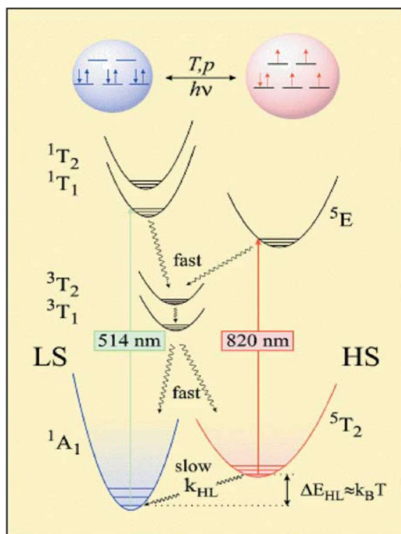
Figure 1-12. Schematic potential surfaces of low-lying ligand field states for a d^6 spin-crossover complex. The arrows indicate the mechanism for LIESST ( LS \rightarrow HS ) and reverse LIESST ( LS \leftarrow HS ). It is described when introducing green light ( \lambda=514.5\text{nm} ) induces the LS states converting into the metastable HS states; while as the introduction of red light ( \lambda=820\text{nm} ) the stable HS states are converted into metastable LS states. 102
