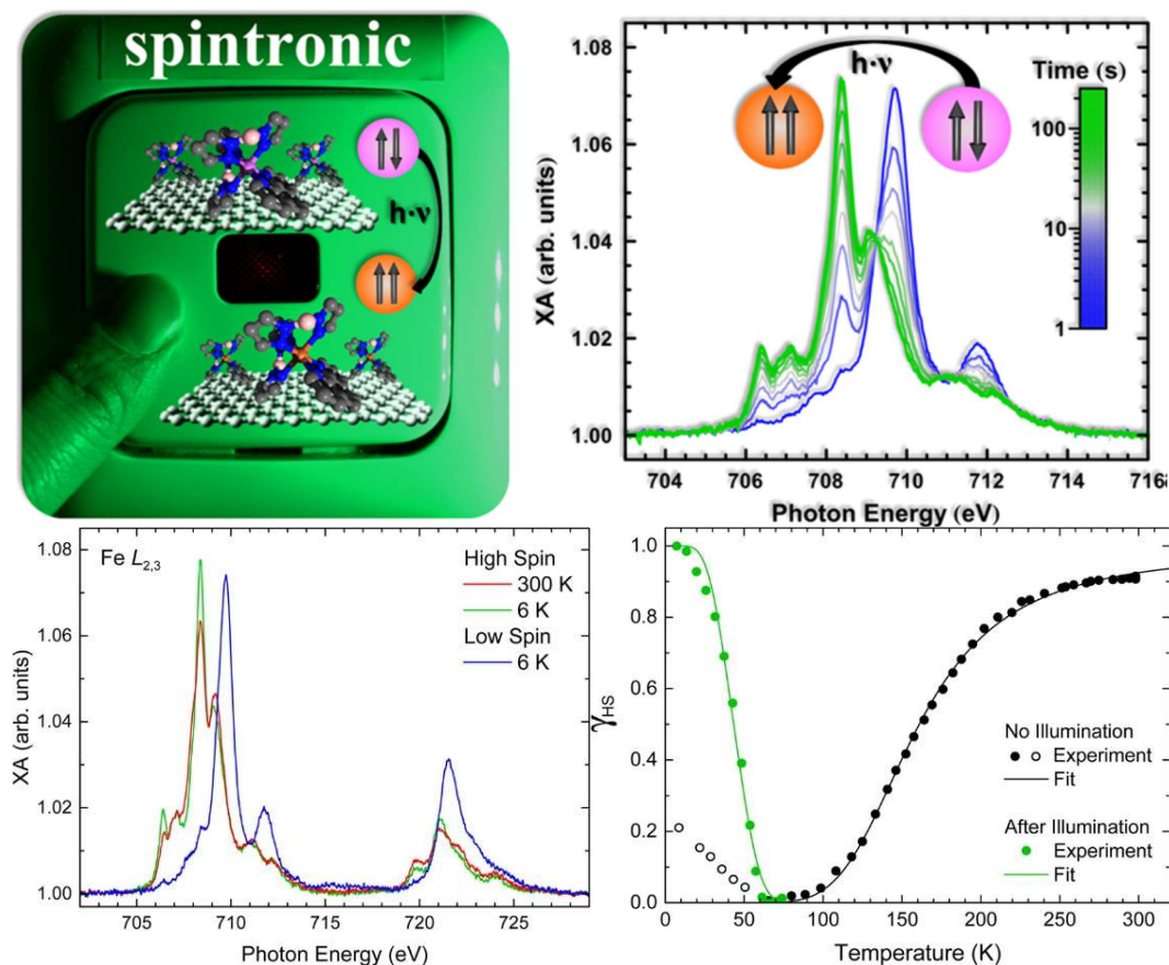
Figure 1-17. (a) Temperature-dependent Fe L_{2,3} X-ray absorption spectra of 0.4 ML of [\text{Fe}(\text{bpz})_2\text{phen}] on HOPG. Spectra before and after illuminating the sample with green light at T = 6 K are shown in blue and green, respectively and (b) Fraction of HS molecules as a function of temperature during cooling the sample without illuminations (black solid symbols) and after saturation of the light-induced HS state during heating the sample (green solid symbols), reproduced with permission from ref 117. 117
