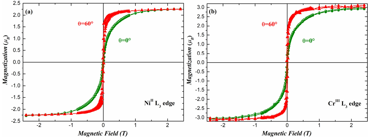
Figure 3-12. XMCD-detected Magnetization curves between 2 T and -2 T for \text{Ni}^{\text{II}} and \text{Cr}^{\text{III}} by setting the energy of the monochromator at the energy of the maximum (in absolute value) of the XMCD signal (i.e. 852.0 eV for \text{Ni}^{\text{II}} and 877.5 eV for \text{Cr}^{\text{III}} )
