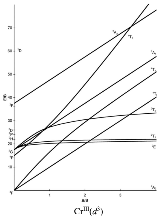
Figure I-1 Tanabe-Sugano diagrams for Cr, Ni and Fe ions. 2
