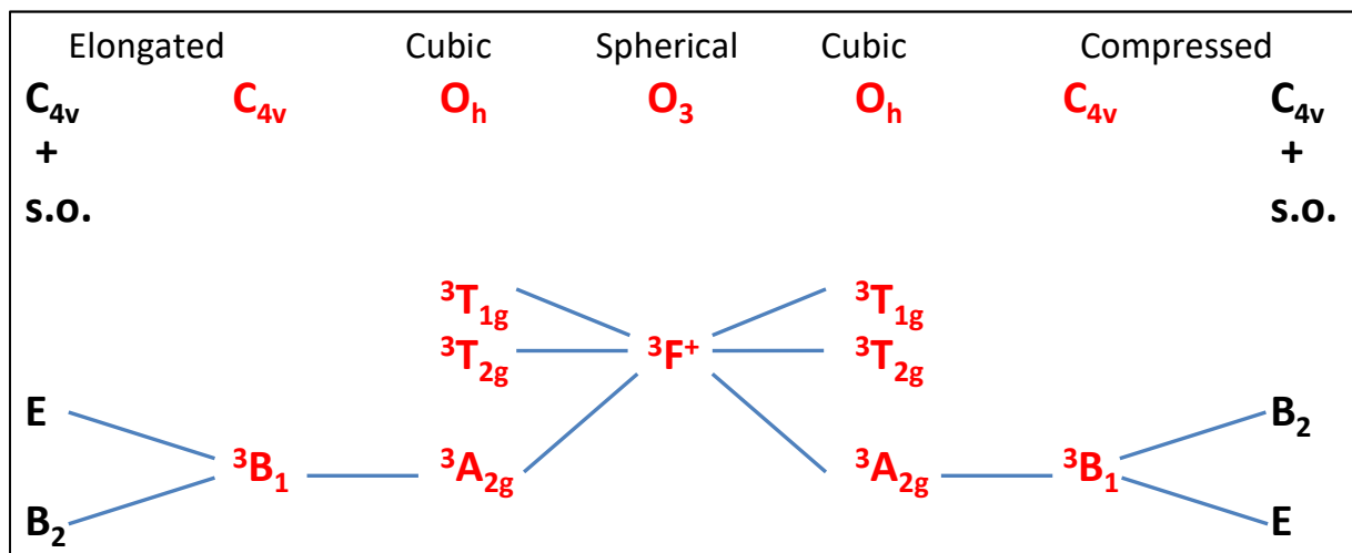
Figure 3-17. Energy diagrams of 3d multi-electronic levels for Ni II as a function of crystal field symmetry and spin-orbit coupling; when spin-orbit coupling is not considered, the irreducible representations are drawn in red and when spin-orbit coupling is turned on, they are reported in black.
