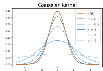
Figure 5.5: Illustration of the proposed approximation built with a Gaussian kernel \mathcal{N}(0, \rho^2) when the target distribution is Gaussian.
