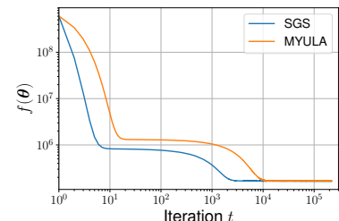
Figure 5.6: Convergence to the typical set of the posterior distribution \pi for SGS and MYULA.
