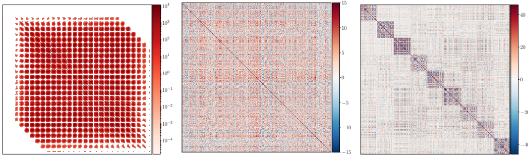
Figure 4.3: Examples of precision matrices \mathbf{X}^T \mathbf{X} for three datasets. Left: MNIST dataset (Le Cun et al., 1998). Only the predictors associated to the digits 5 and 3 have been taken into account for the MNIST dataset (Le Cun et al., 1998). Middle: leukemia dataset (Armstrong et al., 2002). For the leukemia dataset (Armstrong et al., 2002), only the first 5,000 predictors (out of 12,600) have been taken into account. Right: CoEPrA dataset (Ivanciuc, 2006).
