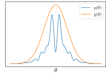
Figure 1: Illustration of the rejection sampling method. Here the instrumental distribution q is a Gaussian from which it is simple to generate samples.
