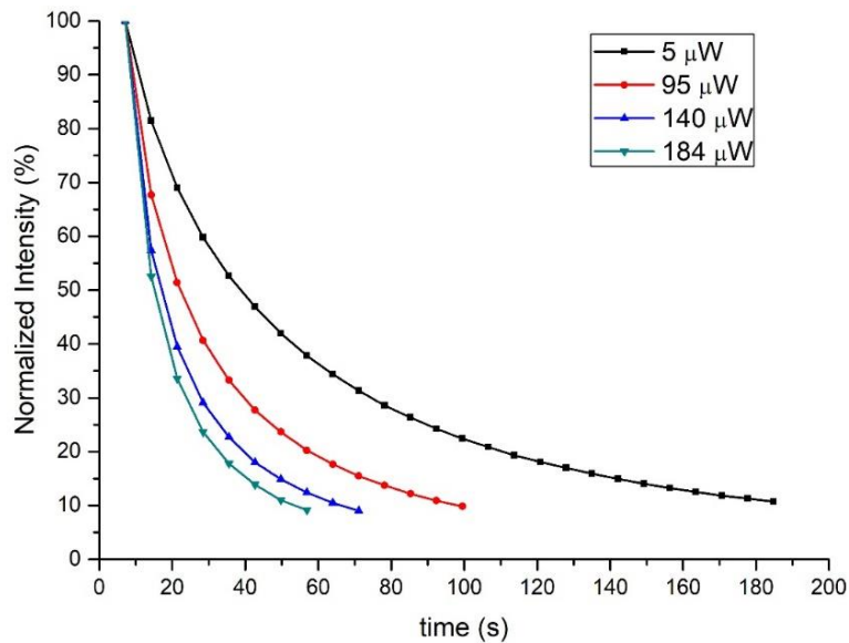
Figure 1.5: Fluorescence decay due to photobleaching. Rhodamine tagged to fibronectin protein emits fluorescence signals that decrease gradually with time. The faster the absorption rate because of the increase of the laser power, the shorter the fluorescence decay time will be.
