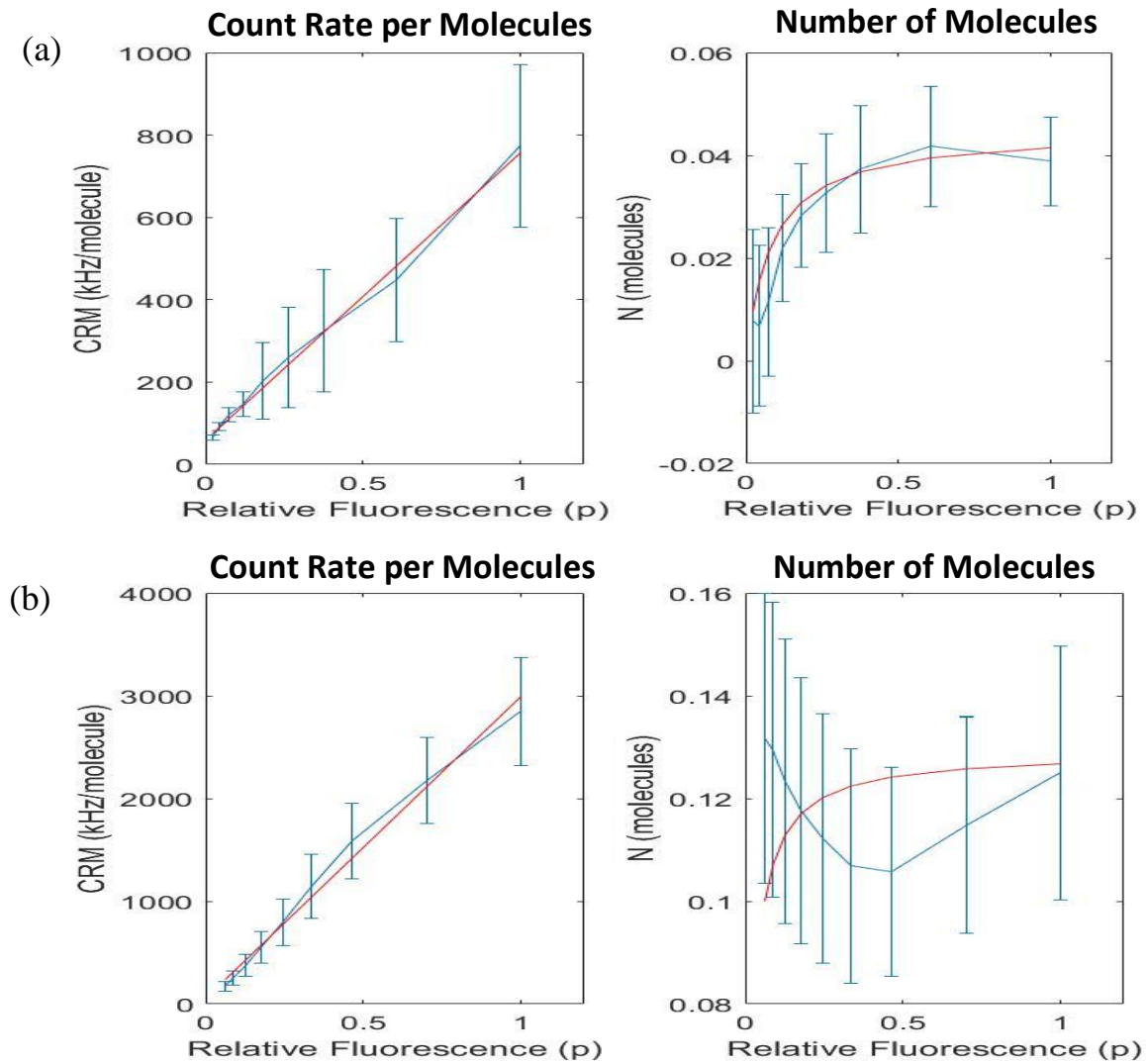
Figure 3.7: Count rate per molecule and number of molecules as a function of the relative fluorescence, p . Plotting for: (a) low concentration (calculated from 11 zones), and (b) high concentration (calculated from 9 zones). The number of beads and count rate per beads decrease as a function of the relative fluorescence. The error bars are obtained from the standard error of the mean of all zones for each relative fluorescence.
