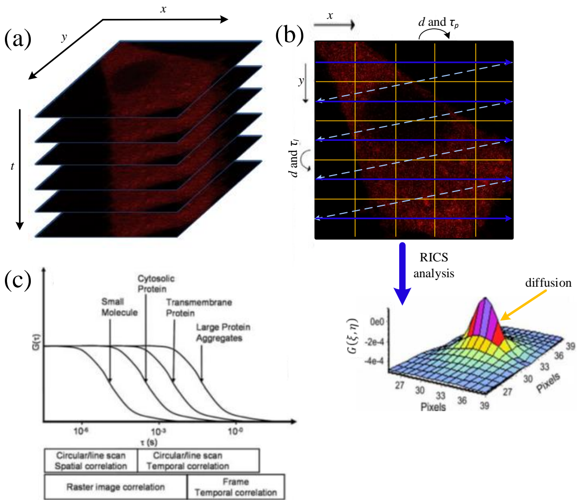
Figure 5.2: Raster Image Correlation Spectroscopy . (a) A series of image acquired with a confocal scanning microscope. Spatial autocorrelation is done in a single image and averaged through the series of images. (b) RICS analyze the spatial autocorrelation of fluorescence signal to determine the diffusion of molecules depends on parameters of acquisition: pixel size ( d ), pixel dwell time ( \tau_p ), and line time ( \tau_l ). (c) Diagram of the range of diffusion times accessible by different scanning techniques. RICS is suitable for small molecules, and cytoplasmic and transmembrane proteins. Adapted from [49].
