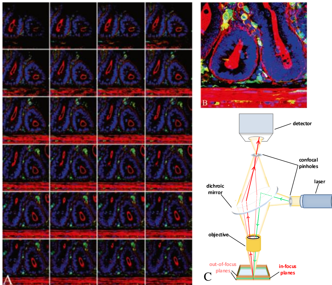
Figure 1.6: Confocal microscopy. (A) Optical sectioning with z-series through a section of intestine stained with multiple fluorescent dyes; blue: DAPI stain for nuclei, red: f-actin stain, green: GFP, yellow: mRNA stabilizing protein. (B) Image reconstruction of all sections in (A). (C) Scheme of laser scanning confocal microscope. Exciting laser light is reflected by a dichroic mirror and focused on the specimen in a focal plane. As the laser scans, fluorescence emitted from the focal plane passes through the mirror, and only light that passes through the pinhole aperture is detected and forms the image. Adapted from [31].
